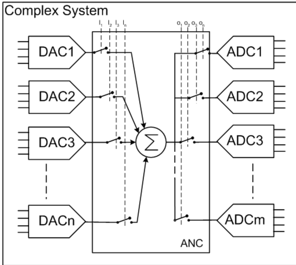
Figure 2-25: Analogue Network of Converters in a complex system
