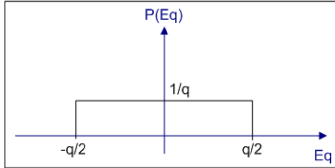
Figure 2-6: Probability density of quantization error
