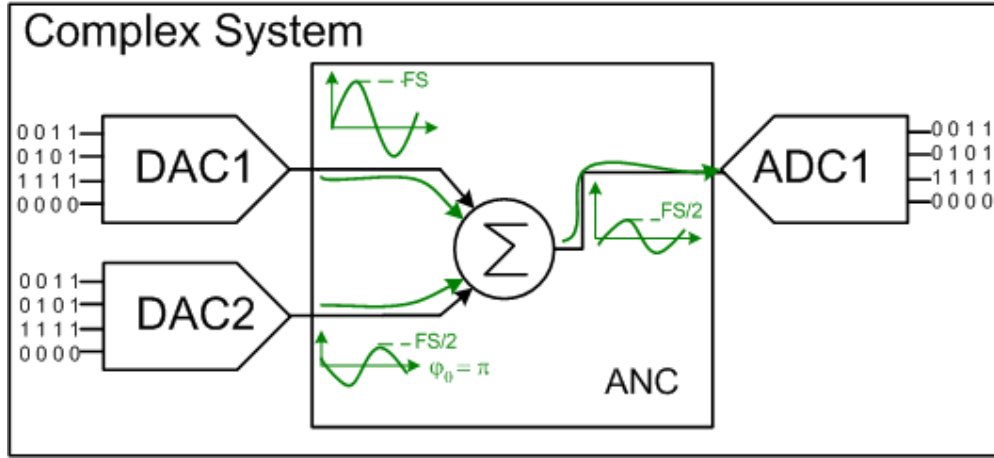
Figure 2-30: Fourth test setup
