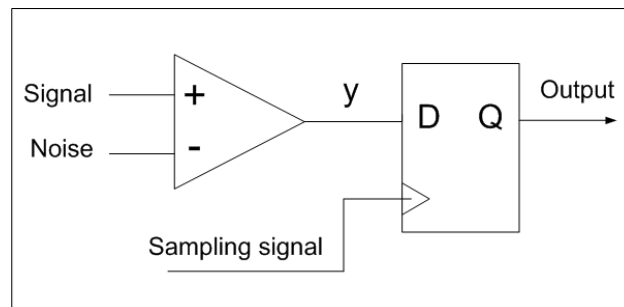
Figure 1-30: 1-bit embedded digitizer
