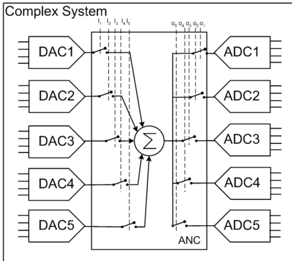
Figure 2-32: ANC made of 5 DACs and 5 ADCs
