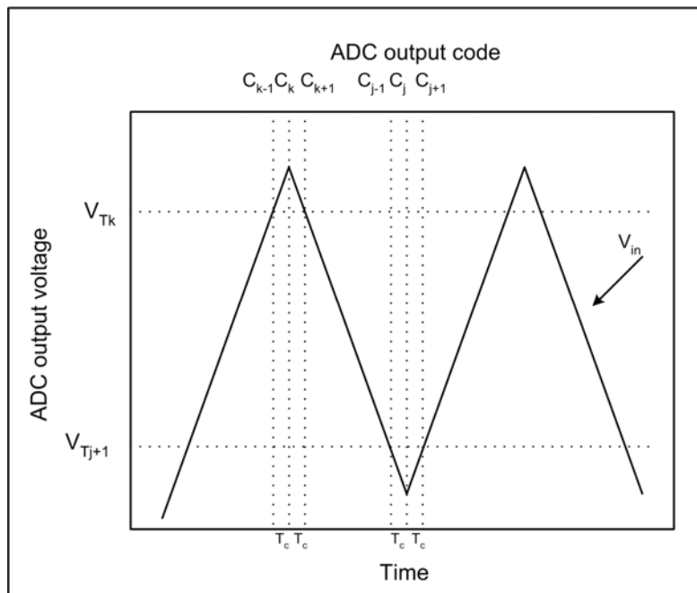
Figure 2-16: ADC input voltage oscillation between V_{Tk} and V_{Tj+1} transition thresholds
