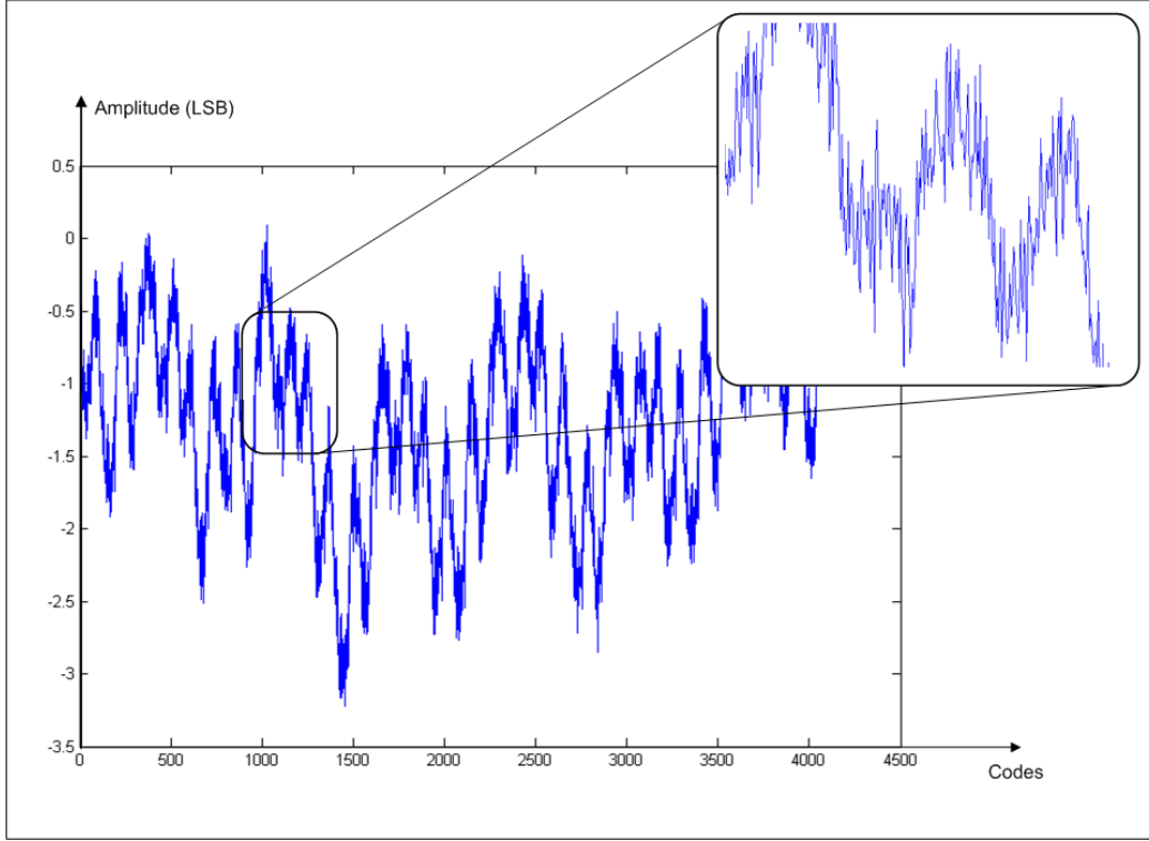
Figure 2-23: INL curve of a real-life 12-bit ADC
