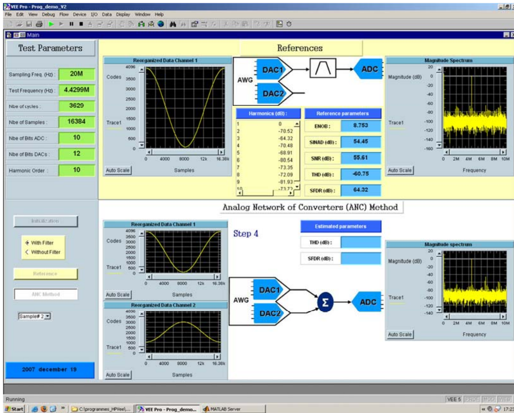
Figure 3-16: HP-Vee interface to control the instruments and the implementation of the method
