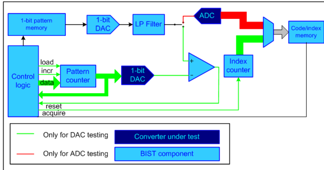
Figure 2-14: BIST architecture for DAC and ADC [chen99]
