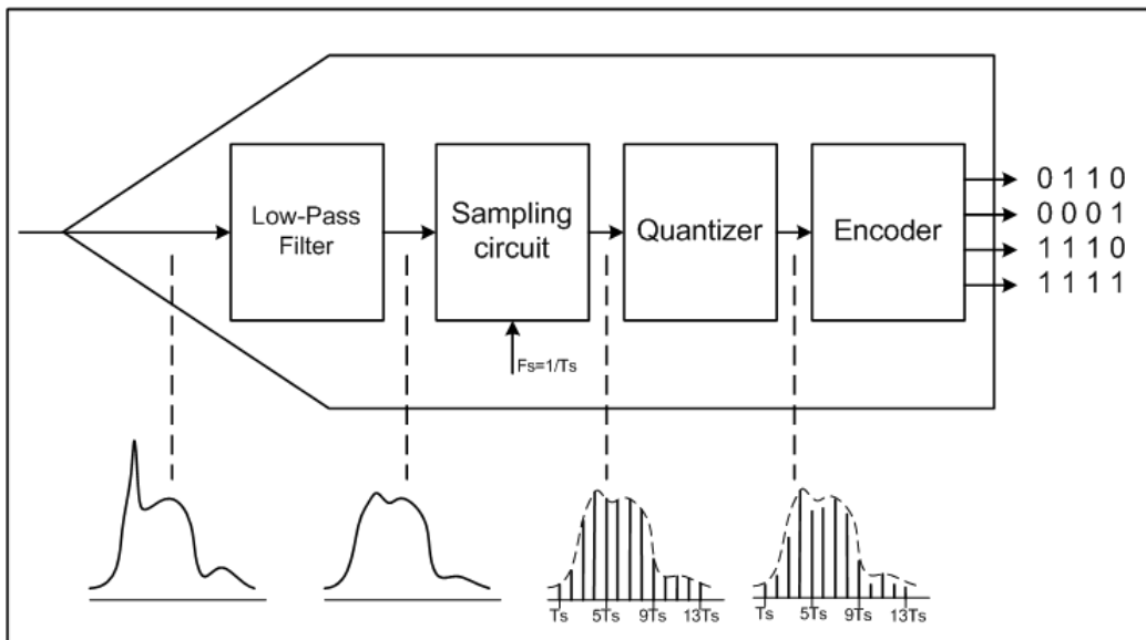
Figure 2-1: Analogue-to-digital conversion
