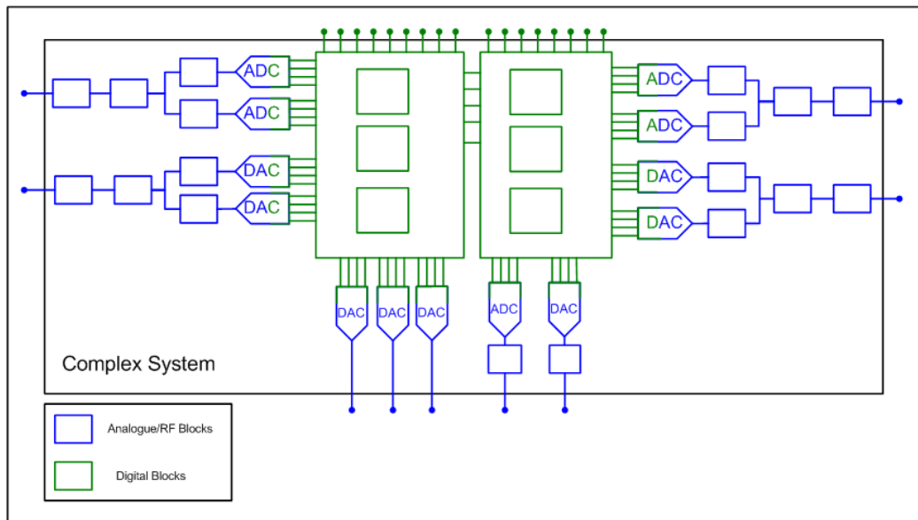
Figure 1-10: Block diagram of a potential system.
