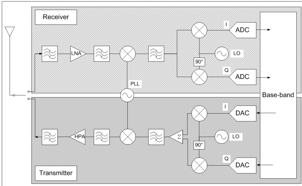
Figure 1-6: Superheterodyne architecture
