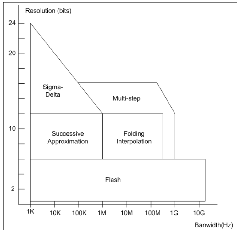
Figure 2-4: Performances of ADC architectures
