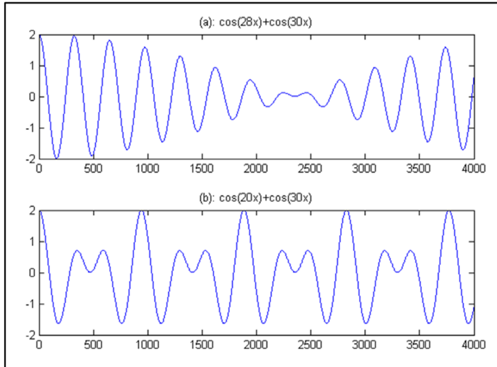
Figure 1-15: Two examples of two-tone sine waves
