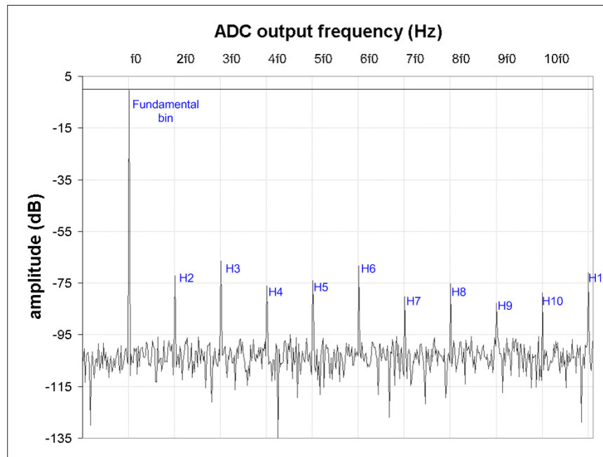
Figure 3-7: Spectrum of a signal captured at the output of a C(2,1) configuration
