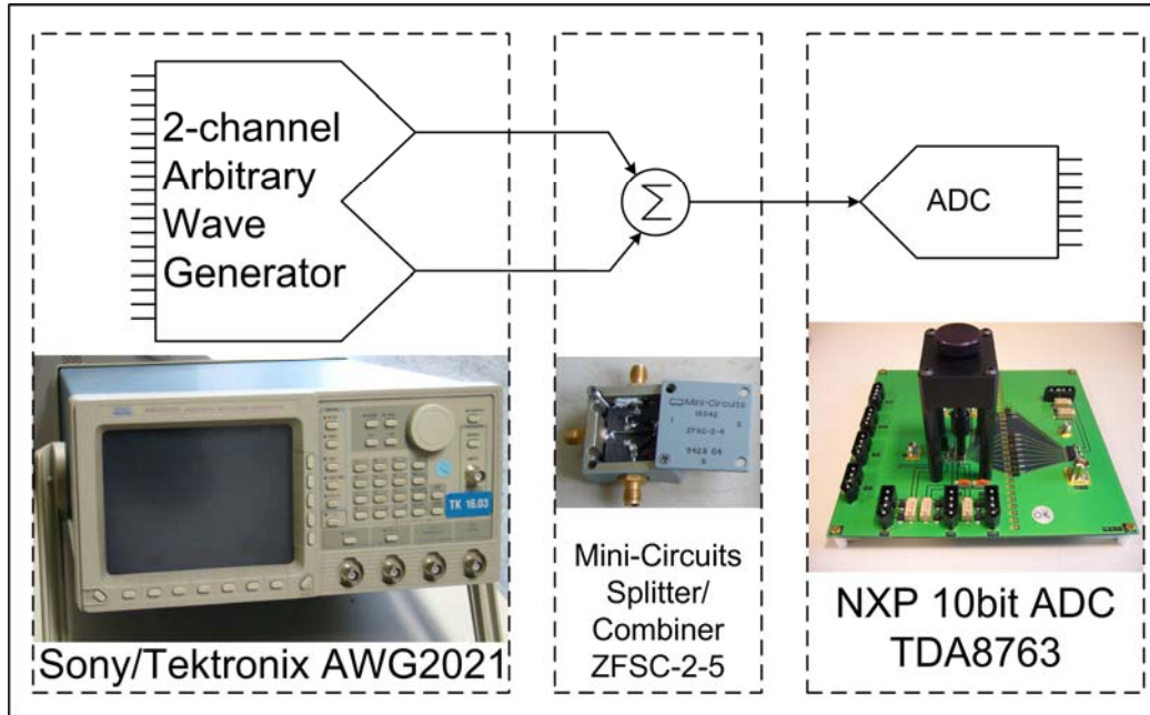
Figure 4-5: Hardware set-up
