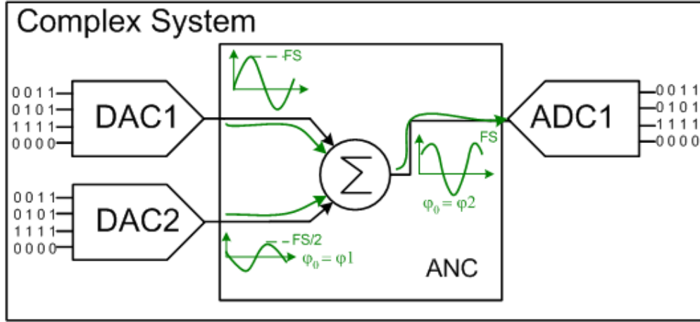
Figure 2-31: Fifth test setup
