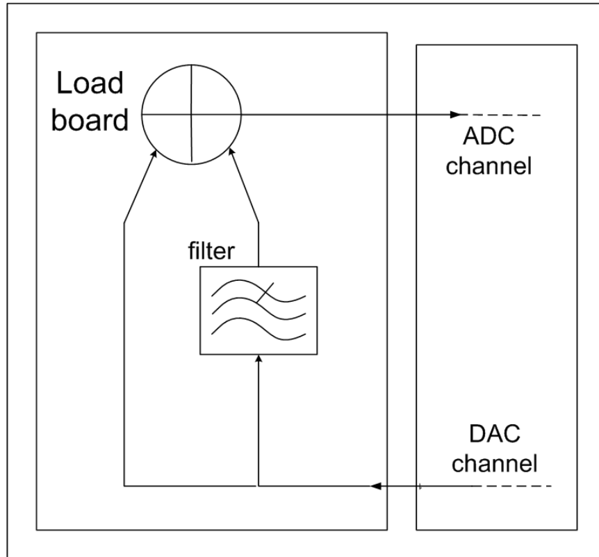
Figure 2-18: Loopback implementation from Abraham et al solution [shin06]
