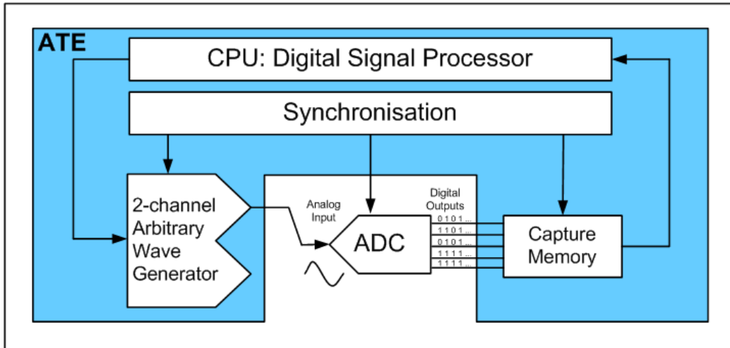
Figure 4-4: Conventional test set-up using a low-resolution AWG for the new approach of industrial ADC test
