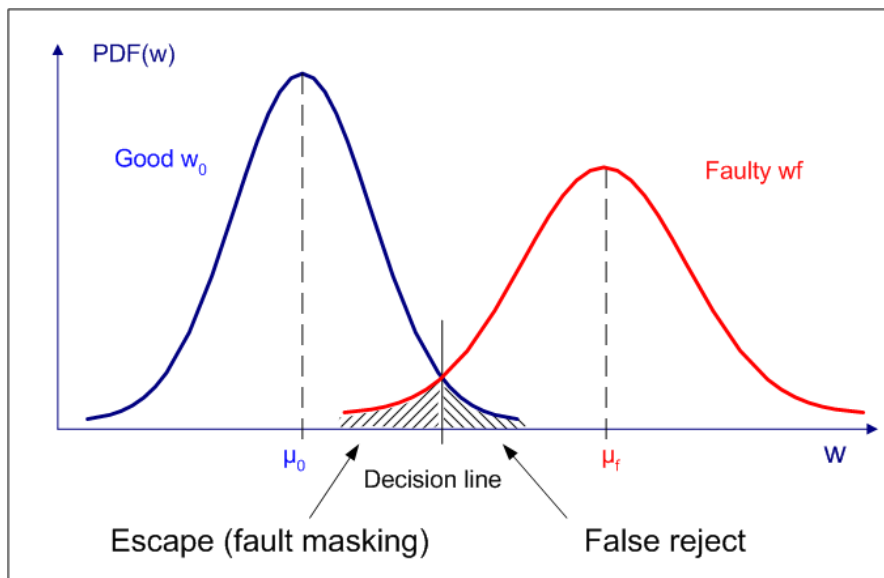
Figure 1-28: Test response PDF [dabr04]
