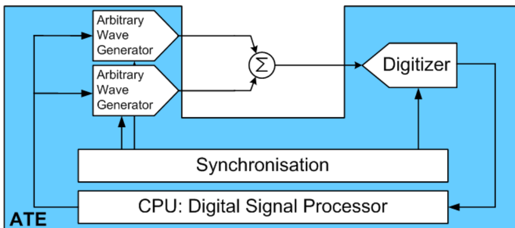
Figure 4-8: Set-up for the calibration of analogue instruments from ATE
