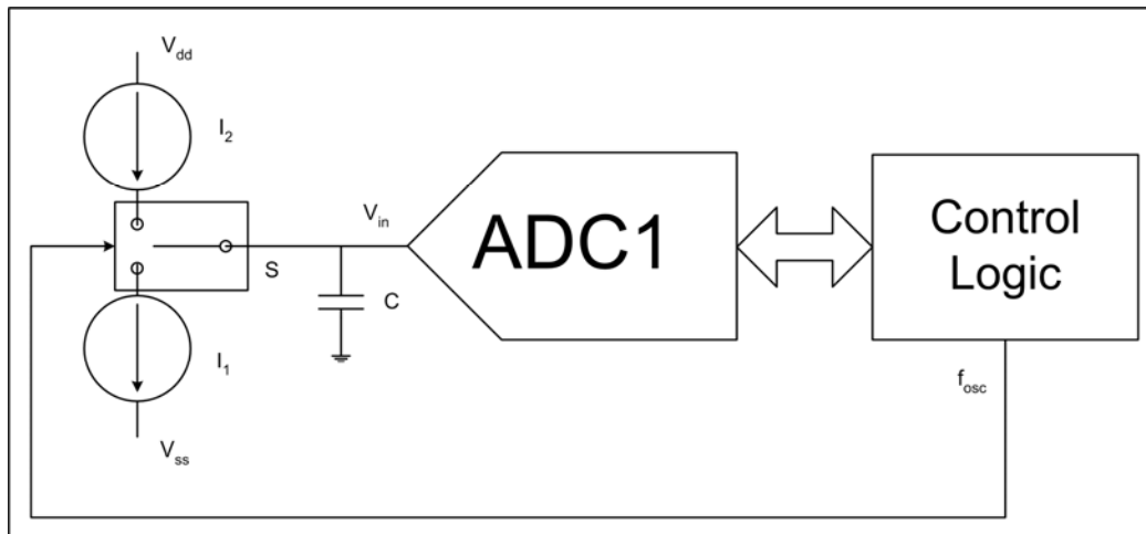
Figure 2-15: Oscillation-based BIST architecture proposed in [arab97]
