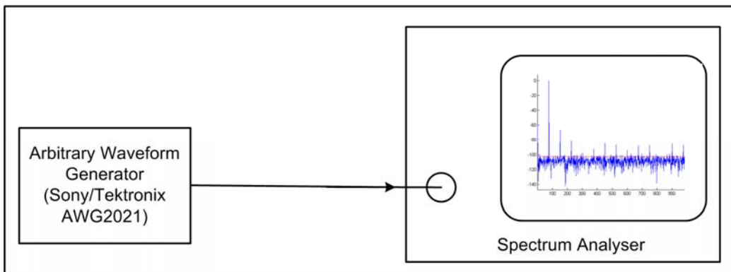
Figure 3-13: Splitter influence on harmonics, first set-up
