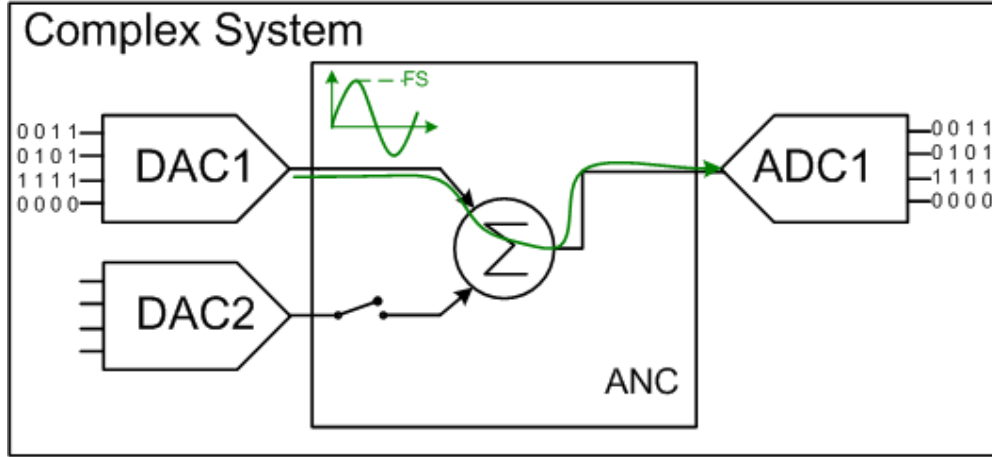
Figure 2-27: C(1,1) test configuration
