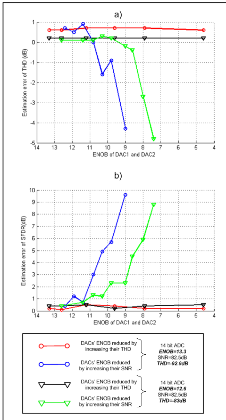
Figure 3-5: a) THD estimation error vs. ENOB of DACs b) SFDR estimation error vs. ENOB of DACs
