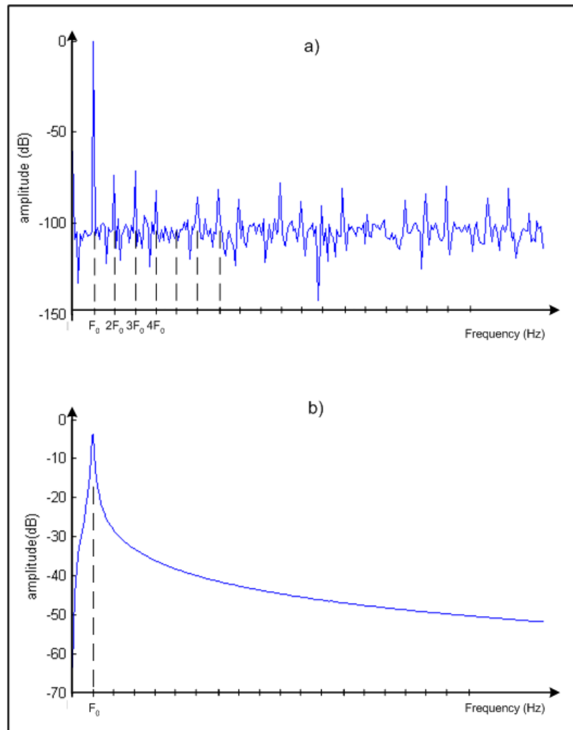
Figure 2-11: Spectrum a of sine wave a) coherently sampled b) non-coherently sampled
