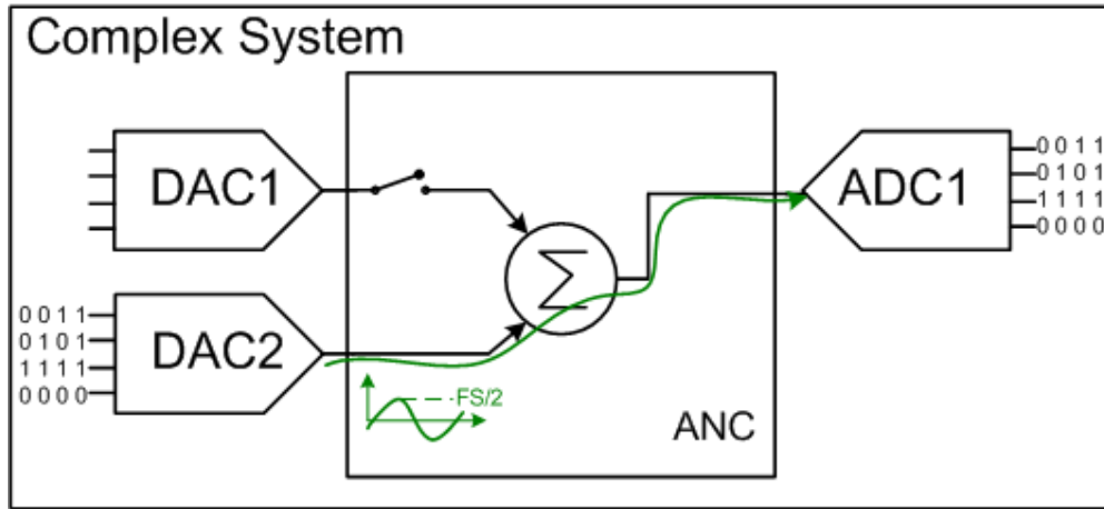
Figure 2-29: New third test setup
