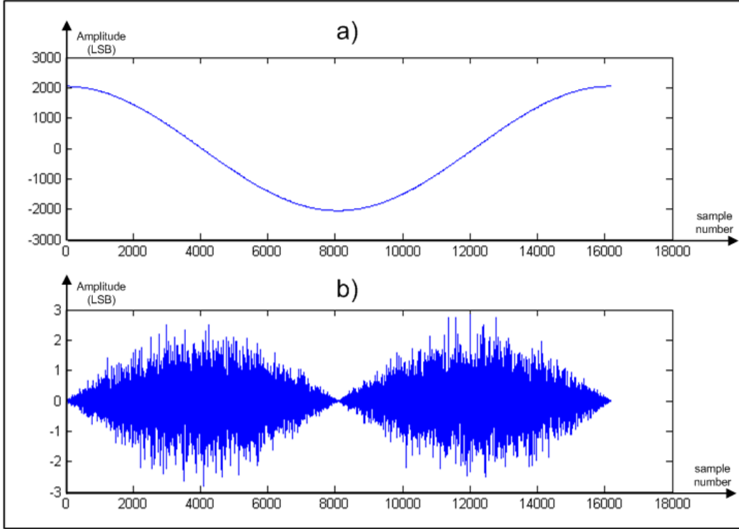
Figure 3-1: a) 1kHz sine wave sampled at f_s=163.84\text{MHz} and deteriorated by a sampling jitter with standard deviation of 5ps b) difference between the deteriorated sine wave from a) and a pure sine wave
