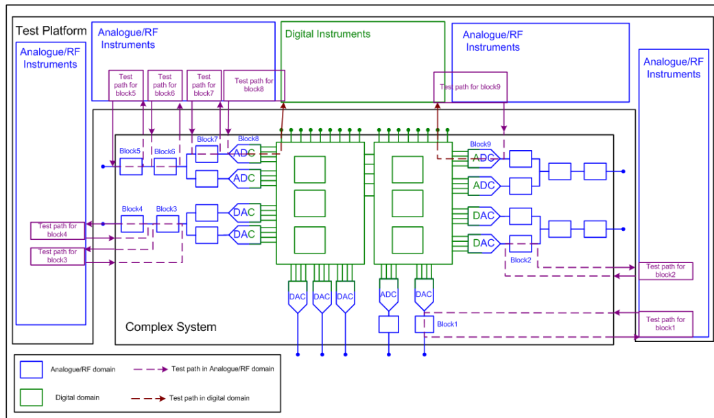
Figure 1-12: Test of analogue cores of a potential system
