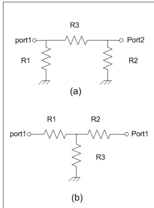
Figure 1-23: Implementation of a resistor-based attenuator [yoon05] a) \Pi -attenuator b) T-attenuator
