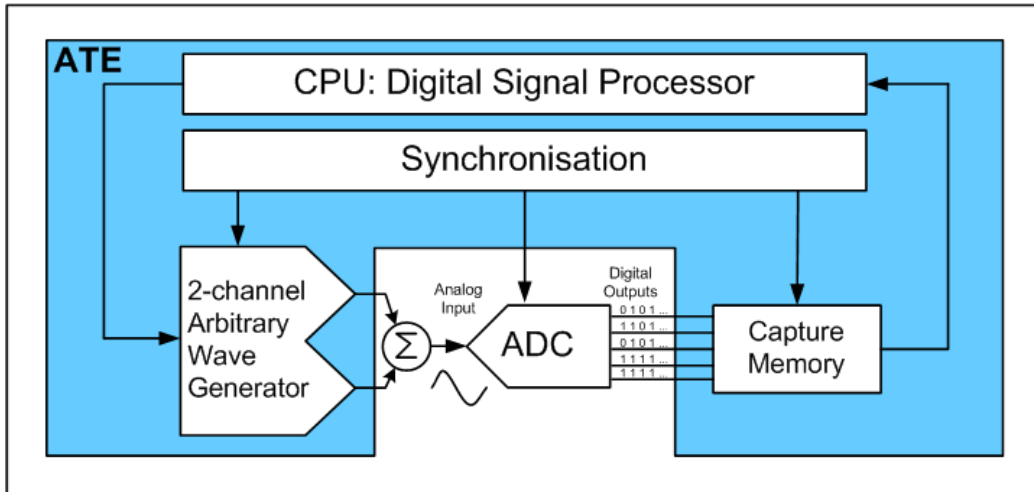
Figure 4-3: Required set-up to estimate the harmonic contributions of the AWG
