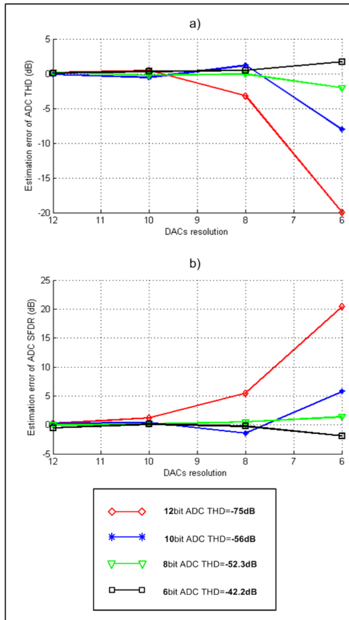
Figure 3-11: a) estimation error of ADC's THD Vs DACs resolution b) estimation error of ADC's SFDR Vs DACs resolution
