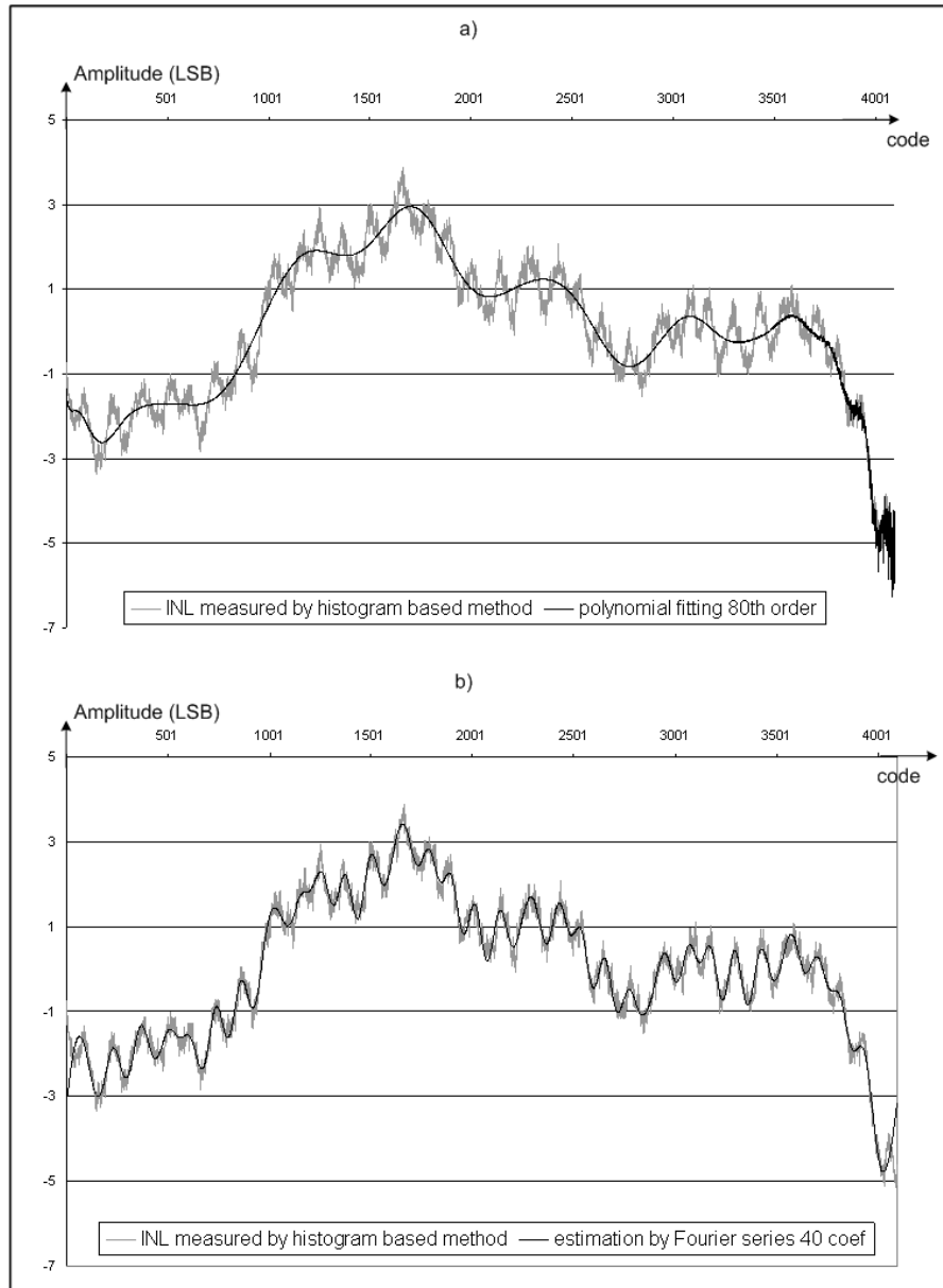
Figure 3-2: INL curve model a) comparison between an INL curve and its 80 th order polynomial fitting b) comparison between an INL curve and its Fourier series expansion, the series development is made with 40 odd and 40 even Fourier coefficients
