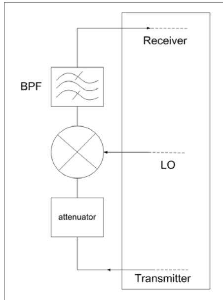
Figure 1-26: Loopback circuitry, as proposed by [srin06]
