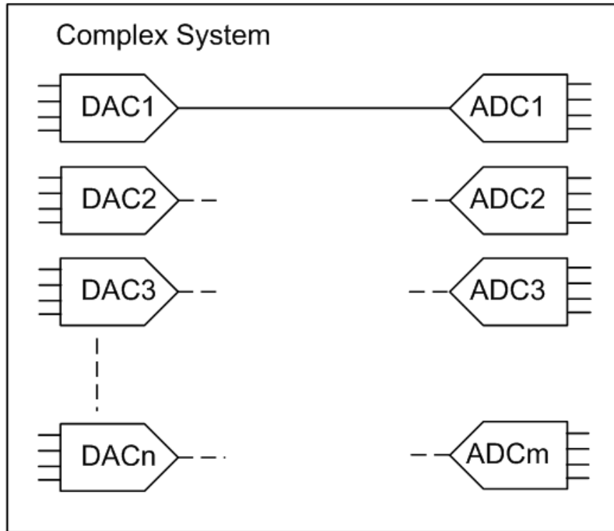
Figure 2-22: A fully digital test implemented by connecting a DAC and an ADC in the analogue domain
