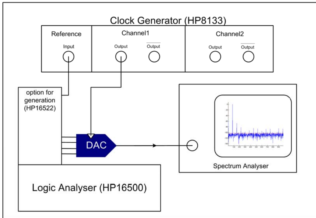
Figure 3-19: Conventional set-up for DAC test
