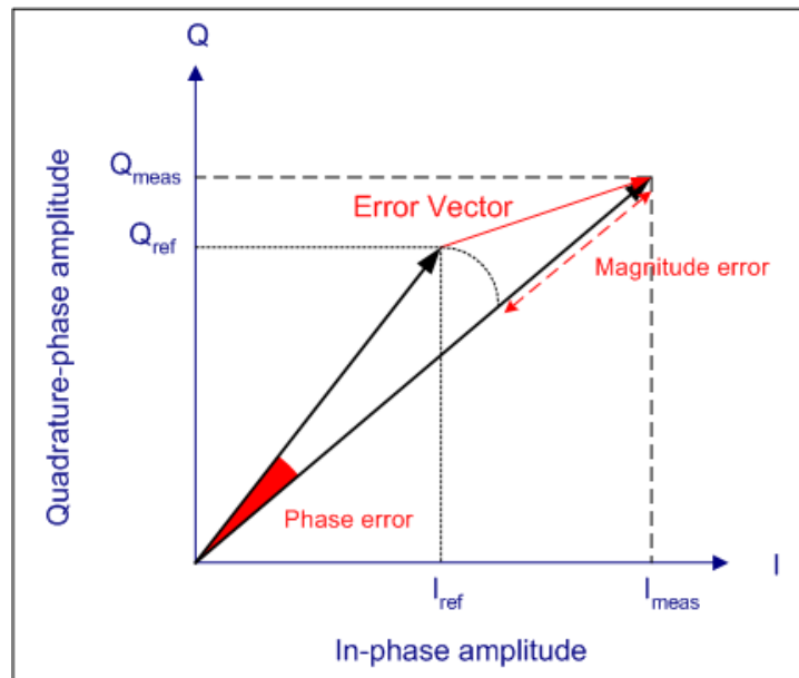
Figure 1-16: Error vector between reference vector and measured vector
