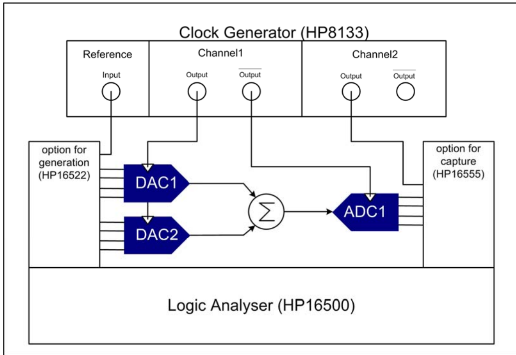
Figure 3-15: Set-up for the ANC-based test
