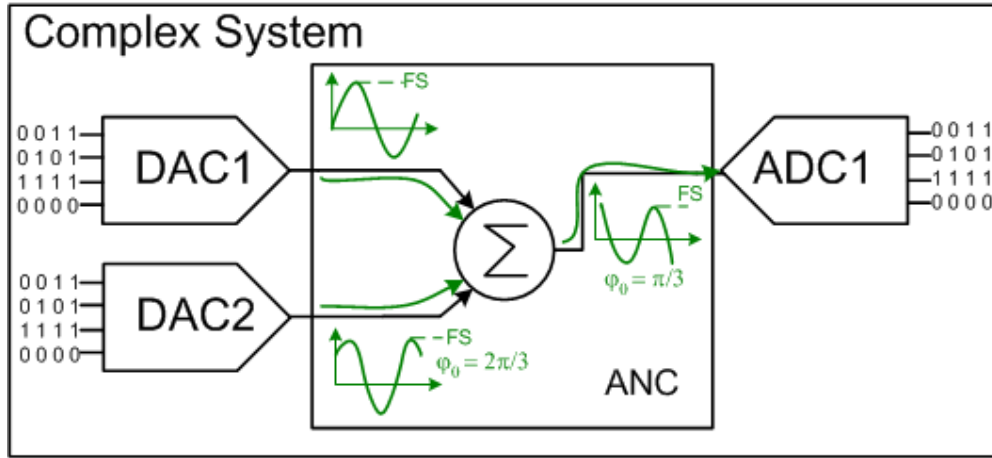
Figure 2-28: Third test setup
