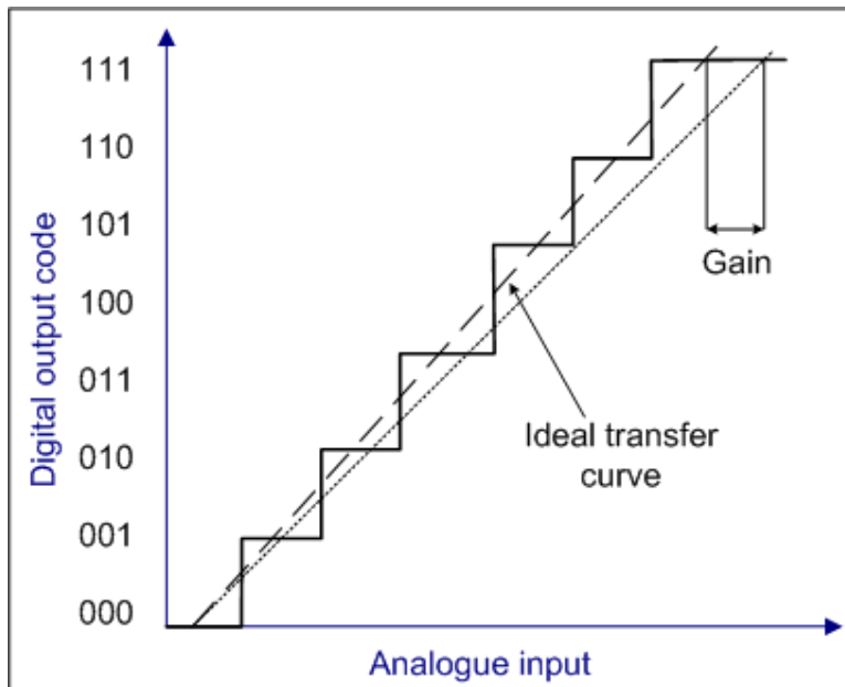
Figure 2-8: Gain error on an ADC transfer function
