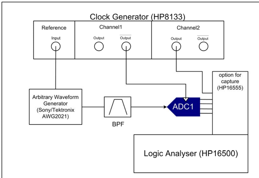
Figure 3-18: Conventional set-up for ADC test
