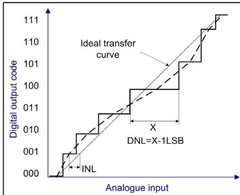
Figure 2-9: Non-linearity error on an ADC transfer function
