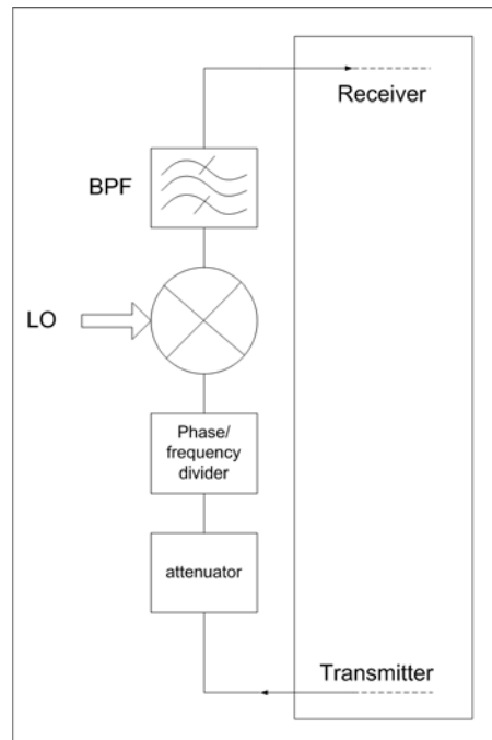
Figure 1-27: Loopback circuitry, as proposed by [hald05]
