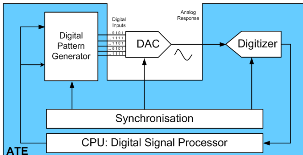
Figure 4-7: Mass production test set-up
