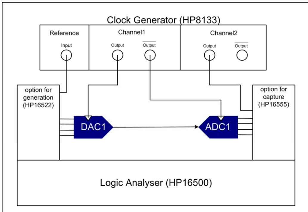
Figure 3-17: Second experimental set-up for ANC-based method validation
