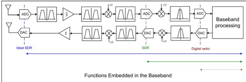
Figure 1-7: SDR architecture
