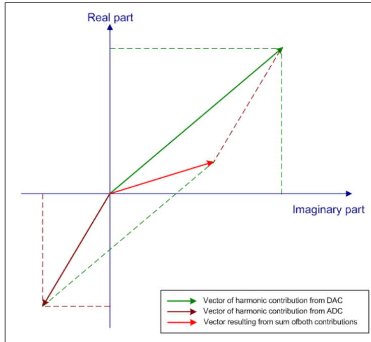
Figure 2-24: Sum of two harmonic contributions
