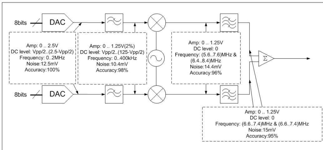
Figure 1-14: Mixed-signal up-conversion path
