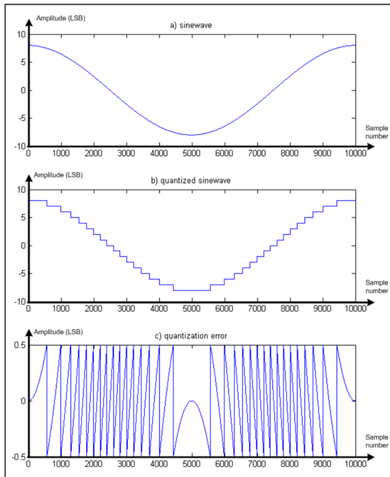
Figure 2-5: Deterministic “quantization noise”: a) continuous sine wave, b) sine wave quantized for conversion, c) quantization error (difference between continuous and quantized sine waves)
