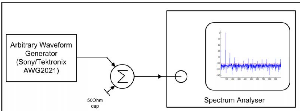
Figure 3-14: Splitter influence on harmonics, second set-up
