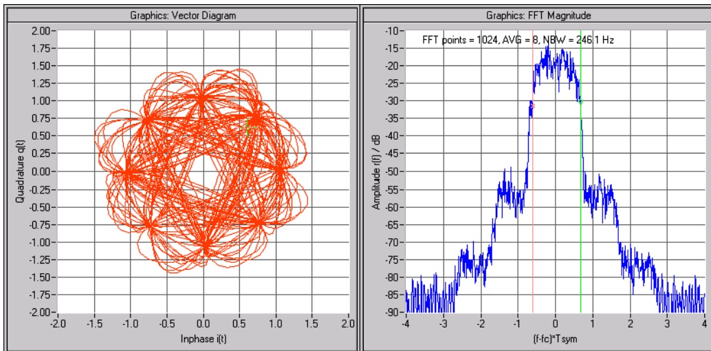
Figure 1-18: Constellation and spectrum of a Q/4DQPSK modulated sine wave at 21kHz, with distortion
