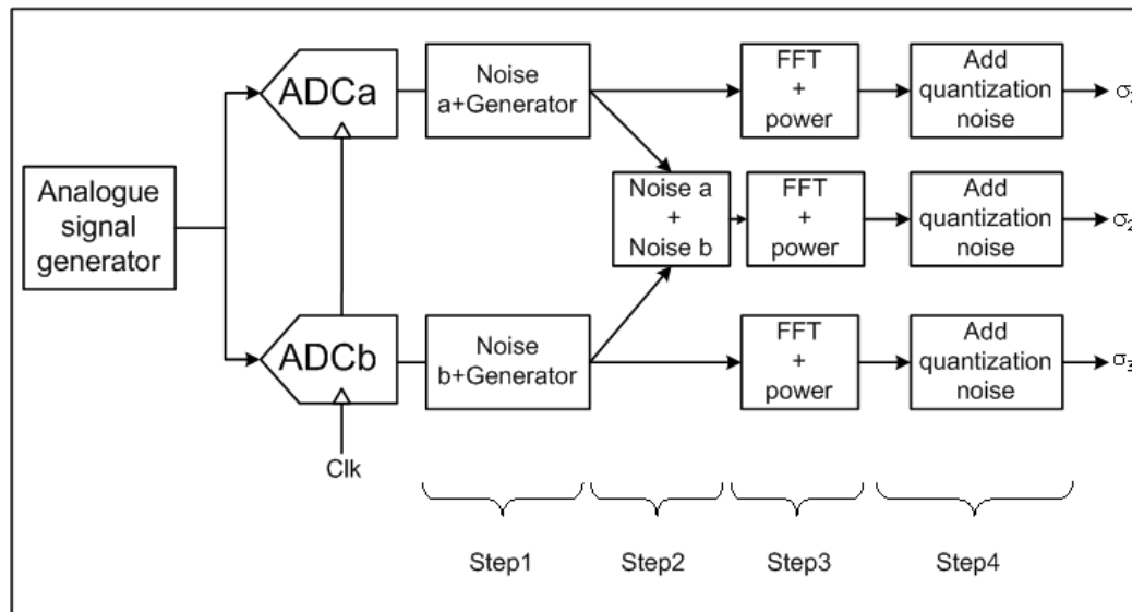
Figure 2-21: 2-ADC method for noise discrimination
