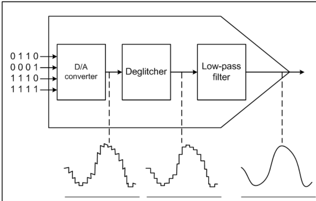
Figure 2-2: Digital-to-analogue conversion
