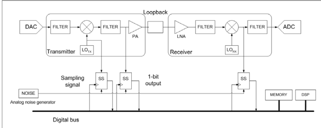
Figure 1-31: Improved loopback structure
