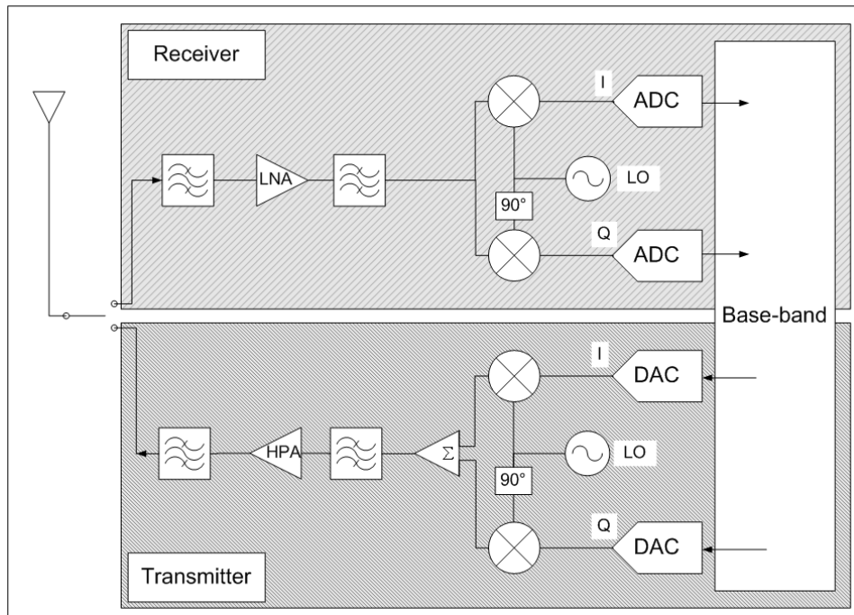
Figure 1-5: Zero-IF architecture
