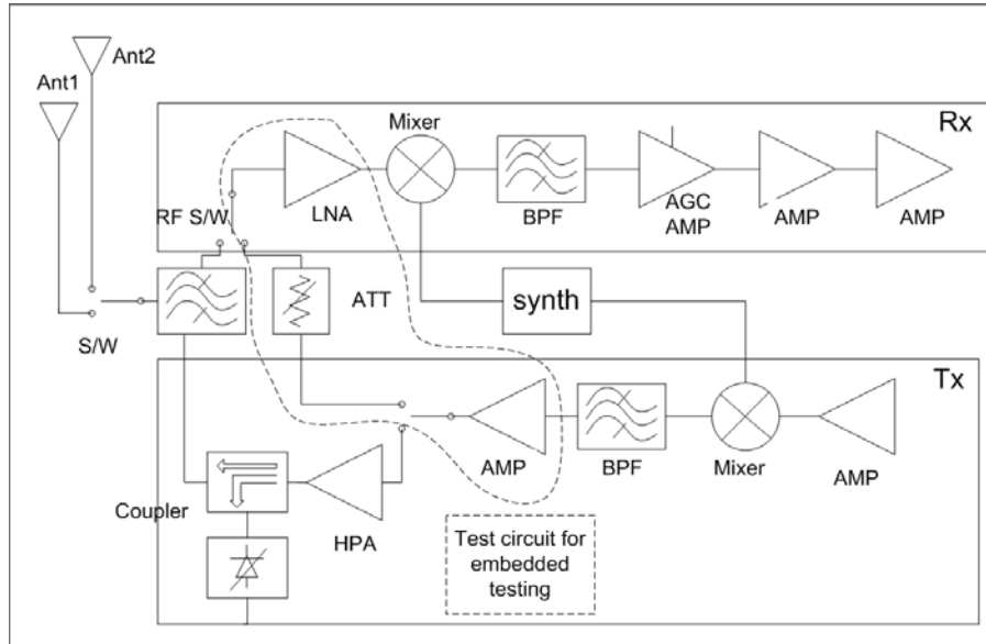
Figure 1-22: Core diagram of a loopback implementation for WLAN transceiver [yoon05]
