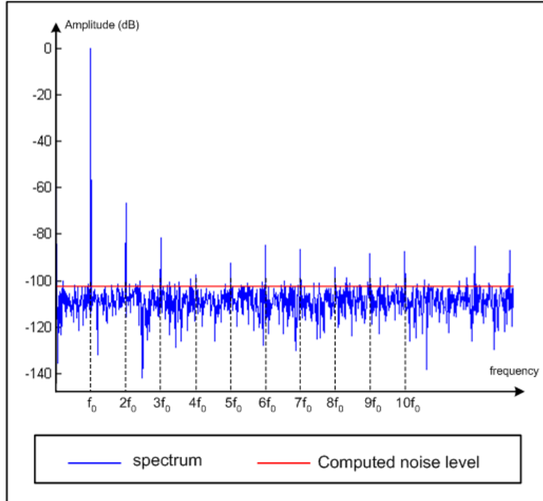
Figure 3-9: Computed noise level for a given spectrum
