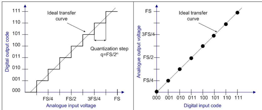
Figure 2-3: Transfer functions of a 3-bit ADC (left) and of a 3-bit DAC (right)
