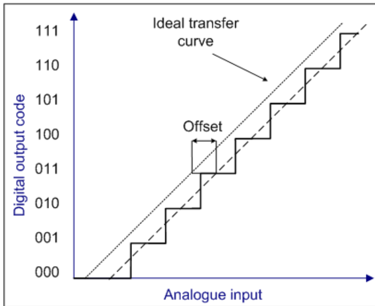
Figure 2-7: Offset error on an ADC transfer function
