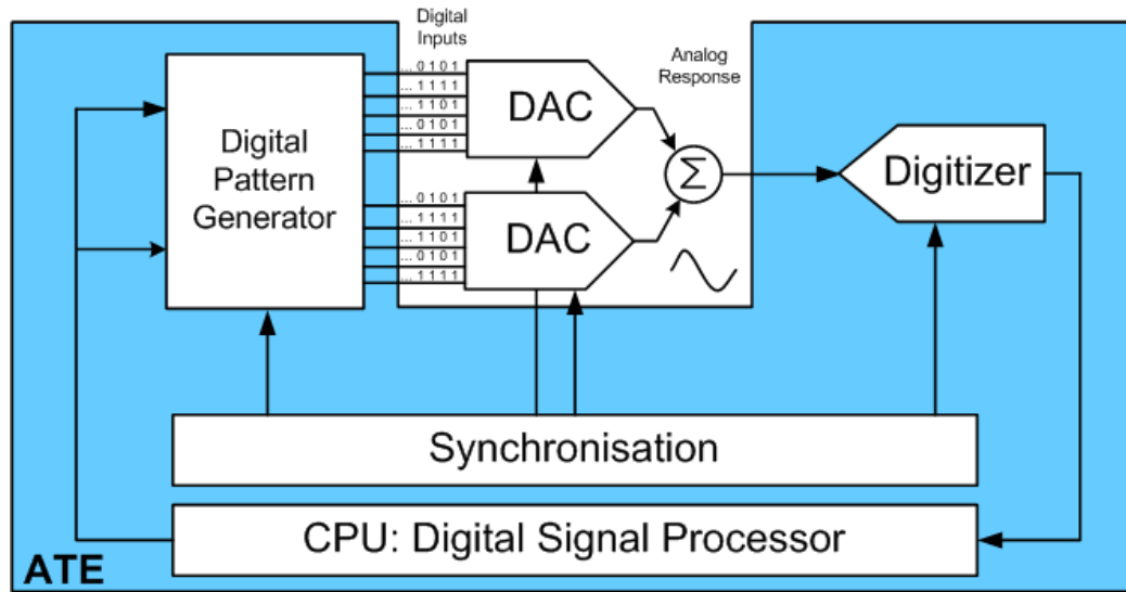
Figure 4-6: Learning step set-up
