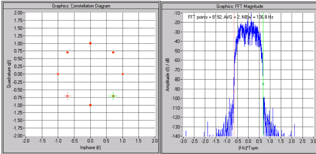
Figure 1-17: Constellation and spectrum of a Q/4DQPSK modulated sine wave at 21kHz, no distortion
