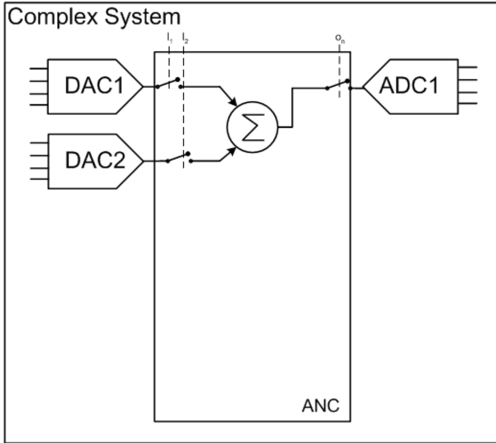
Figure 2-26: Two DACs and one ADC interconnection using ANC
