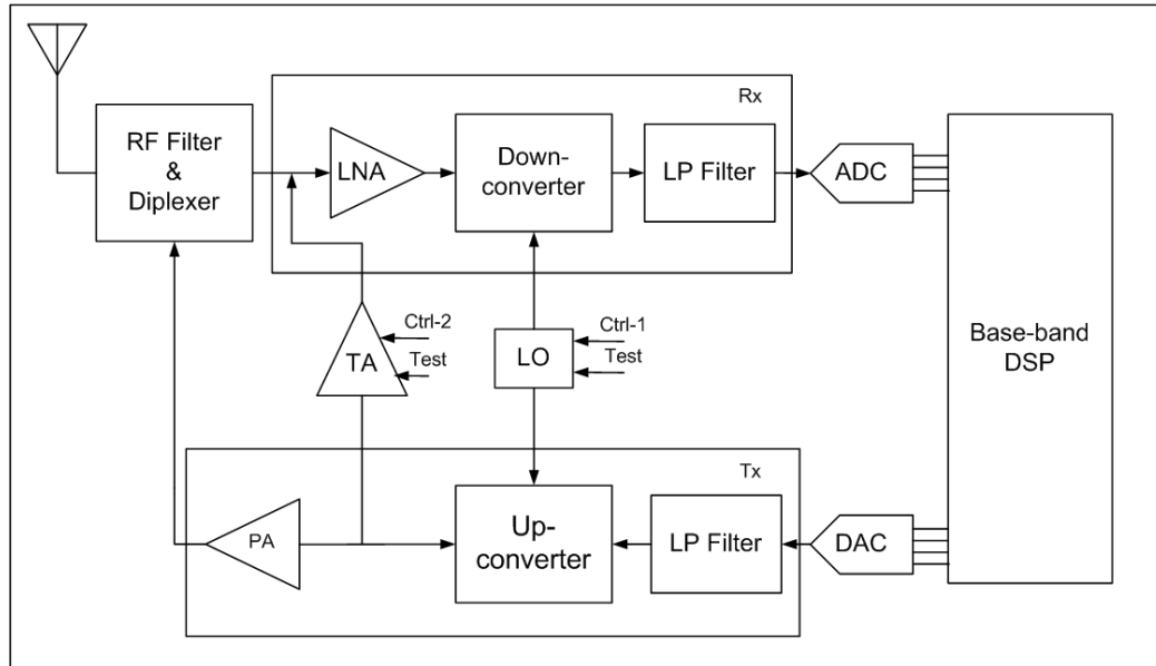
Figure 1-24: Loopback principle with different frequencies for Tx and Rx [dabr03]
