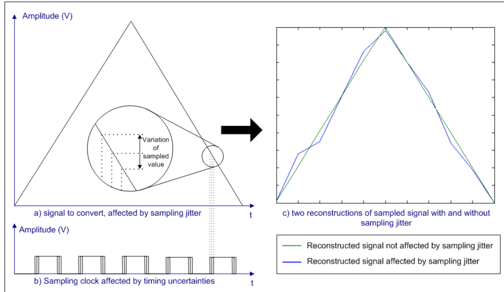
Figure 2-10: Effect of sampling jitter a) signal to convert b) sampling clock affected by some jitter c) signal reconstructed after sampling with and without jitter
