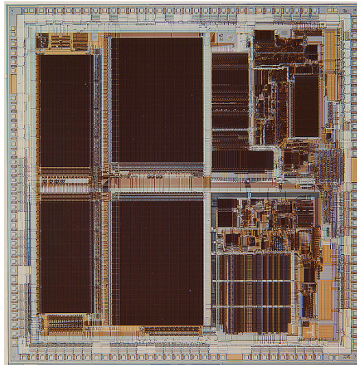
Figure 1-8: Example of SoC embedding, CFPA chip developed by CVAX.
