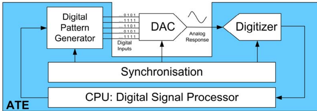
Figure 2-13: DSP-based test set-up of a DAC
