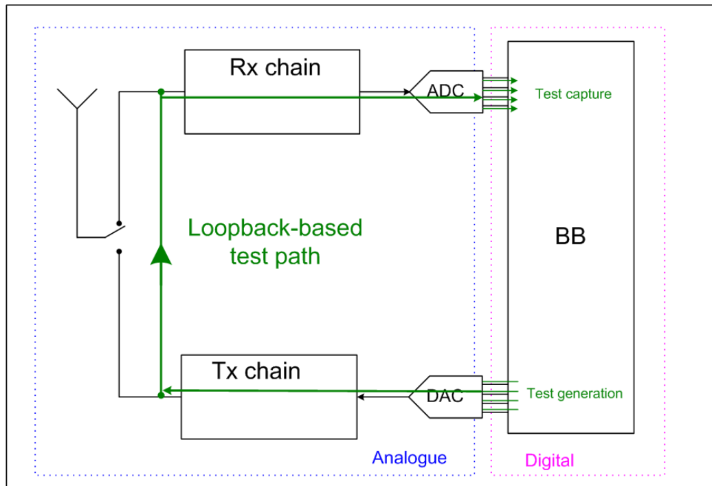
Figure 1-21: Basic principle of loopback-based test implementation
