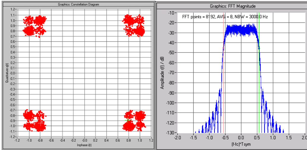
Figure 1-19: Constellation and spectrum of a QPSK modulated sine wave at 4.096MHz, no distortion
