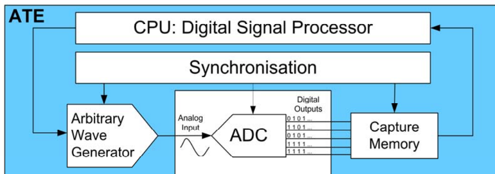
Figure 2-12: DSP-based test set-up of an ADC
