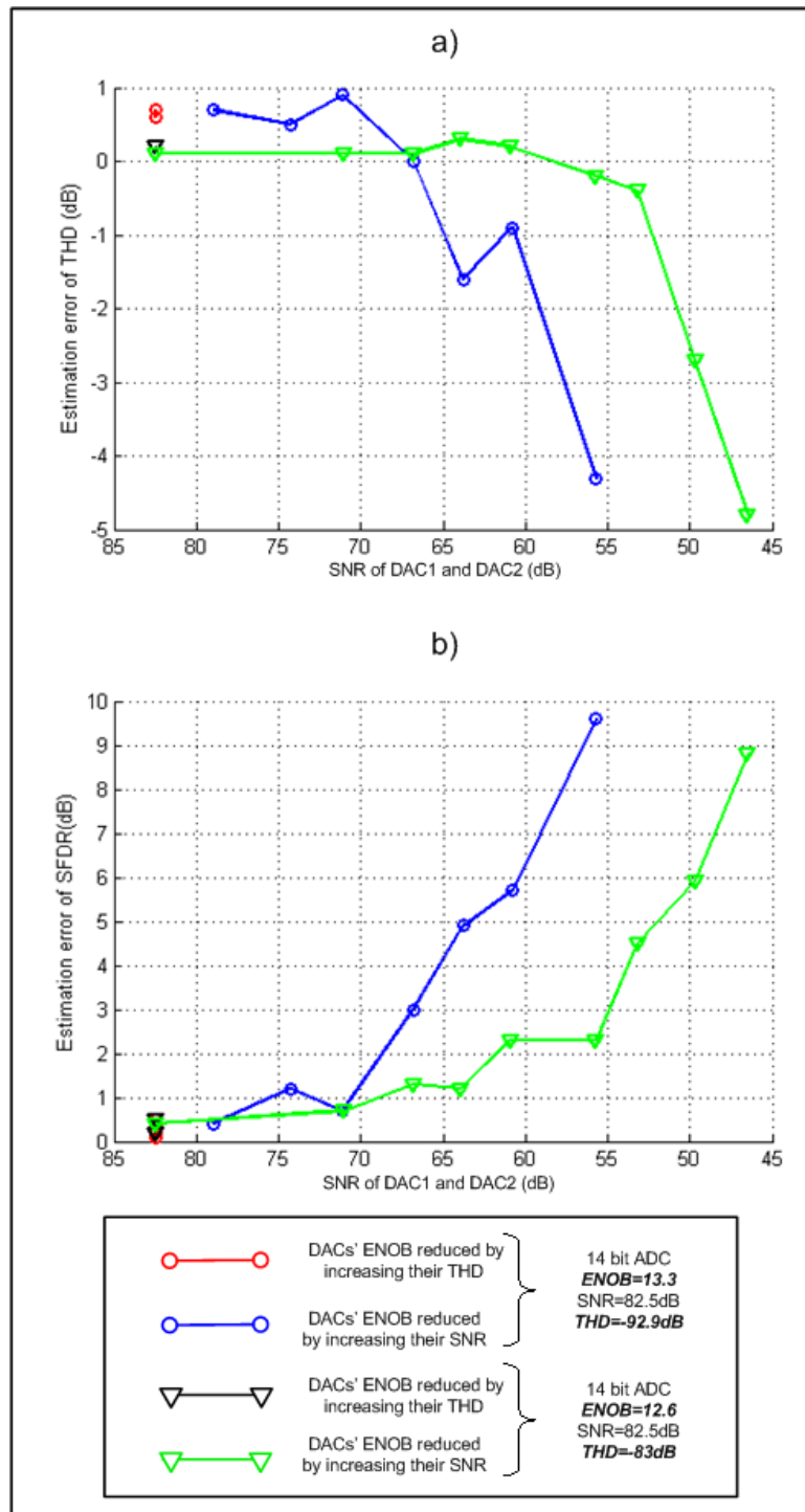
Figure 3-6: a) THD estimation error vs. SNR of DACs b) SFDR estimation error vs. SNR of DACs
