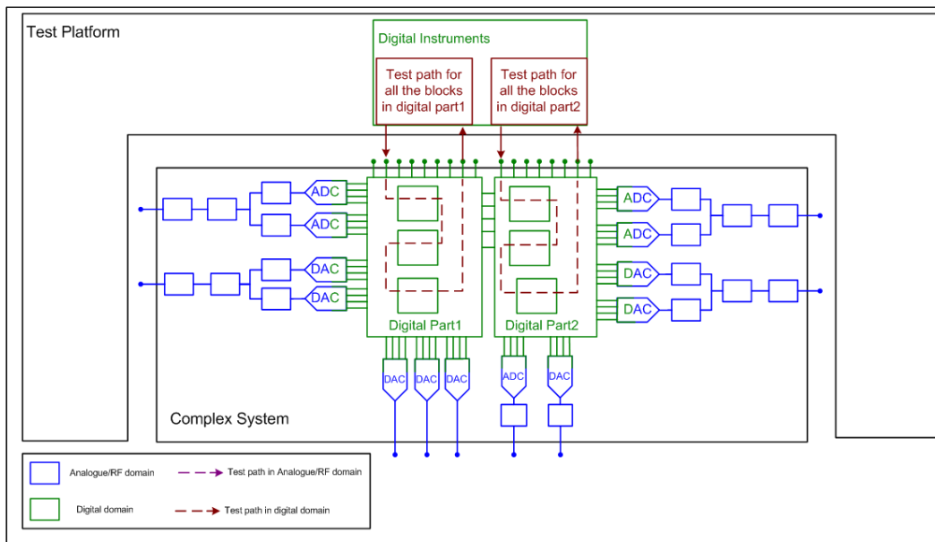
Figure 1-11: Test of digital cores from potential system
