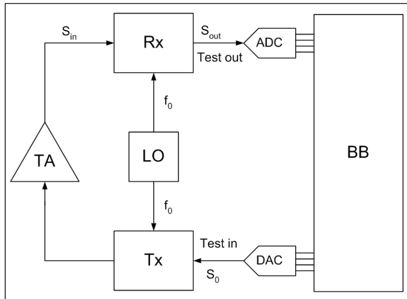
Figure 1-25: Loopback principle with Tx and Rx operating at the same carrier frequency [dabr04]
