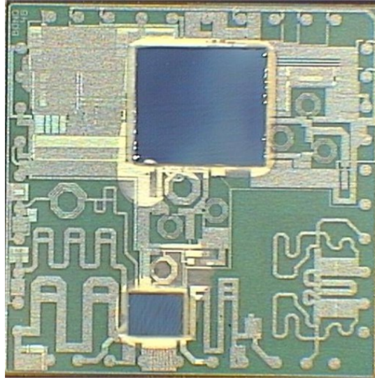
Figure 1-9: Example of SiP made of two active dies stacked on a passive one
