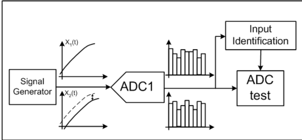
Figure 4-1: Basic principle of the SEIR approach [jin05_2]
