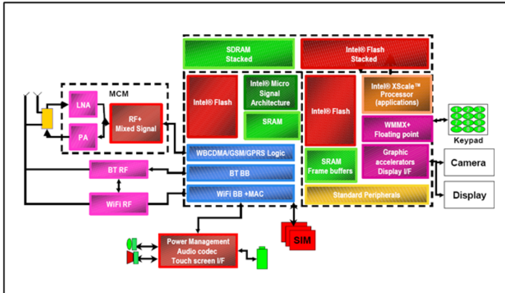
Figure 1-3: Intel pxa800f
