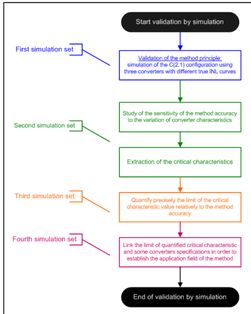
Figure 3-4: Simulation strategy in order to validate the test approach
