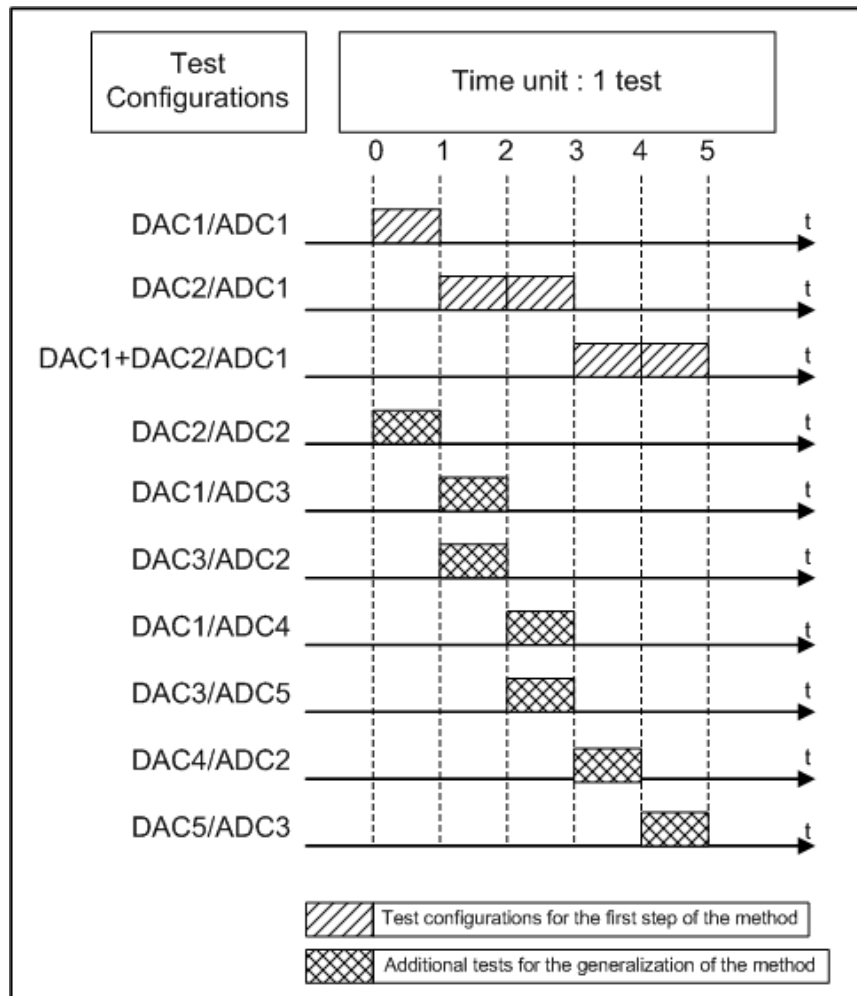
Figure 2-33: Temporal description of the test configurations for the generalization of the method
