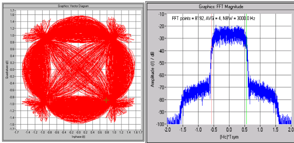
Figure 1-20: Constellation and spectrum of a QPSK modulated sine wave at 4.096MHz, with distortion
