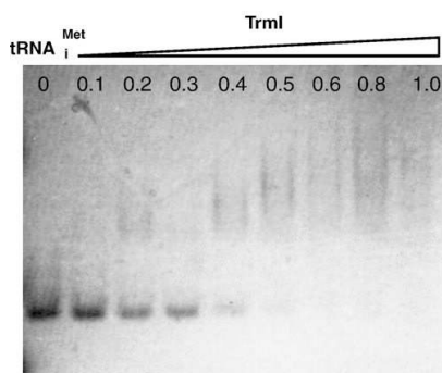
Fig. 4. Nondenaturing agarose gel electrophoresis. Constant amount of E. coli tRNA i Met (4 µg) with increasing amounts of th TrmI protein (from 0 to 1 molar equivalent of th TrmI tetramer). Bands were visualized by UV shadowing.
