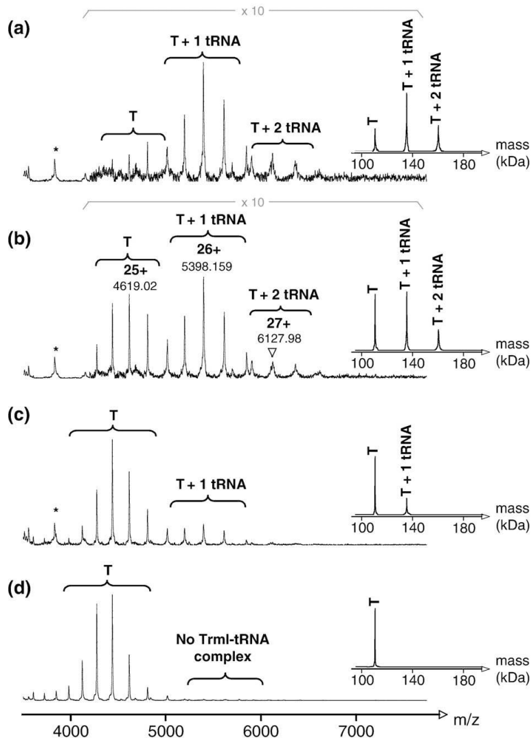
Fig. 5. Influence of the buffer ionic strength on thTrmI -tRNA complex stabilities. ESI mass spectra obtained under nondenaturing conditions (ammonium bicarbonate, pH 8.0; V_c=120 V; P_i=6.1 mbar) for thTrmI tetramer (20 \mu M) in the presence of 100 \mu M E. coli tRNA i Met . Ammonium bicarbonate concentration was set to (a) 100 mM, (b) 200 mM, (c) 400 mM, and (d) 1250 mM. Insets correspond to deconvoluted spectra showing molecular weights on the x-scale. T corresponds to ( thTrmI ) 4 ; T+1tRNA corresponds to the ( thTrmI ) 4 :(tRNA) 1 complex; and T+2tRNA corresponds to the ( thTrmI ) 4 :(tRNA) 2 complex. *tRNA signals.
