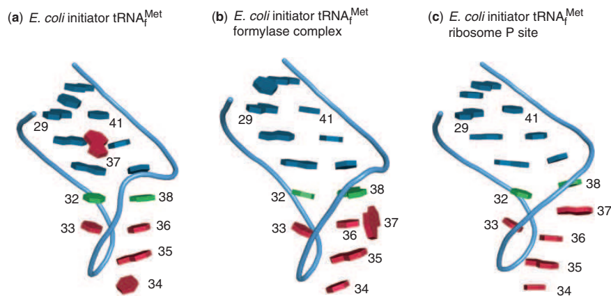
Figure 5. Comparison of the anticodon loop base stacking. (a) E. coli tRNA f Met , (b) E. coli tRNA f Met in the complex with formylase (PDB ID 2FMT), (c) in the P-site (PDB ID 2J00). The '37-unstacked' conformation refers to (a) and (b) structures and the '37-stacked' to the (c) one.
