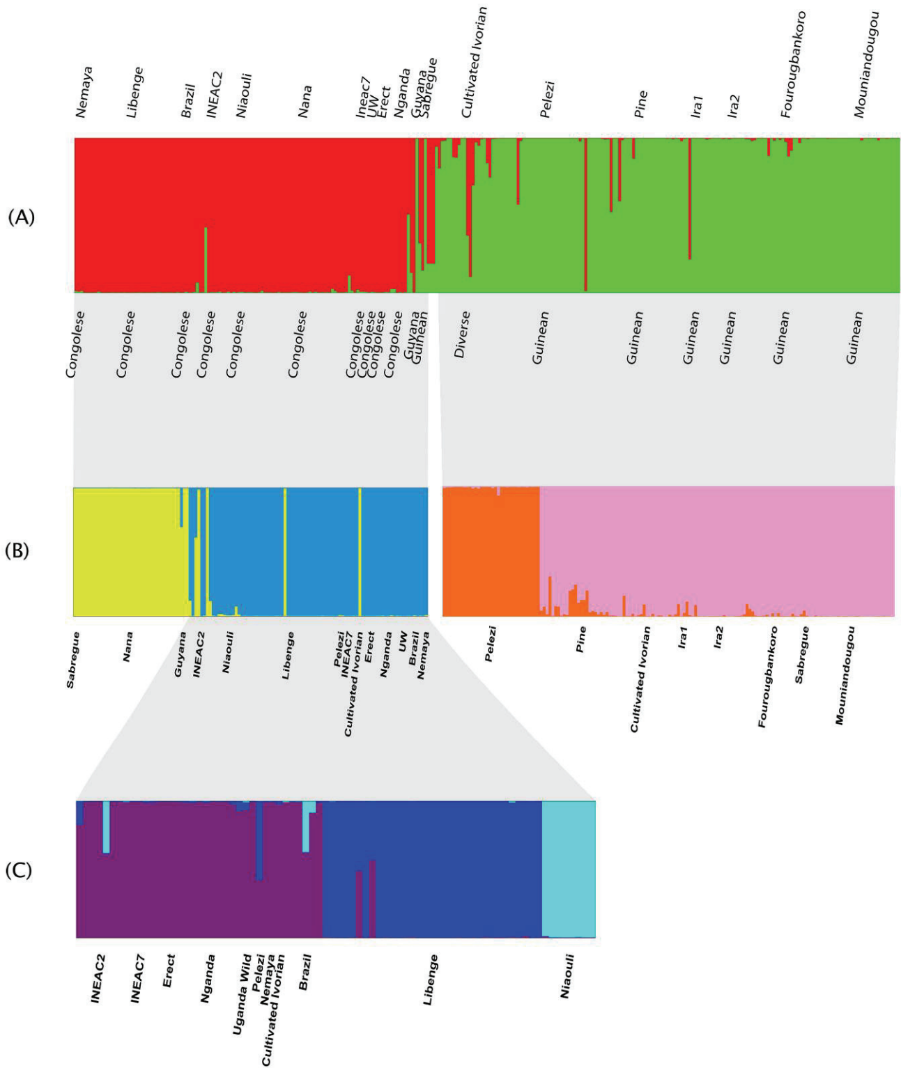
Figure 3.2: Structure outputs on different levels of structure investigation. (A) = Structure output for the whole sample, K=2, Congolese group (red) and Guinean group (green). Lower labels are for the putative origin of the populations, upper labels are the populations names. (B) = Structure outputs for the two datasets (Congolese on the left, Guinean on the right) of the 2 nd level of investigation. Yellow = C, Blue = Other Congolese, Orange = Pelezi, Pink = Other Guinean (C) = Structure output for the “Other Congolese” group for the 3 rd level of investigation. Purple = SG2, Dark-Blue = B, Light-Blue = SG1.
