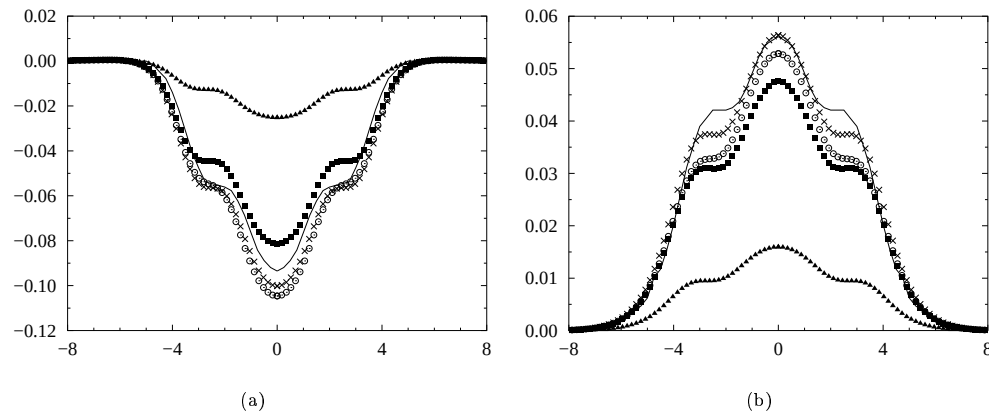
Figure 1: ID40 at 150 kHz, real part (a) and imaginary part (b) of the variation of the probe impedance \Delta Z ( \Omega ) along the x -axis (mm); measurement (solid line), full solution (crosses), LN (open circle), QLS (solid triangle), QA (solid square)
