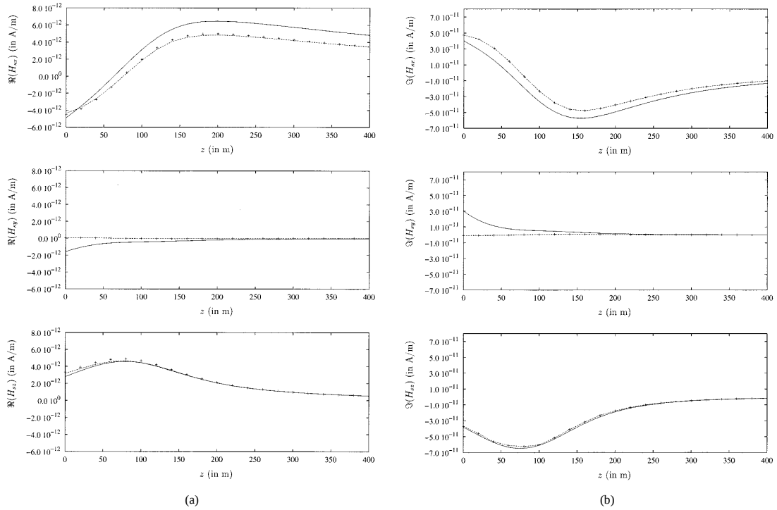
Fig. 4. Vertically-oriented elongated triaxial ellipsoid ( a_1 = 62 m, \mathbf{x}_1/z , a_2 = 31 m, \mathbf{x}_2/y , a_3 = 15.5 m, \mathbf{x}_3/x ) of conductivity \sigma_e = 2 \times 10^{-2} S/m is buried at p = 75 m in a less conductive Earth ( \sigma = 2 \times 10^{-3} S/m) and is illuminated by a 500 Hz, 1 Am 2 vertically-orientated magnetic dipole at ( x_S = 100 m, y_S = 0 , z_S = 75 m). (a) Real parts and (b) imaginary parts of the components of the secondary magnetic field are calculated along a ( x_R = -50 m, y_R = 90 m) vertical line: exact expansion (EE) results in the case of the half space (---) and for an infinite space (+ + +), MoM results (—).
