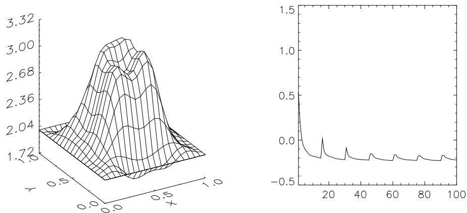
Figure 6. Reconstruction at 300 MHz of the square obstacle displayed in figure 2 with a 20 \times 20 -pixel mesh and refreshment every 15 iterations (left) and evolution of the log of the cost functional F_n against the iteration number (right). The inversion is started from the map obtained by a previous inversion led at 200 MHz. The data are corrupted with a 10 dB noise.
