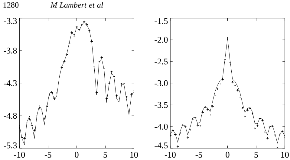
Figure 13. The 400 MHz scattered field(in dB) yielded by the inversion after 100 iterations and corresponding to the retrieved obstacle displayed in figures11 and 12 (crosses) is compared with the exact one (full curve) for the firstand most eccentric line source (left) and the eighth and central line source (right).
