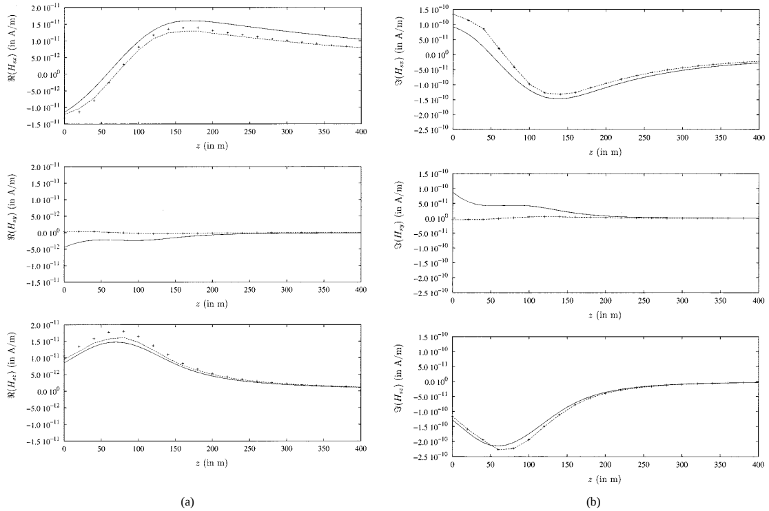
Fig. 6. Plate-like, vertically-oriented oblate spheroid ( a_1 = 62 m, \mathbf{x}_1/\mathbf{z} , a_2 = 62 m, \mathbf{x}_2/\mathbf{y} , a_3 = 15.5 m, \mathbf{x}_3/\mathbf{x} ) of conductivity \sigma_e = 2 \times 10^{-2} S/m is buried at p = 75 m in a less conductive Earth ( \sigma = 2 \times 10^{-3} S/m) and is illuminated by a 500 Hz, 1 \text{ Am}^2 vertically-orientated magnetic dipole at ( x_S = 100 m, y_S = 0 , z_S = 25 m). (a) Real parts and (b) imaginary parts of the components of the secondary magnetic field are calculated along a ( x_R = -50 m, y_R = 80 m) vertical line: EE in the case of the half space (---) and for an infinite space (+ + +), MoM results (—).
