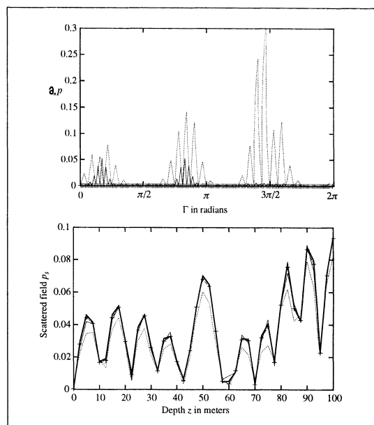
Figure 3. Same as Figure 2 for the sound-hard three-leaf clover obstacle with now M = 32 (dotted line), M = 64 (plain line) and M = 128 (cross symbol) whereas the boundary condition concerns the normal derivative of the total pressure.
