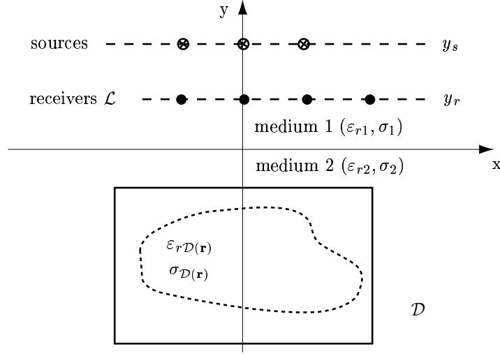
Figure 1. The geometrical and electrical configuration of study.
