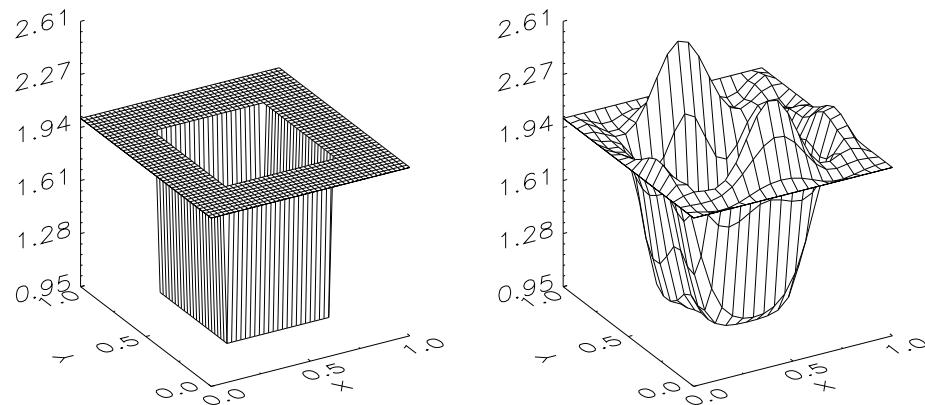
Figure 8. Reconstruction at 400 MHz and by frequency-hopping (four frequencies are used: 100, 200, 300, 400 MHz) of the lower-contrast square obstacle (relative permittivity equal to 1) with a 20 \times 20 -pixel mesh and refreshment each 15 iterations.
