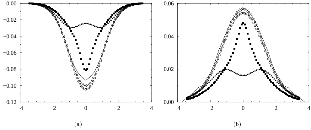
Figure 2: ID40 at 150 kHz, real part (a) and imaginary part (b) of the variation of the probe impedance \Delta Z ( \Omega ) along the y -axis (mm); measurement (solid line), full solution (crosses), LN (open circle), QLS (solid triangle), QA (solid square)
