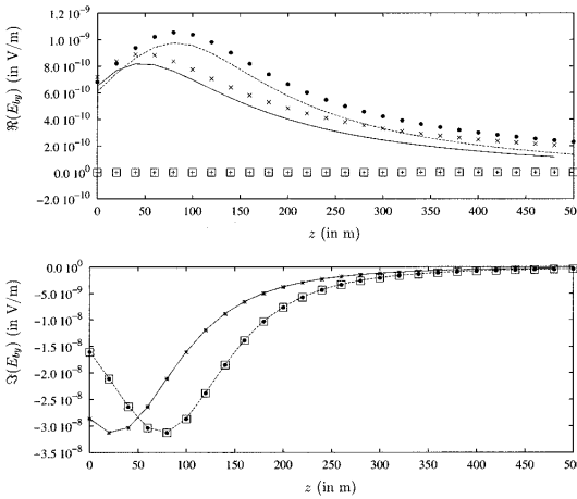
Fig. 3. Primary electric field due to a 500 Hz, 1 Am 2 vertically-orientated magnetic dipole (along z ) in the half-space Earth ( \sigma = 2 \times 10^{-3} S/m). Same as in Fig. 2, but the exact y -component values are now compared to those of its expansions up to powers (jk)^2 and (jk)^4 . z_S = 25 m, exact (—), (jk)^2 (+ + +), and (jk)^4 (× × ×); z_S = 75 m, exact (---), (jk)^2 (o o o), and (jk)^4 (□ □ □).
