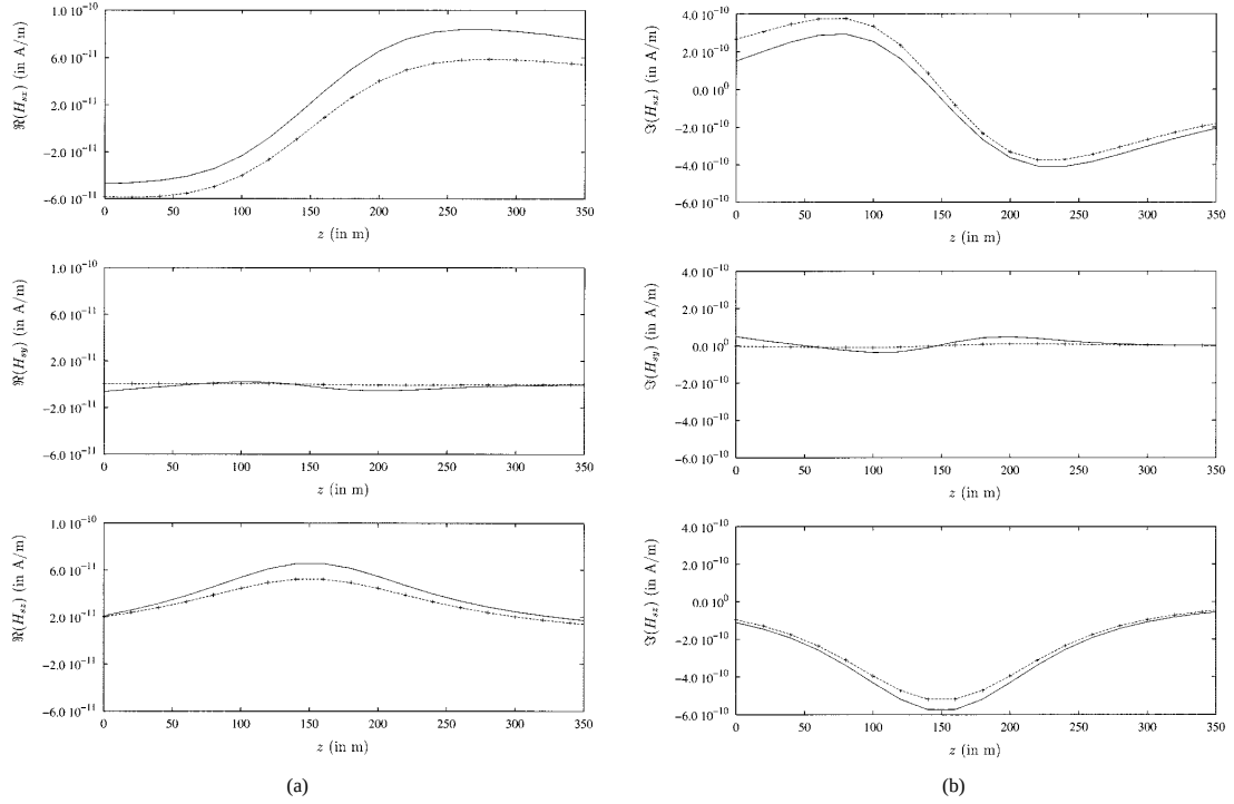
Fig. 7. Vertically-oriented elongated triaxial ellipsoid ( a_1 = 62 m, \mathbf{x}_1/z , a_2 = 31 m, \mathbf{x}_2/y , a_3 = 15.5 m, \mathbf{x}_3/x ) of conductivity \sigma_e = 2 \times 10^{-1} S/m (see Fig. 4) is buried at p = 150 m in a much less conductive Earth ( \sigma = 2 \times 10^{-3} S/m) and is illuminated by a 1000 Hz, 1 \text{ Am}^2 vertically-orientated magnetic dipole at ( x_S = 100 m, y_S = 0 , z_S = 150 m). (a) Real parts and (b) imaginary parts of the components of the secondary magnetic field are calculated along a ( x_R = -50 m, y_R = 90 m) vertical line: EE in the case of the half space (---) and for an infinite space (+ + +), MoM results (—).
