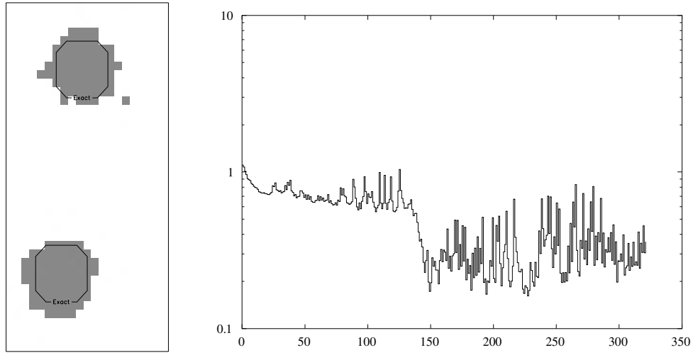
Figure 3. The two dielectric cylinders (TM data, twodiellTM_4f.exp): monochromatic data (at 8 GHz). Left: best result (227th iteration); right: variations of the objective function as a function of the number of iterations. The time step is \Delta t = 2 \times 10^{-2} .
