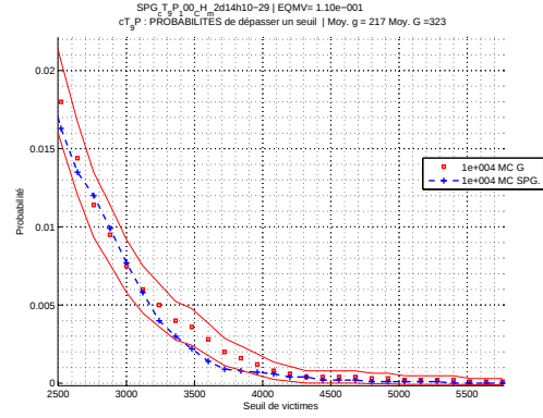
(b) Sparse grid g_{SC-100}
