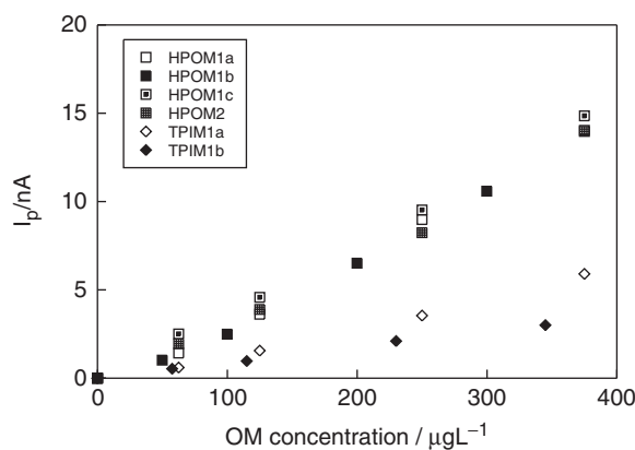
Figure 3. SWV response curves for OM isolated fractions from the WWTP Seine-Aval and the Seine River. OM concentrations are expressed in \mu\text{gL}^{-1} . Meaning of the abbreviations: HPO, hydrophobic; TPI, transphilic; HPI, hydrophilic; A1, WWTP April 2006; A2, WWTP Seine-Aval December 2006; AN: Seine River at Andrésy; Mt: Seine River at Méricourt.
