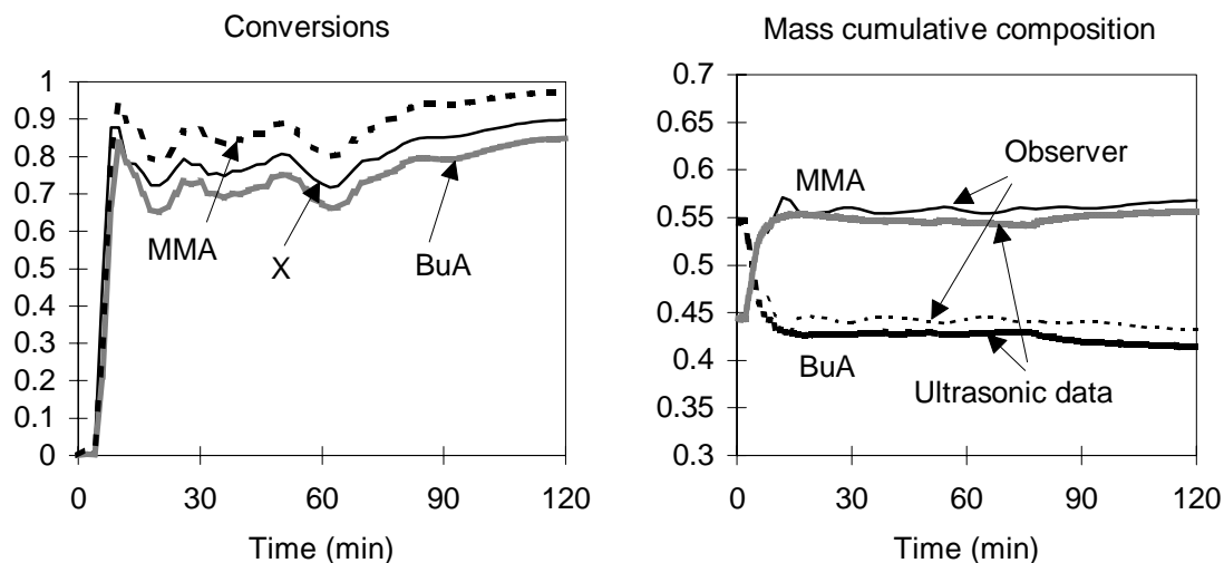
Figure 4.13: Experiment 14/11/97: Copolymerization of BuA and MMA. The overall conversion obtained by an ultrasonic probe and the individual conversions of MMA and BuA estimated by the observer, at left. At right, the estimated composition and its validation obtained by the ultrasonic sensor.
