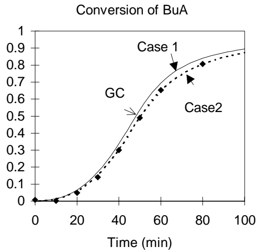
Figure 4.10b: Experiment BuA/STY 50-50. Case 1: K_{P11}=3.37 \times 10^7 , K_{P22}=2.97 \times 10^5 \text{ cm}^3/\text{mol/s} r_1=.18 , r_2=.95 , and in cases 2 : K_{P11}=2.47 \times 10^5 , K_{P22}=3.53 \times 10^5 \text{ cm}^3/\text{mol/s} r_1=.3 , r_2=.7 , for BuA and STY respectively.
