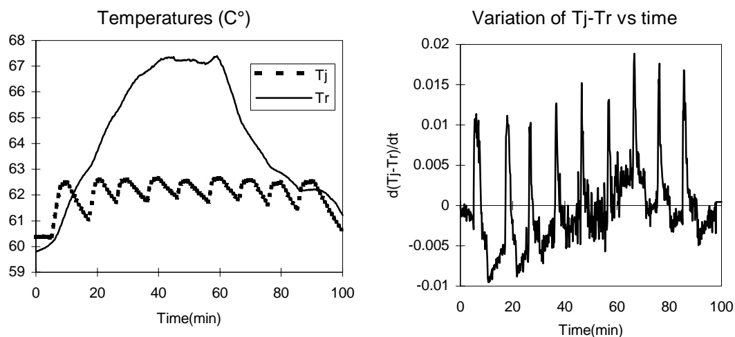
Figure 3.6a: Homopolymerization of styrene. Temperature ramps on the jacket temperature: T_j (--), at left. The corresponding value of d(T_j - T_R)/dt as a function of time, at right.
