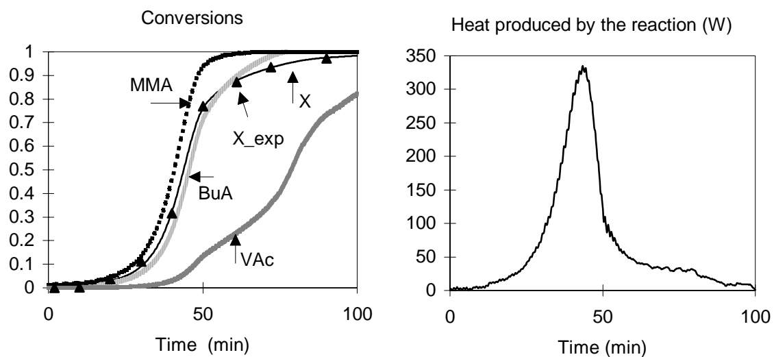
Figure 5.4: MMA-BuA-VAc-1. Overall conversion ( X ) obtained by calorimetry fitted to the experimental ( X_{exp} ) conversion and the estimated individual conversions obtained by the observer, at left. At right, the heat produced by the reaction.
