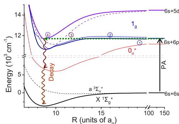
FIG. 5. (Color online) Theoretical \text{Cs}_2 molecular potential curves including spin orbit [25,26], relevant for the present PA and cold molecule formation process. The PA laser excites levels of a long-range 1_g curve (label 1), which is coupled to the v=0 level of the short-range 1_g curve (label 4) through several avoided crossings involving 1_g curves labeled 2 and 3. Formation of a deeply bound ground-state molecule proceeds through a spontaneous emission cascade via the 0_u^+ states.
