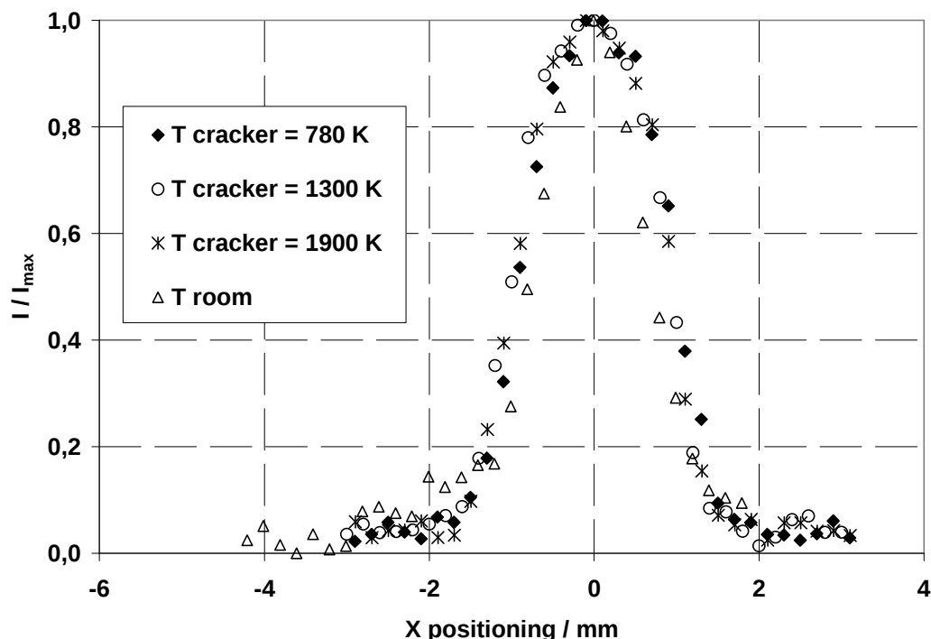
Figure V-16: X axis scanning of the CHIP reactor effusion orifice position under Ar flow when varying the cracking cell temperature. The ion \text{Ar}^+ is monitored at mass 40.
