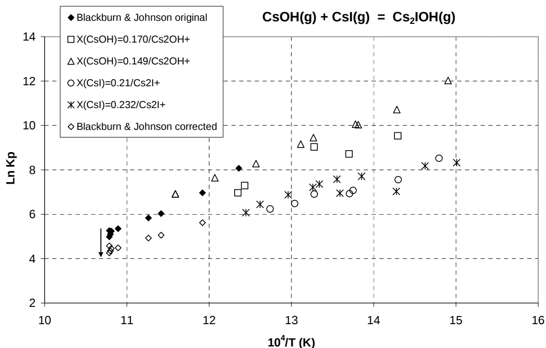
Figure IV-17: Experimental equilibrium constant for the reaction \text{CsOH(g)} + \text{CsI(g)} = \text{Cs}_2\text{IOH(g)} as determined using the only \text{Cs}_2\text{OH}^+ ionic intensity from \text{Cs}_2\text{O}_2\text{H}_2\text{(g)} and \text{Cs}_2\text{I}^+ ionic intensity from \text{Cs}_2\text{I}_2\text{(g)} as measured when vaporizing different CsI-CsOH mixtures and comparison with Blackburn and Johnson original data with the \text{Cs}_2\text{OH}^+ ion. Blackburn and Johnson data have been corrected according to our selected value for the CsOH dimerization constant (see text).
