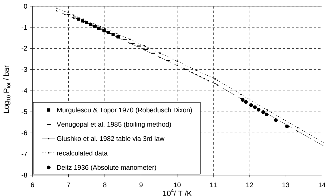
Figure III-12: Total pressure determinations over CsI given by different authors and comparison with recalculated data using our selected K_{\text{dim}} and CsI(s,l) enthalpy of vaporization = 194.83 \text{ kJ.mol}^{-1}
