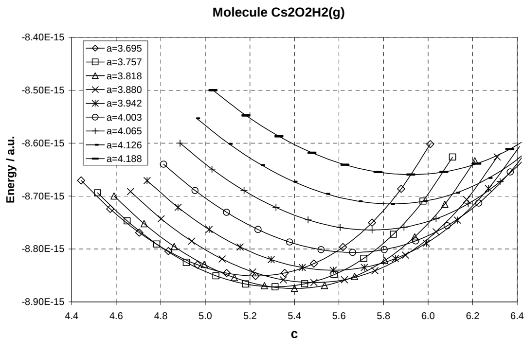
Figure IV-25: Cs 2 O 2 H 2 (g) ionic model results and its inter-atomic distance optimization for a minimum potential energy
