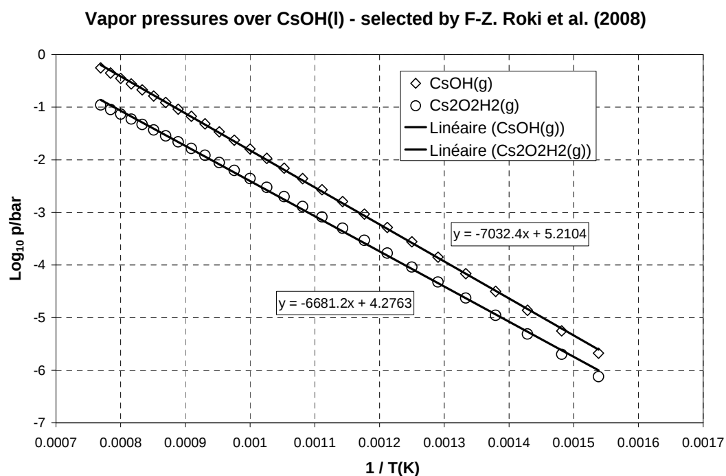
Figure II-4: Selected CsOH(g) and Cs 2 O 2 H 2 (g) vapor pressures over liquid phase
