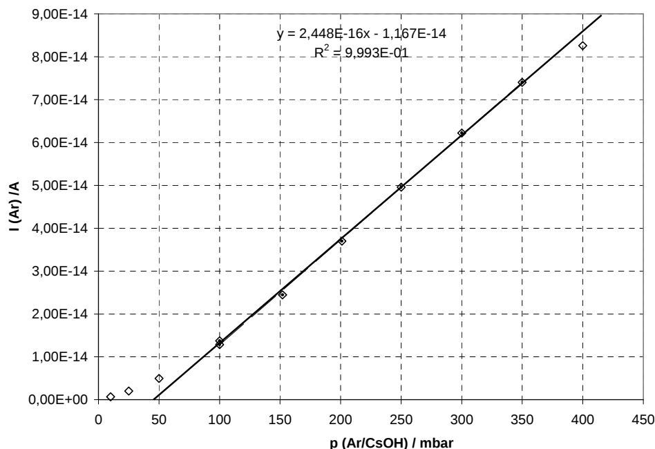
Figure V-17: test of Ar/CsOH line using argon gas. Ionic intensity of \text{Ar}^+ as a function of the input pressure at the nozzle. Other lines: Ar/ \text{H}_2 / \text{H}_2\text{O} line constant at 100 mbar (without any input flow because of a defectuous pressure sensor) and Ar/ \text{I}_2 line off (the nozzle is clogged).
