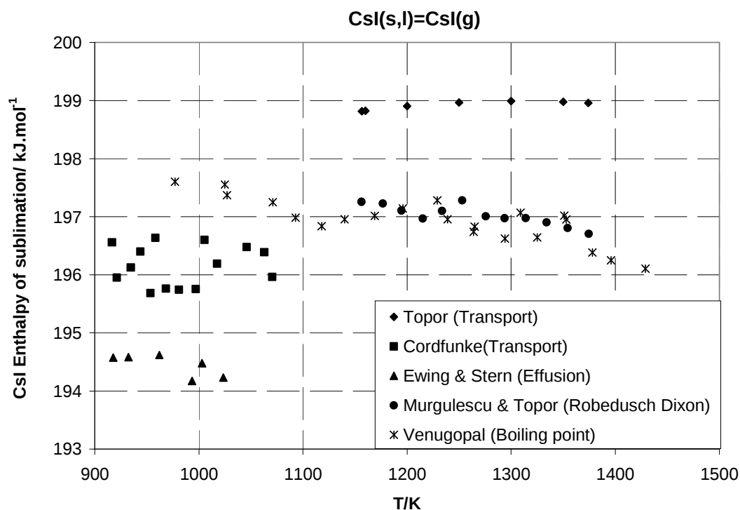
Figure III-9: Third law \text{CsI(g)} enthalpy of sublimation calculated from experimental determinations performed over the liquid phase as a function of temperature of measurements.
