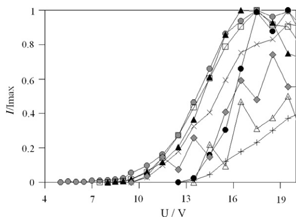
FIGURE 8. An example of the ionization efficiency curves obtained during the MS vaporization of \text{CsOH} in a cell of Gold. \bullet : \text{Cs}^+ , \square : \text{Cs}_2\text{OH}^+ , \blacktriangle : \text{CsOH}^+ , \times : \text{Cs}_2\text{O}^+ , \triangle : \text{CsO}^+ , \bullet : \text{Cs}_2\text{H}^+ , \diamond : \text{Cs}_3\text{O}_2\text{H}_2^+ , + : \text{H}_2\text{O}^+ .
