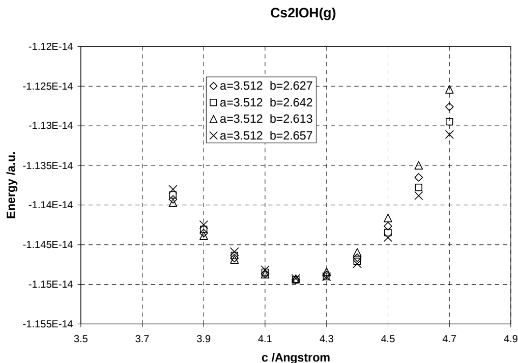
Figure IV-26: \text{Cs}_2\text{IOH(g)} ionic model results and its minimum potential energy
