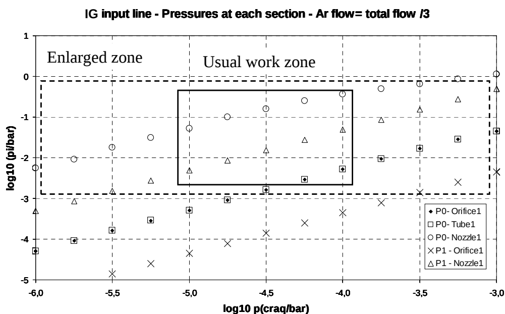
Figure V-5: Pressures calculation in different sections: from IG line (Iodine/Ar), the nozzle1 ( 50 \mu\text{m} diameter), connection tube (Tube1, 12 mm diameter) and orifice 1 of introduction in the cracking cell (orif1, 30 \mu\text{m} diameter). Calculation is carried out with a flow in the line equal to 1/3 total flow at the cracking cell exit.
