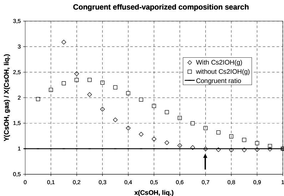
Figure IV-2: Test for congruent composition in the vaporization of CsI-CsOH liquid phase when taking or not into account the \text{Cs}_2\text{IOH(g)} molecule as proposed by Blackburn and Johnson. The arrow shows the congruent composition attained only when taking into account the new molecule.
