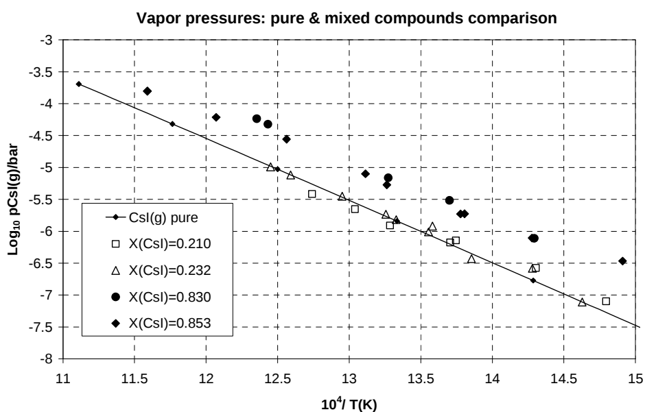
Figure IV-11: Experimental vapor pressure of \text{CsI(g)} in equilibrium with different CsI-CsOH mixtures and comparison with our selected vapor pressure for the pure CsI compound.(this work, chapter III)
