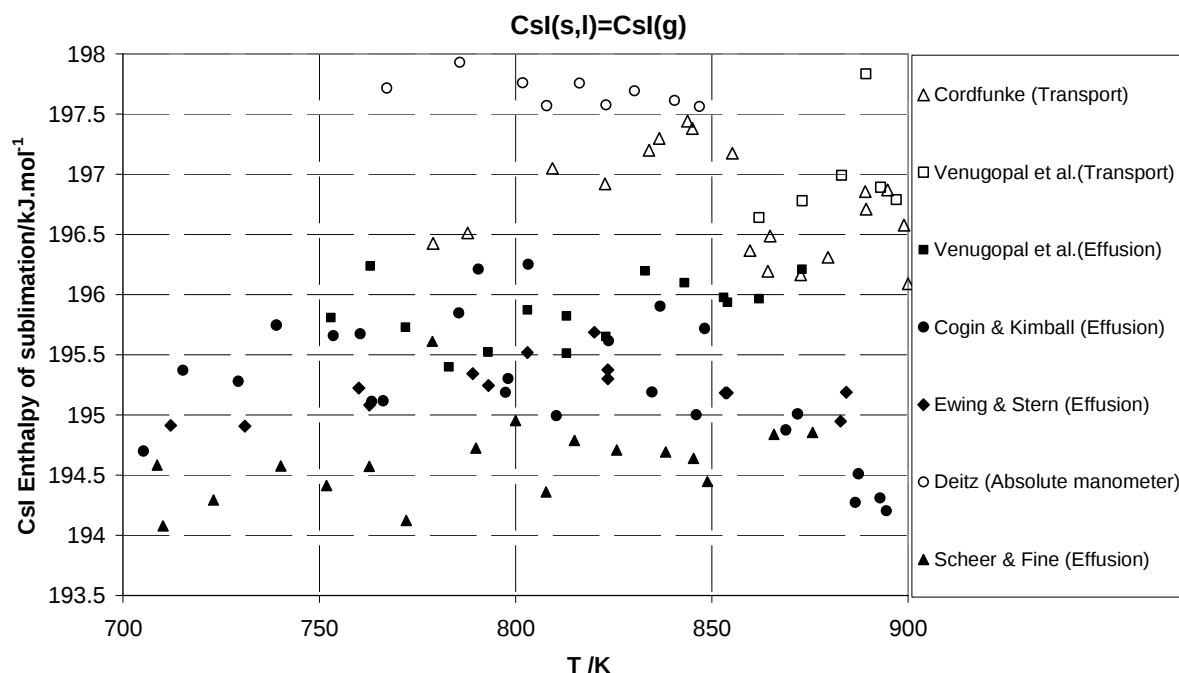
Figure III-8: Third law \text{CsI(g)} enthalpies of sublimation calculated from experimental determinations performed over the solid phase as a function of temperature of measurements.
