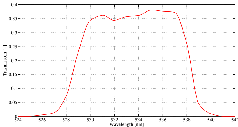
Figure 2.12.: Spectral response of the linear channel interference filter (data provided by SESO)
