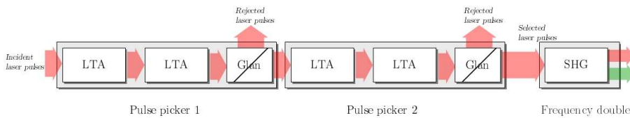
Figure 3.1.: The pulse picker - frequency doubler assembly (LTA: birefringent crystal, Glan: polarizer, SHG: second harmonic generation)
