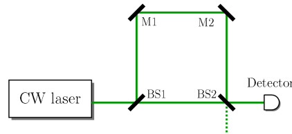
Figure 7.2.: Mach-Zehnder interferometer: The light is divided by the beam splitter BS1, retarded by \Delta t in the long branch, and recombined on the second beam splitter BS2.
