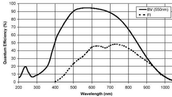
Figure 3.11.: Quantum efficiency (‘BV’) of the Andor DW 436 N camera (graph from [36])
