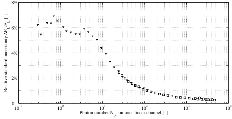
Figure 5.4.: Relative precision or 1\text{-}\sigma uncertainty of the linear pulse measurement. It is given here over the corresponding photon number N_{\text{ph}} on the non-linear channel. The photon number present on the linear channel is more than 10^3 higher.
