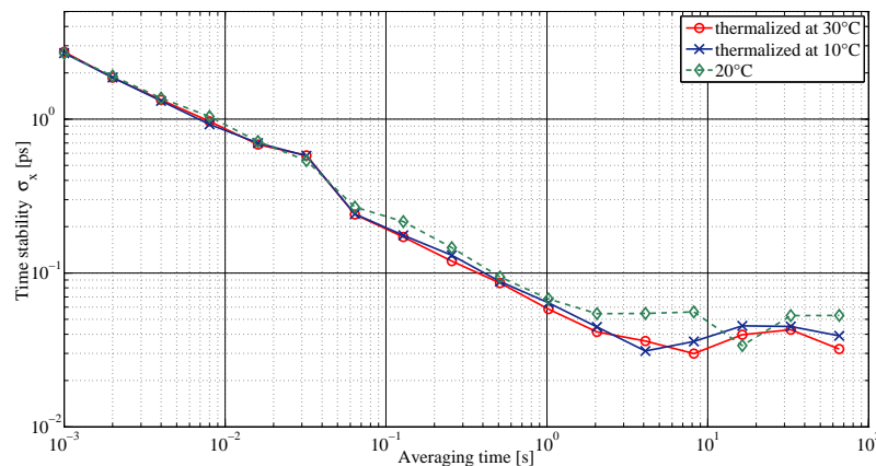
Figure 3.36.: Time stability of the T2L2J2 frequency synthesis phase compared to reference phase same (the plot of 20°C corresponds to a dataset of a somewhat less thermalized experiment)
