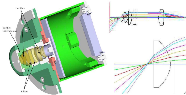
Figure 2.11.: The mechanical and optical layout of the linear channel. CAD-view and ZEMAX simulation © SESO, France
