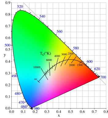
Figure 3.13.: The CIE x,y-color space
