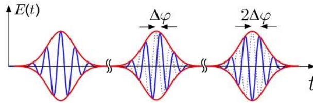
Figure 7.6.: Carrier-envelope delay of a free-running femtosecond laser
