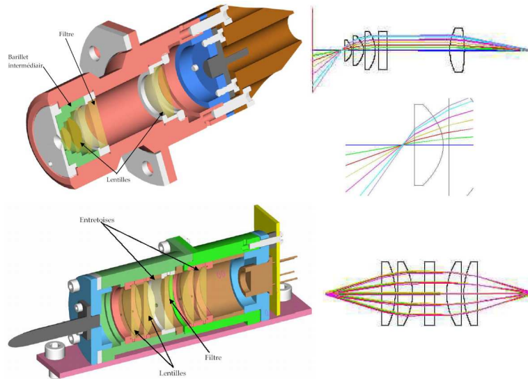
Figure 2.14.: The collimation optics BONL of the non-linear detection channel located outside the satellite body and the coupling optics OCTO located in the electronics unit. CAD-view and ZEMAX simulations © SESO, France
