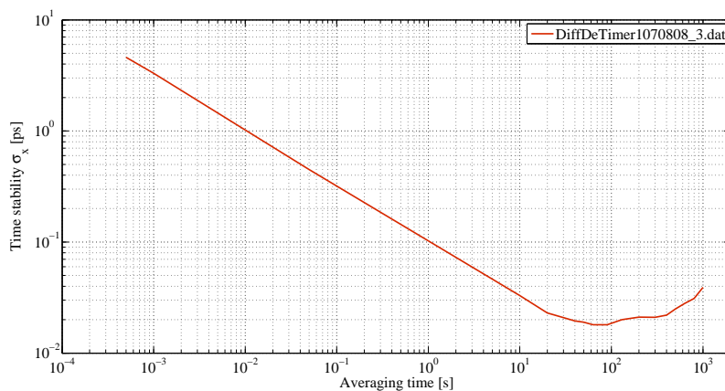
Figure 8.11.: Time stability plot of the differential measurement
