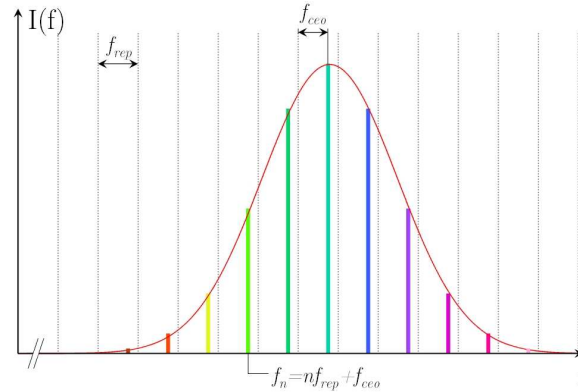
Figure 7.7.: Spectral properties of a frequency comb
