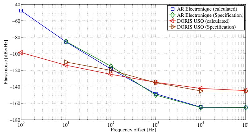
Figure 2.16.: Combined phase noise of DORIS oscillator and event timer local oscillator AR Electronique
