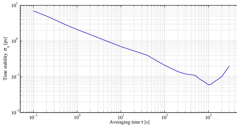
Figure 3.27.: Time stability of Dassault Electronique event timer
