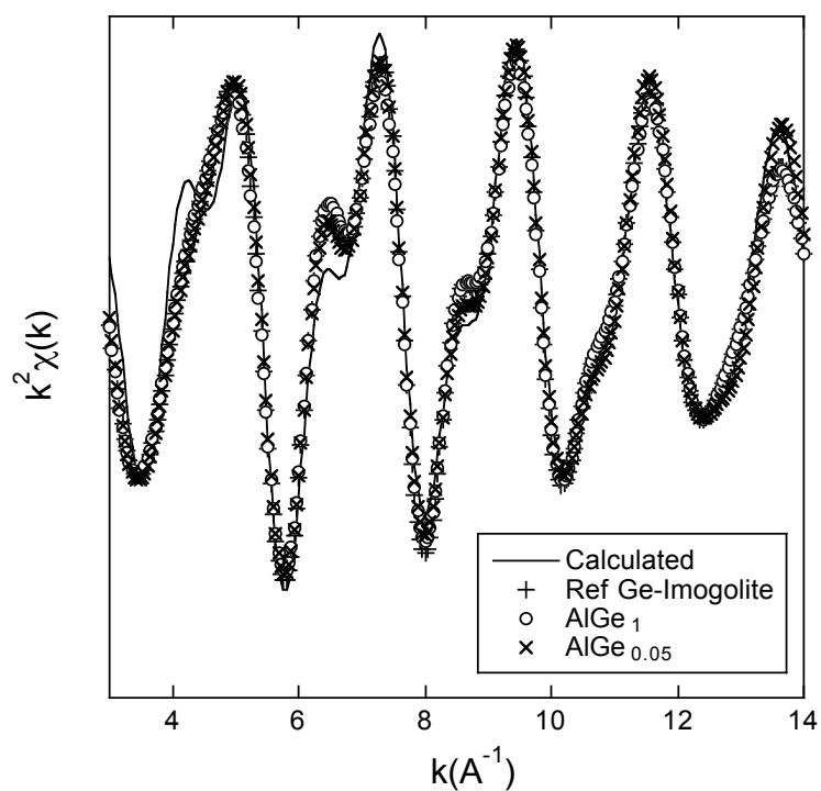
Figure S1. Partial EXAFS spectra (1-3.47 \text{\AA} ) of AlGe 1 and AlGe 0.05 synthesized from a decimolar concentration and comparison with the Ge-imogolite reference synthesized from a millimolar concentration.
