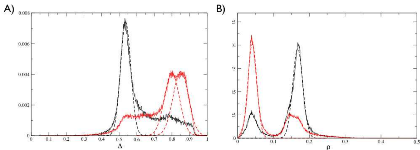
Figure 31: Panel A : Normalized distributions for Oriental Distance \Delta in \mathbb{A} (in black ) and in \mathbb{B} (in red ). Fitted Gaussian functions are shown in dashed lines. Correlation coefficients between distributions and fitted curves are between 0.90 and 0.96. Panel B : Normalized distribution for the helix radii \rho in \mathbb{A} (in black ) and in \mathbb{B} (in red ). Fitted Gaussian functions are shown in dashed lines. Correlation coefficients are between 0.94 and 0.96.
