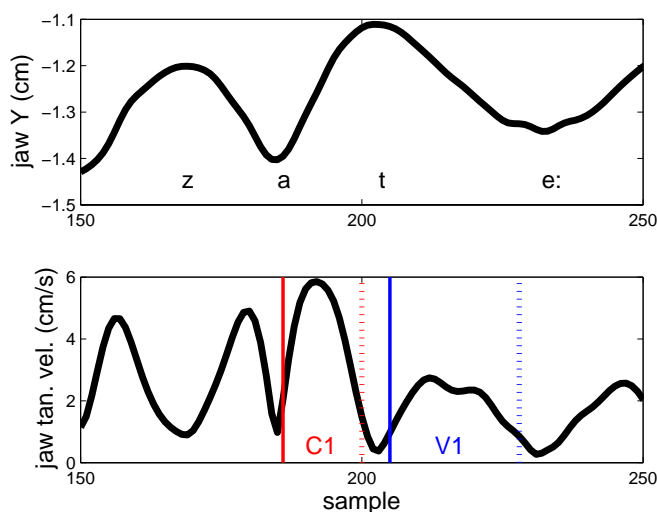
Figure 4.3: Example for measurements of articulatory gestures in the sequence /za'te:/ ( sah from the carrier phrase and beginning of test word teeta ). Upper subplot: Vertical movement of the jaw sensor. Lower subplot: Corresponding tangential velocity. Red vertical lines mark beginning (solid) and end (dotted) of the consonantal gesture leading towards C1, blue vertical lines mark beginning (solid) and end (dotted) of the vocalic gesture leading towards V1. Beginning and end of each gesture are 20% above a velocity minimum.
