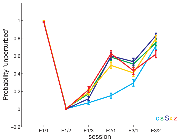
Figure 7.1: Mean probability over speakers to belong to the group of unperturbed productions. Each line gives the results for one sound. Error bars show standard error. Colours as indicated: cyan: /ç/, green: /s/, blue: /ʃ/, yellow: /x/, red: /z/.
