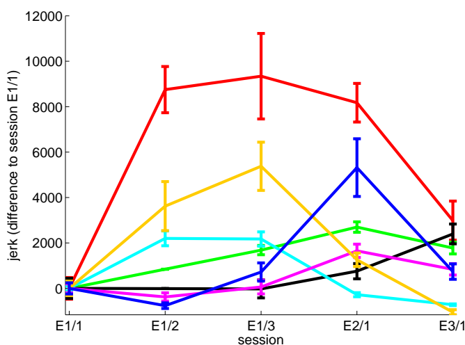
Figure 11.1: Differences in jerk to session E1/1 during the tongue tip gesture towards /o/. Different colours correspond to different speakers. TP: red, KD: green, OP: black, SK: cyan, BP: magenta, DS: yellow, AP: blue. Error bars show standard error.
