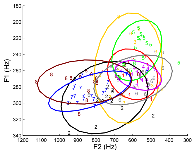
Figure 5.2: F2 (abscissa) and F1 (ordinate) values of /u/ for speaker TP. Colours and numbers denote different sessions in chronological order (cf. figure 5.1). Ellipses (2 standard deviations) show the subregions of the vowel.
