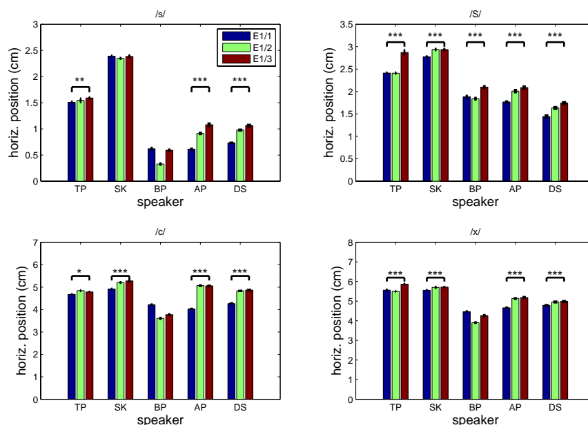
Figure 9.2: Mean horizontal position of the consonantal target position in four fricatives over the first three recordings. Higher values denote more retracted positions. Error bars show standard error. When the difference between sessions E1/1 and E1/3 is significant this is signalled by a bracket above the bars. Significance levels: * p < 0.05 , ** p < 0.01 , *** p < 0.001 . If there is no increase from E1/1 to E1/3 the significance levels are not given.
