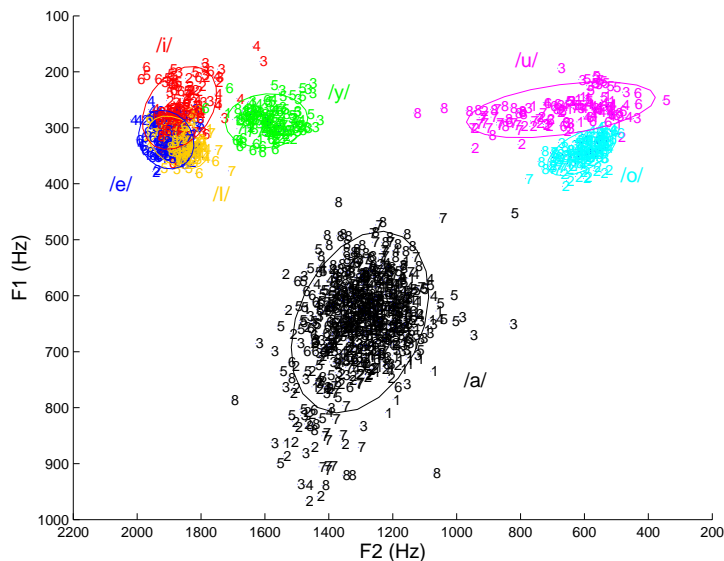
Figure 5.1: F2 (abscissa) and F1 (ordinate) of the vowels produced by speaker TP. The colours denote different sounds, the numbers denote the sessions: 1: E1/1, 2: E1/2, 3: E1/3, 4: AU1, 5: E2/1, 6: AU2, 7: E3/1, 8: E3/2.
