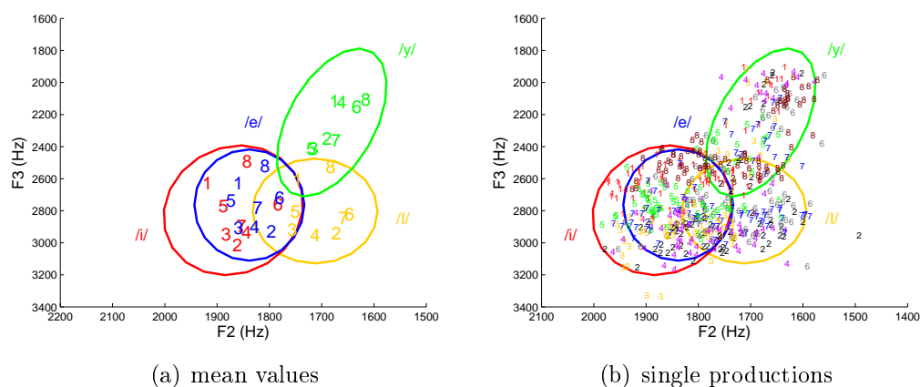
Figure 5.3: F2-F3 space for the productions of /i, e, ɪ/ and /y/ of speaker DS. Left: Coloured numbers give means of sessions in chronological order (cf. figure 5.1, coloured ellipses (2 standard deviations) the regions corresponding to a phoneme. Right: Coloured numbers give single productions with colours corresponding to sessions. Coloured ellipses give regions corresponding to a phoneme.
