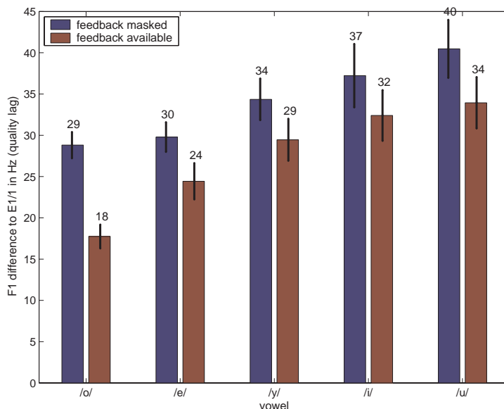
Figure 8.1: "Quality lag" (difference F1 in Hz between the pre-perturbed productions and the perturbed productions) for the session with auditory feedback masked (blue) and with auditory feedback available (brown) for the five vowels investigated. Error bars show standard error.
