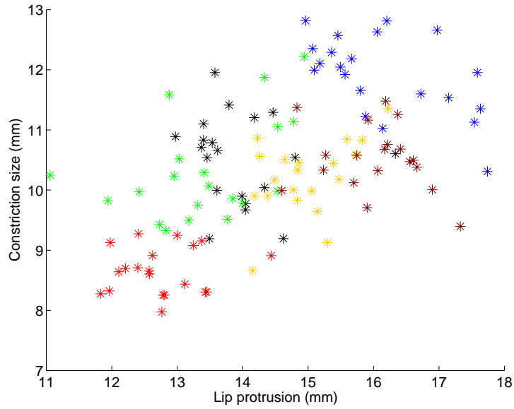
Figure 10.1: Lip protrusion and constriction size measurements for speaker DS. Different colours represent different sessions: E1/1: red, E1/2: black, E1/3: yellow, E2/1: green, E3/1: blue, E3/2: brown.
