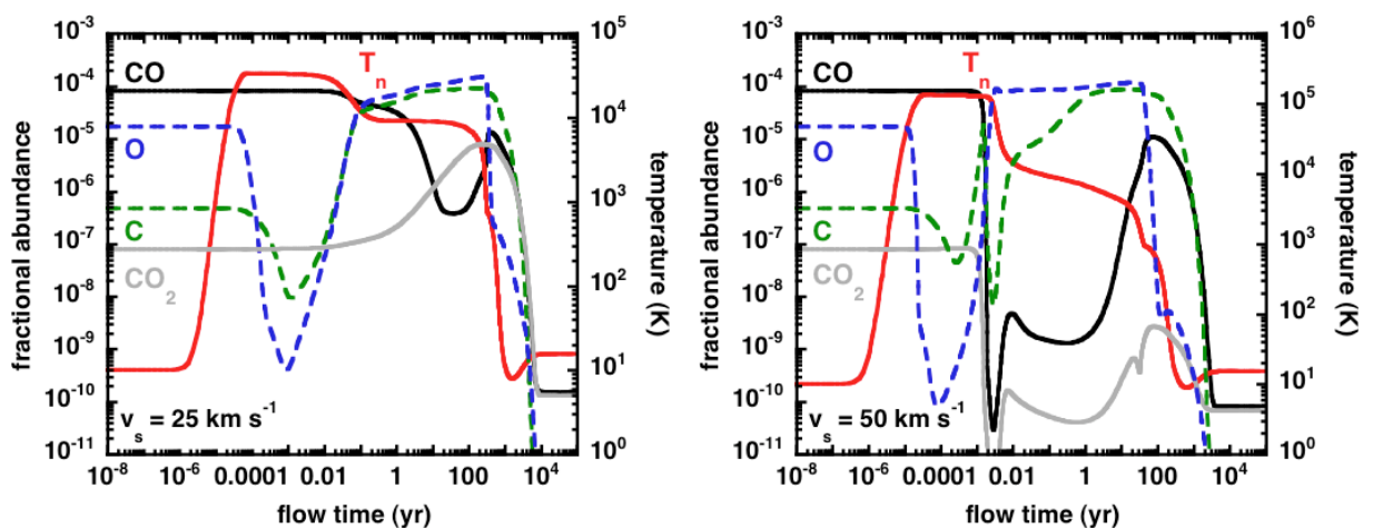
Figure 11.3 – CO production in J-type reference shock models : n_{\text{H}} = 10^4 \text{ cm}^{-3} , b = 1 , v_s = 25 (left panel) and 50 \text{ km s}^{-1} (right panel). C, O, CO, \text{CO}_2 fractional abundance and temperature profiles.
