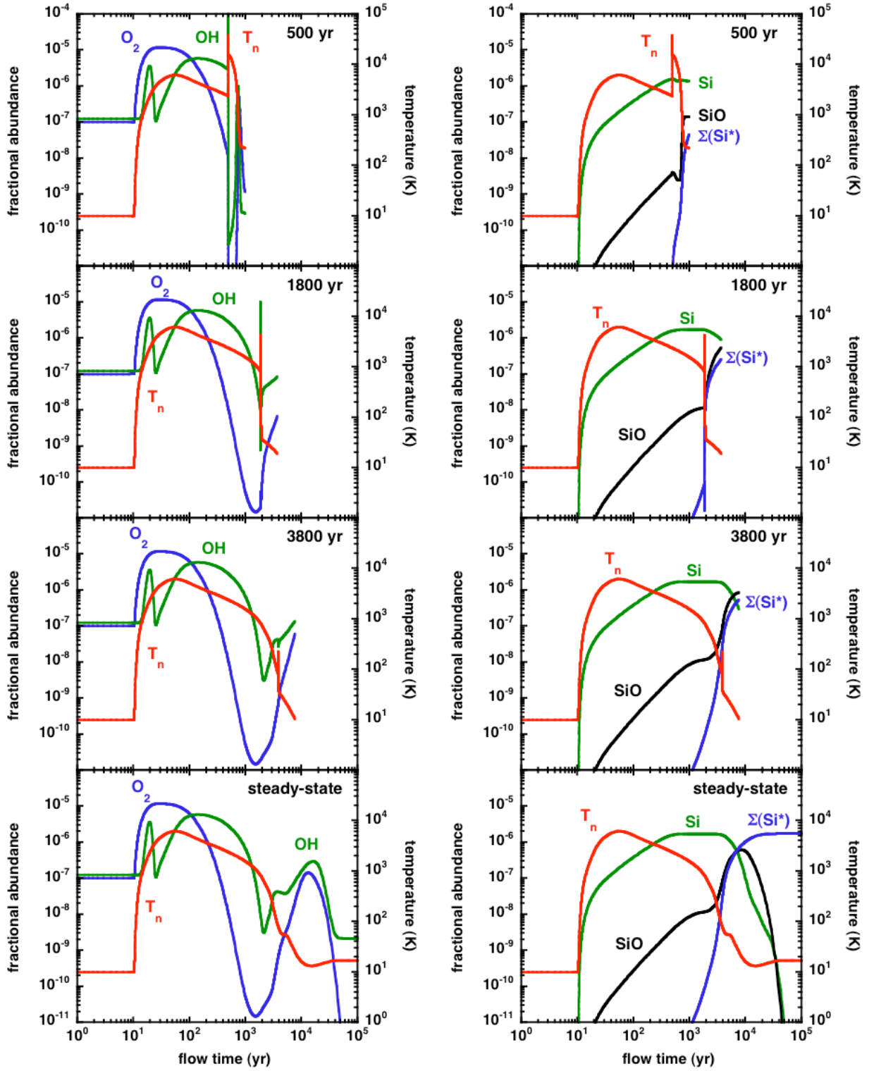
Figure 10.8 – The temperature of the neutral fluid, T_n , and the fractional abundances of OH and O_2 (left-hand panels) and of Si, SiO, and silicon in the grain mantles, \Sigma Si^* (right-hand panels), as functions of the flow time of the charged fluid, for the CJ-type shock model in which n_H = 10^4 \text{ cm}^{-3} , b = 1 , and v_s = 50 \text{ km s}^{-1} . The shock age increases from top to bottom : 500, 1800, 3800 years, and steady-state. In these calculations, there is no SiO in the grain mantles, and the gas-phase silicon is produced solely by erosion of the silicate grain cores.
