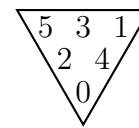
\Delta S_6
