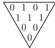
\Delta S_7
