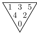
\Delta S_3
