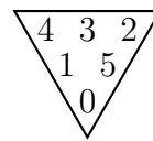
\Delta S_5
