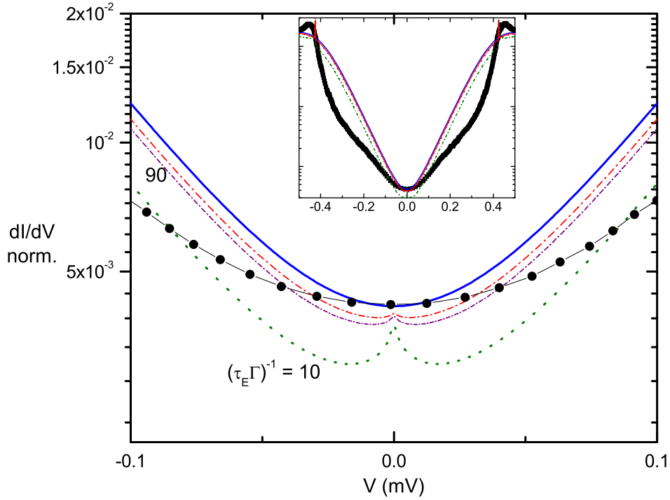
Figure 5.11: Differential conductance plot (Sample B) at T = 330 mK of cooler junction along with the simulated curve at different relaxation time \tau_E \Gamma^{-1} = 10, 50 and 90 at low bias. Inset shows the complete curve.
