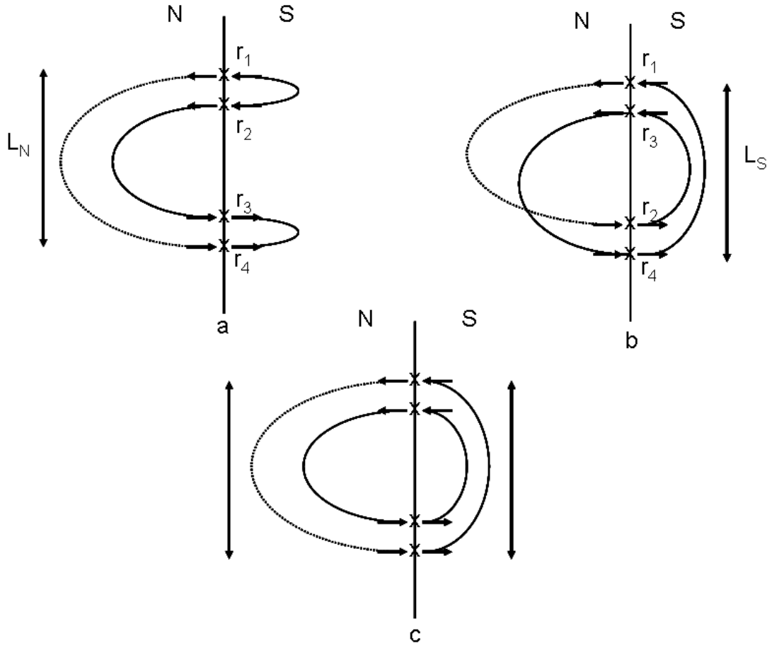
Figure 3.8: Contribution to the sub-gap conductivity due to interference in (a) the normal electrode, (b) the superconducting electrode, and (c) both electrodes.
