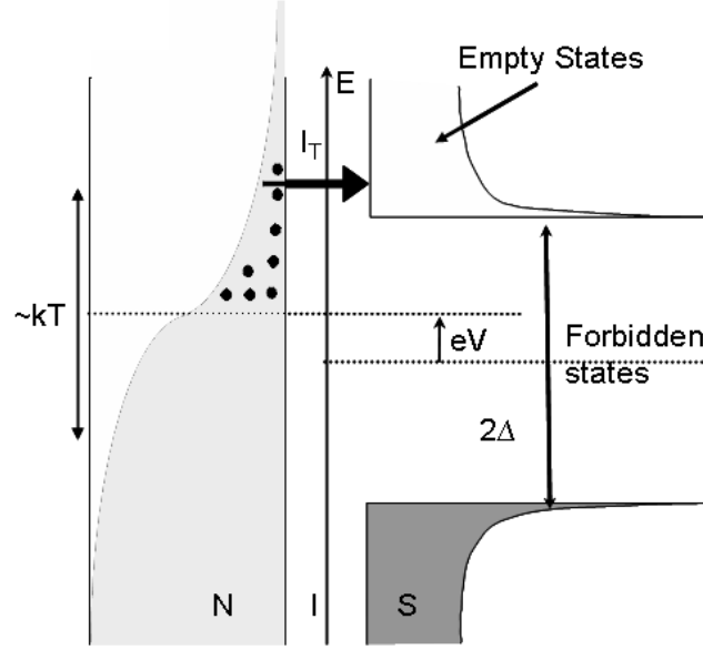
Figure 2.1: Density of states vs energy schematic of a N-I-S junction showing single quasiparticles transfer across the junction.
