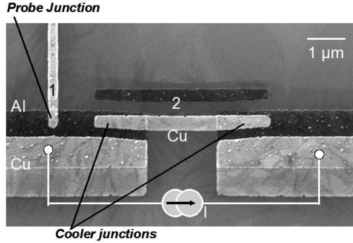
Figure 5.5: Sample B: Scanning electron micrograph of a cooler with no external thermometer on the central N-island. Cooler junctions are two Al-AlO(x)-Cu junctions in series. The area of a cooler junction is 1.5 \mu\text{m} \times 0.3 \mu\text{m} . In addition to the cooler there is one of the three Al-AlO(x)-Cu probe junction on one of the superconducting arm of the cooler junction.
