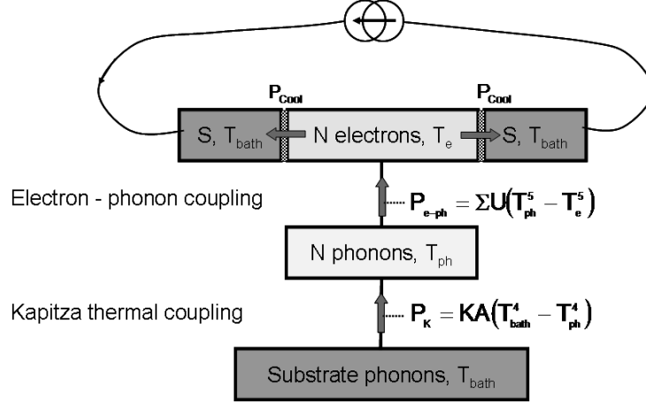
Figure 7.6: Schematic of the thermal model.
