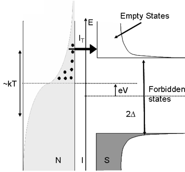
Figure 1.1: Density of states vs energy schematic of a N-I-S junction showing single quasiparticles transfer across the junction.
