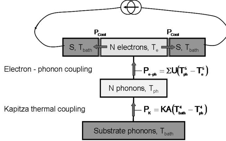
Figure 6.4: Heat flow paths between the different constituents in the cooler.
