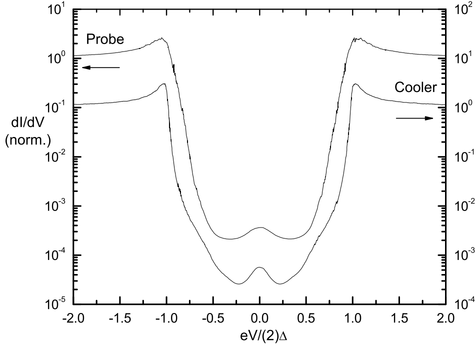
Figure 7.5: Sample C: Differential conductance at a cryostat temperature of 90 mK. Top curve - the dI/dV of one probe junction 1.55 \mu\text{m} from the cooler junction which has been fitted in the previous section with the phase-coherent Andreev current and the single quasiparticle current (see left y-axis). The normal state resistance of the probe junction, R_N = 2.76 \text{ k}\Omega . Bottom curve: cooler junction data (see right y-axis) with normal state resistance, R_N = 1.9 \text{ k}\Omega .
