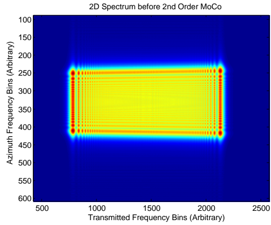
Figure 4.13: 2D Spectrum before 2^{nd} Order MoCo
