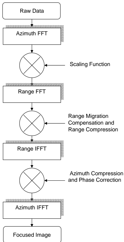
Figure 2.14: Block Diagram of the Chirp Scaling Algorithm
