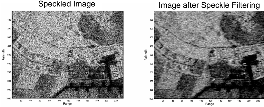
Figure 5.3: Speckled Image and Speckle Filtered Image
