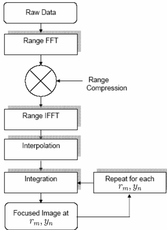
Figure 1.11: Block diagram of the Backprojection Algorithm ( r_m and y_n represent the m^{\text{th}} range and n^{\text{th}} azimuth bin, respectively)
