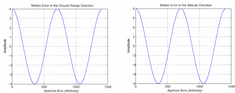
Figure 4.6: Simulated Motion Errors in Ground-Range and Altitude Directions
