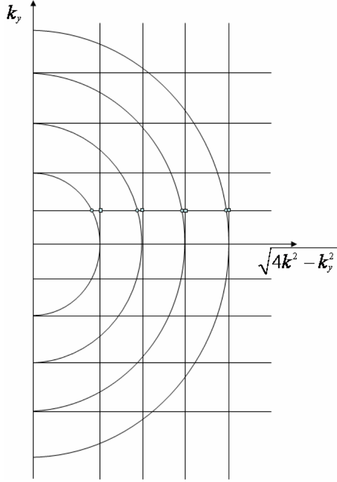
Figure 2.4: Stolt Interpolation
