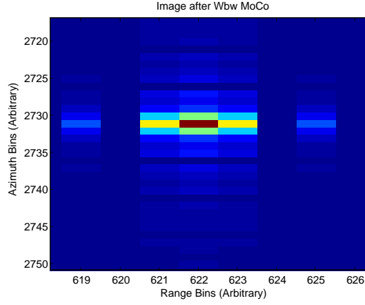
Figure 4.11: Raw Data Processing with Wbw MoCo (16° Aperture Angle)
