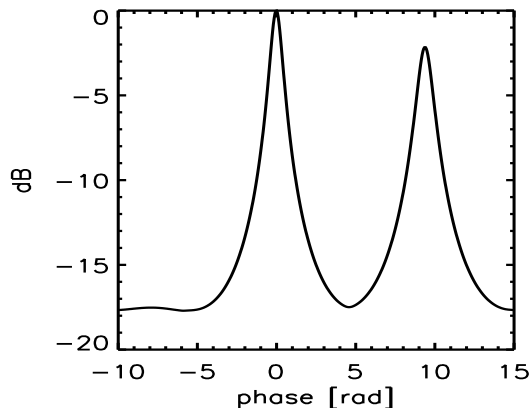
Figure 4.3: Polarimetric MUSIC pseudo-spectrum including two sources.
