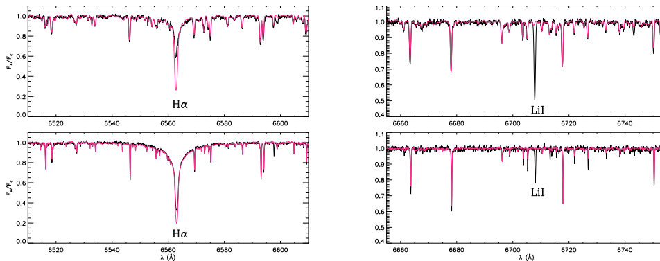
Figure 1. Observed AURELIE spectra (black lines) in the H\alpha (left panels) and Lithium (right panels) regions for a very young lithium-rich PMS candidate (top panels) and a fairly young star (low panels). The template spectra built up with “non-active” standard stars are over-plotted with red lines.
