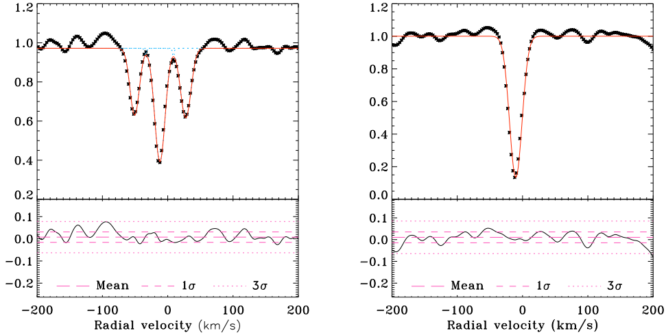
Figure 3. The CCFs of RasTyc 2034 at two orbital phases. The triple system nature appears from the CCF displayed in the left panel, while it is completely hidden at the phase of observation shown in the right panel. The RV uncertainty is about 1 km/s at our spectral resolution. The multiple Gaussian fits of the CCFs are over-plotted with full lines (top boxes) and the residuals of the fits are plotted in the lower boxes.
