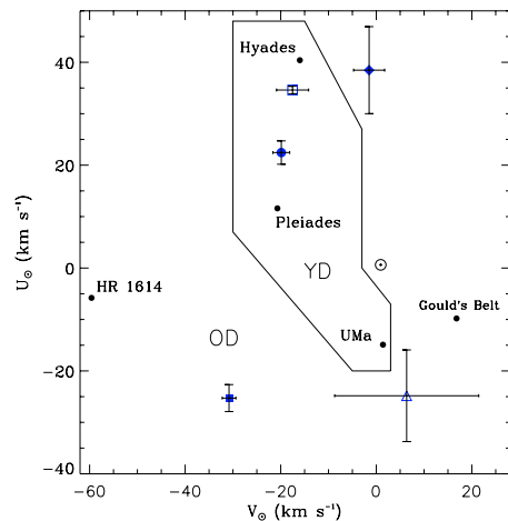
Fig. 6. Space velocities, U , V , of the RasTyc sources in the galactic plane. The meaning of the symbols is the same as in Fig. 4. The locus of the young-disk (YD) and the old-disk (OD) populations and the average velocity components of some moving groups (Eggen 1996) and of the Gould's Belt (Lindblad et al. 1997) are also indicated.
