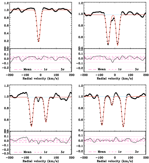
Fig. 2. The CCFs of RasTyc 0524+6739 at various orbital phases. These CCFs permit emphasis of the change of configuration from a one-peak shape at a conjunction ( left top panel ) to a three-peak shape ( right lower panel ), passing through phases of partial blending in which only two peaks are easily distinguished ( left lower panel and right top panel ). The RV uncertainty is about 1 \text{ km s}^{-1} at our spectral resolution. On each panel, the multiple Gaussian fits of the CCFs are over-plotted with full lines ( top box ) and the residuals of the fits are plotted in the lower box .
