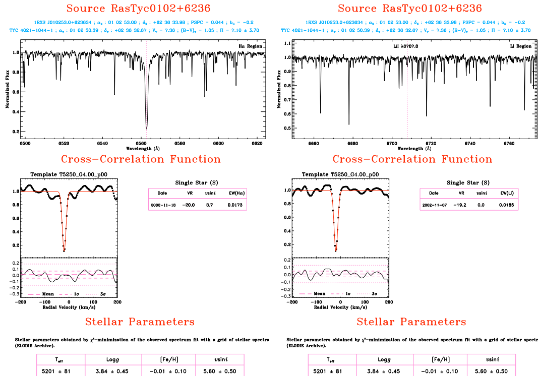
Fig. 14. Summary files of the single star HD 6026 (RasTyc 0102+6236) in the H\alpha (left panel) and lithium (right panel) spectral regions.
