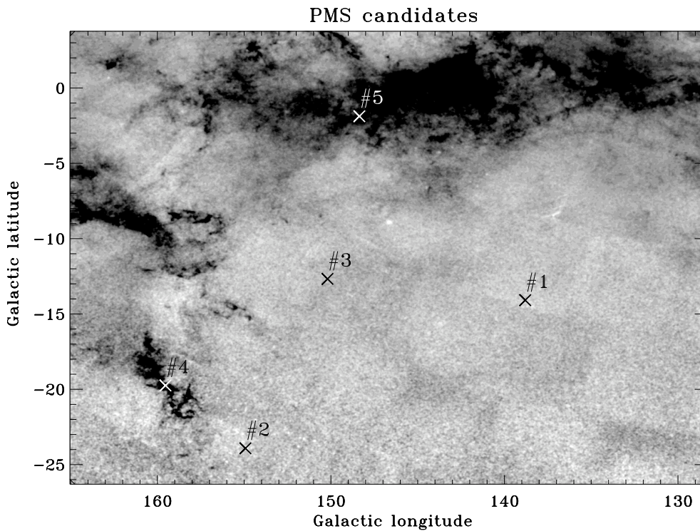
Fig. 10. Position (galactic coordinates) of PMS-like candidates overlotted on a map of dark clouds enhancing interstellar material (see #i next to cross symbols for cross-match with Tab. 4)
