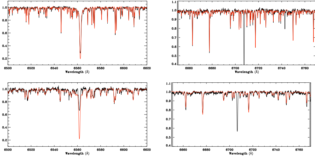
Fig. 13. H\alpha (left panel) and lithium (right panel) spectra (black solid line) of lithium-super-rich giants RasTyc 0319+4212 and RasTyc 1825+6450 (from top to bottom) together with the synthetic spectrum built up with the reference spectra broadened at the v \sin i of the star's components and Doppler-shifted according to its RV (thin red line).
