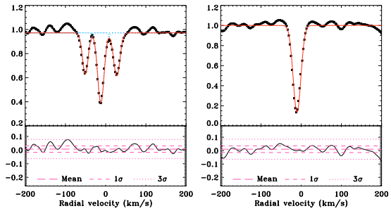
Fig. 4. The CCFs of RasTyc 2034+8253 at two orbital phases. The triple system nature appears from the CCF ( left panel ), while it is completely hidden at another phase of observation ( right panel ).
