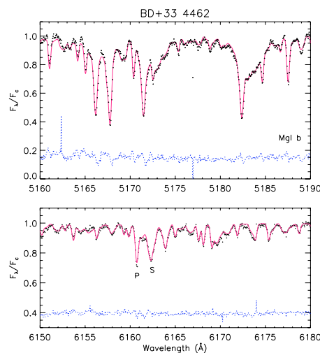
Fig. 3. Observed ELODIE spectrum of BD+33 4462 (dots) in the MgIb ( upper panel ) and in the \lambda 6170 Å ( lower panel ) regions. The “synthetic” spectrum (F7IV + K0III-IV) is displayed with thin lines in the same boxes. Each box also displays the difference (observed – synthetic) with a thin dotted line.
