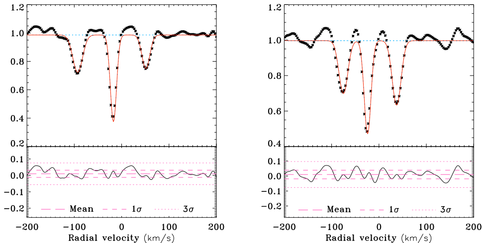
Figure 4. The CCFs of RasTyc 1828 clearly show three peaks with different widths. The two components of the inner binary appear to rotate faster than the third star, probably due to spin-orbit synchronization.
