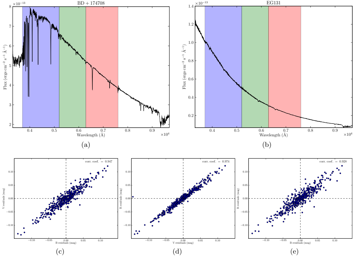
Figure 11.3: (a) BD+174708 and (b) EG131 spectrophotometric standard stars spectra. Residuals’ (difference of the synthesized magnitude and the median magnitude per filter) color correlation for the 6 spectrophotometric standard stars, for (c) V vs. B, (d) R vs. V and (e) R vs. B. The correlation coefficients are respectively 0.947, 0.974 and 0.928.
