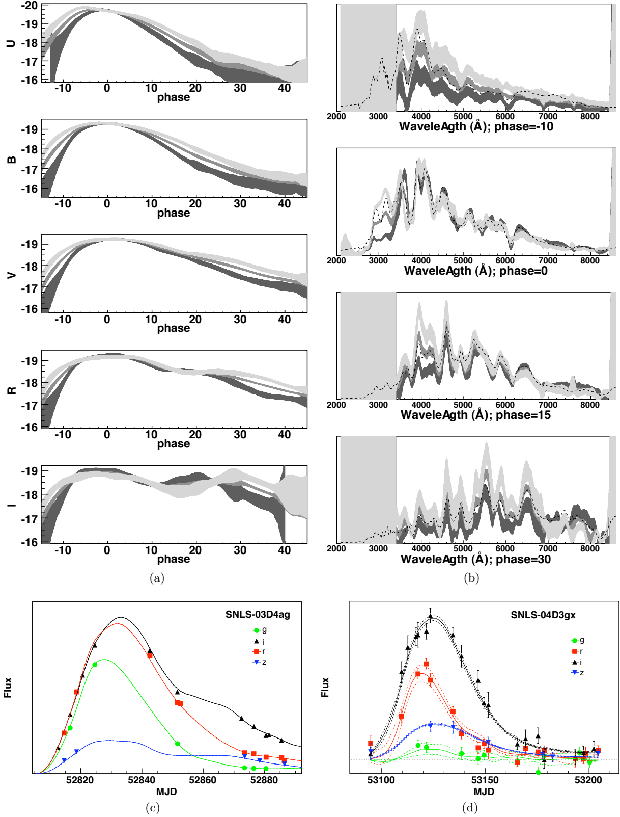
Figure 2.11: SALT2 models and results: (a) UBVRI template light curves for x_1 of -2,0,2 (dark to light curves); (b) template spectra for x_1 of -2,0,2 (dark to light curves), compared to Nugent et al. (2002) templates (dashed line); (c)–(d) photometric measurement points for SNLS’ SNe Ia at z = 0.285 and z = 0.91 respectively, and derived light curves from the SALT2 model. From Guy et al. (2007).
