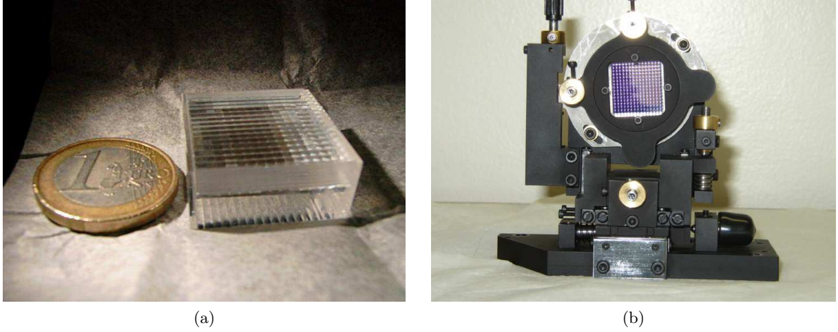
Figure 4.4: One microlens-array ( 21\text{mm} \times 21\text{mm} ) (a) next to an 1€ coin for scale; (b) in its support mount during assembly.
