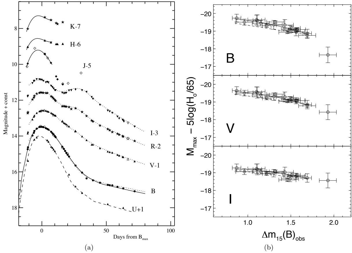
Figure 2.6: (a) Light curve in several bands (Johnson-Cousins UBVRI and near-infrared) from a typical SN Ia (SN2003du). Phase is with relation to B maximum. Adapted from Stanishev et al. (2007); (b) Brighter-slower correlation for SNe Ia light curves. Adapted from Phillips et al. (1999).
