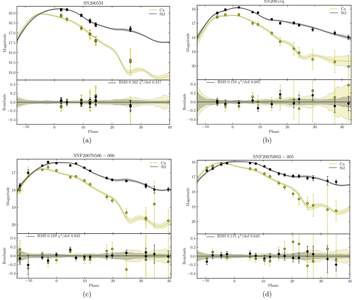
Figure 12.10: \mathcal{V} (Ca + Si2) sharp filter combination light curves for (a) SN2005M, (b) SN2007cq, (c) SNF20070506-006 and (d) SNF20070803-005.
