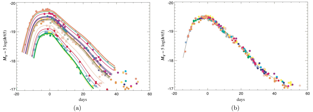
Figure 2.7: Cálan/Tololo nearby supernovæ absolute magnitudes in V band, (a) as observed and (b) after correction using the stretch parameter. Adapted from Perlmutter et al. (1997a).
