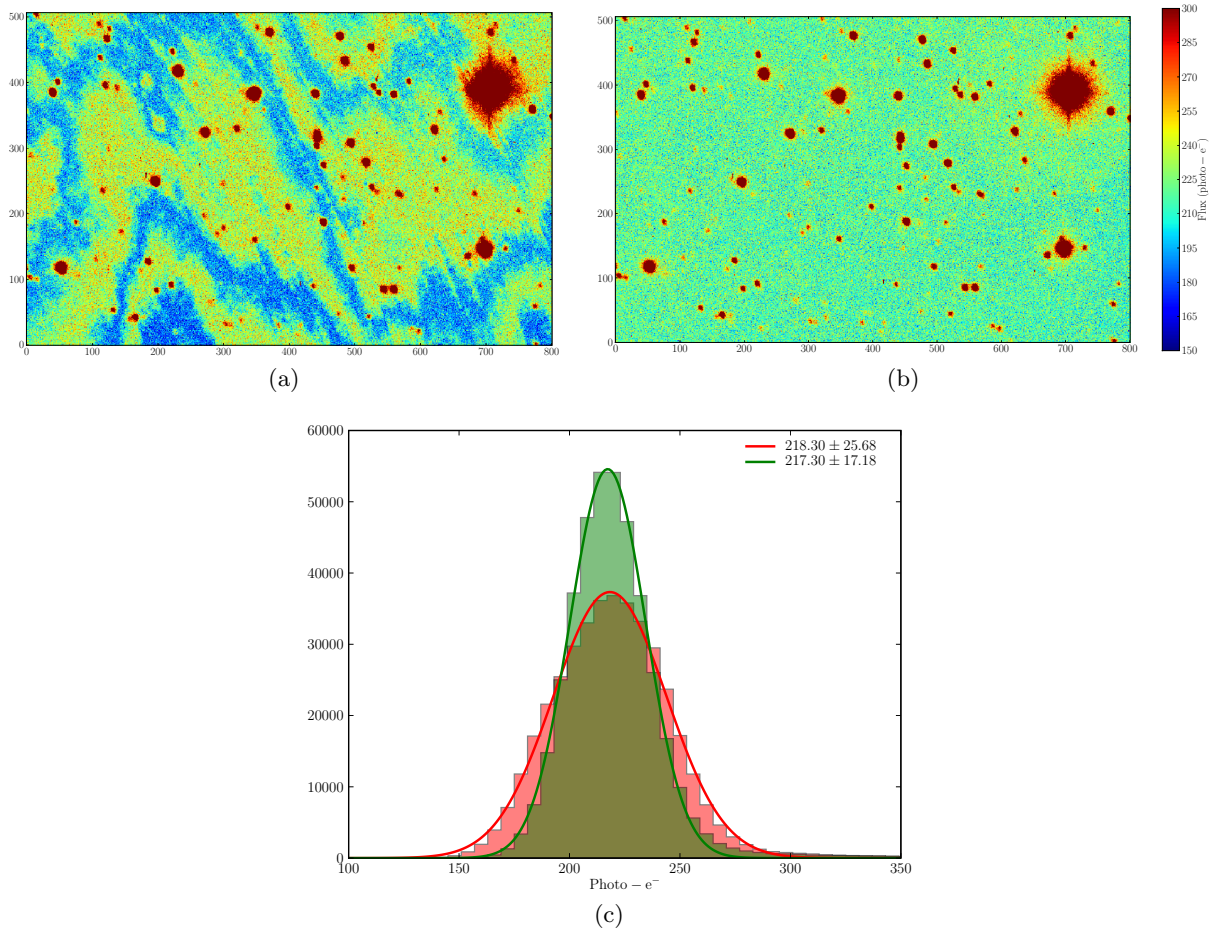
Figure 8.9: (a) F5 image of EG131, with visible fringes whose amplitude is \sim 25\% of the background value; (b) the same F5 exposure after defringing, showing a uniform background without the fringing spatial pattern; (c) Background pixel's distribution before (red) and after defringing (green). Notice the reduced RMS (up to near poissonian noise levels), after the removal of the fringes.
