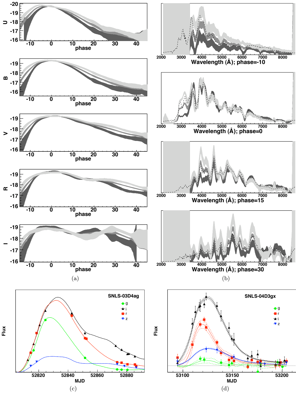
Figure 2.11: SALT2 models and results: (a) UBVRI template light curves for x_1 of -2, 0, 2 (dark to light curves); (b) template spectra for x_1 of -2, 0, 2 (dark to light curves), compared to Nugent et al. (2002) templates (dashed line); (c)–(d) photometric measurement points for SNLS’ SNe Ia at z = 0.285 and z = 0.91 respectively, and derived light curves from the SALT2 model. From Guy et al. (2007).
