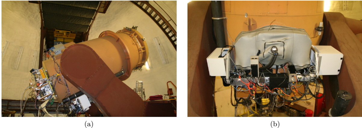
Figure 4.1: (a) University of Hawaii 2.2m (UH88) telescope; (b) SNIFS mounted on the bent-Cassegrain port of UH88. The main instrument is in the center under the neoprene cover, used to isolate it from external light and keep the internal temperature and humidity from large changes, besides all the support electronics.
