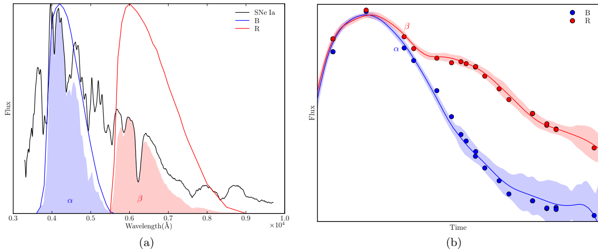
Figure 3.1: Spectrophotometry concept: (a) by convolving any filter (here Bessell B and R are shown) with each flux calibrated spectrum from a SNe Ia temporal sequence, we can obtain (b) the corresponding light curve points for that filter, without any \mathcal{K} -corrections involved. The light curve line fitted using SALT2 is given for reference.
