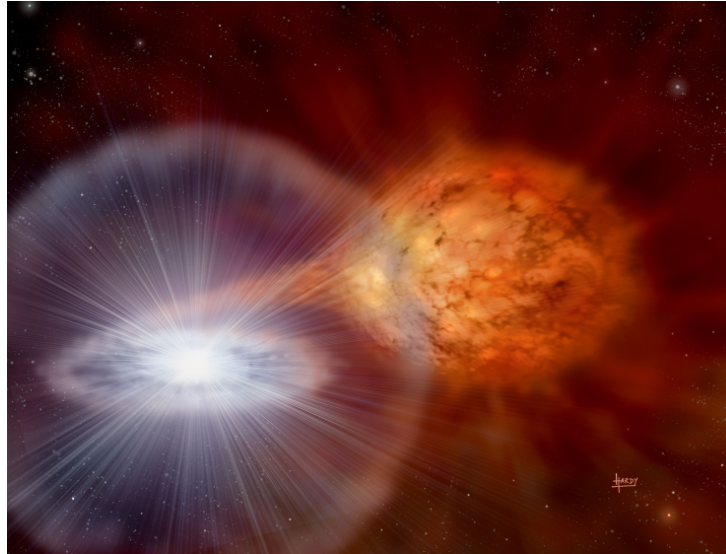
Figure 2.5: Artist impression of a SNe Ia caused by the explosion of a WD accreting matter in a binary system. By D. Hardy ( http://www.astroart.org ).
