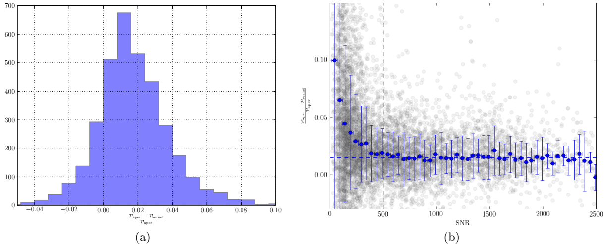
Figure 9.10: (a) Distribution of the normalized difference between photometric ratios for \sim 3500 exposures with SNR > 500. (b) Median normalized difference between photometric ratios and respective nMAD per SNR bin of 50. The vertical dashed line corresponds to the chosen SNR threshold, and the horizontal one to the median normalized difference above this threshold, 0.015.
