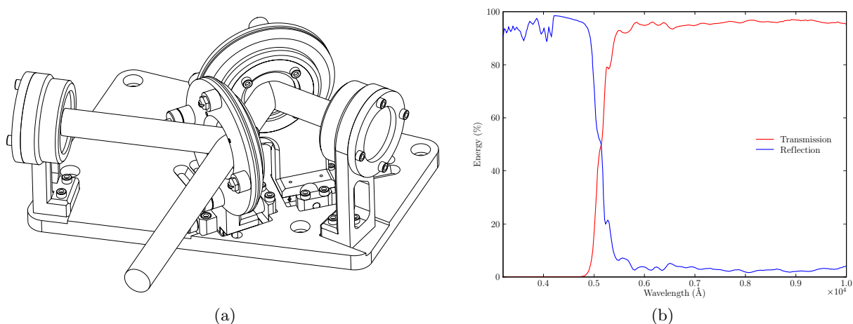
Figure 4.3: (a) Spatial stage schematic. The dichroic is visible at the lower center, and splits the entrance beam for the blue (left) and red (right) spectrographs; (b) Dichroic transmission for the blue and red wavelengths.
