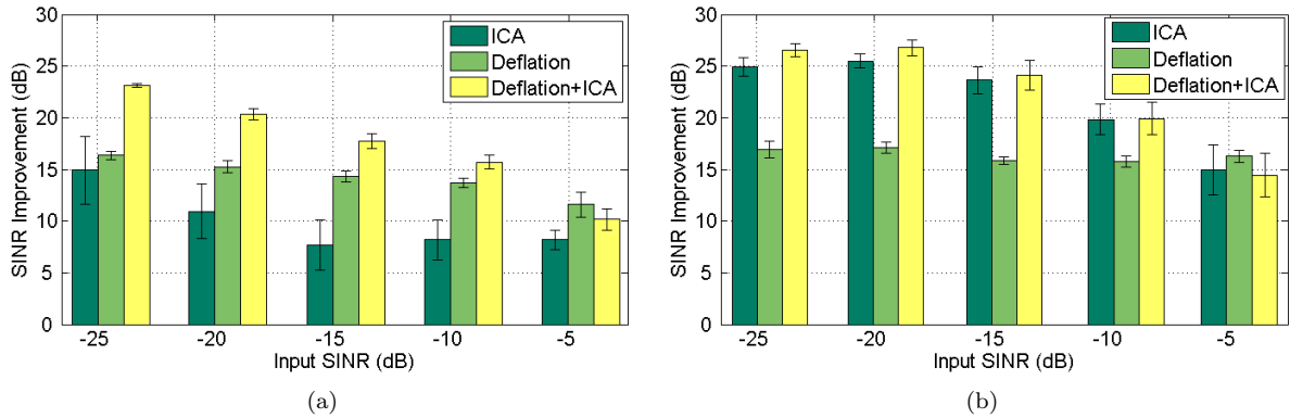
Figure 8.5: The mean and standard deviation bar of SINR improvements achieved in different input SINRs for (a) \theta_{mf} < 10^\circ (b) \theta_{mf} > 60^\circ
