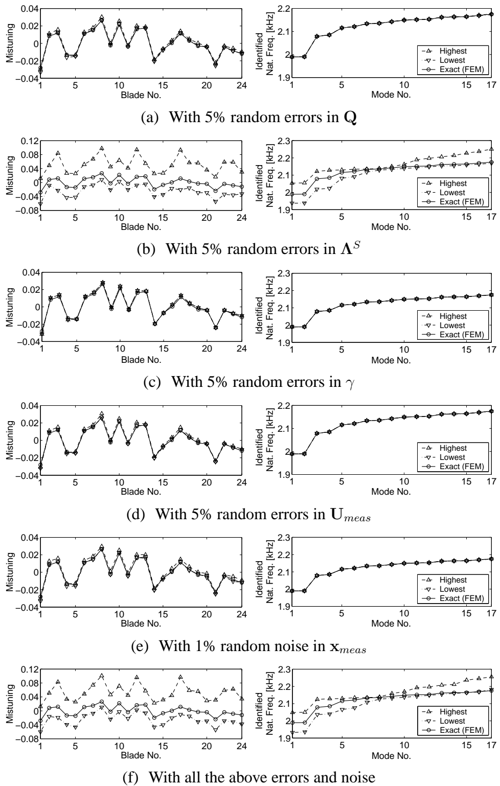
Figure 3.6: Sensitivity of identification results to errors in model parameters and measured data.
