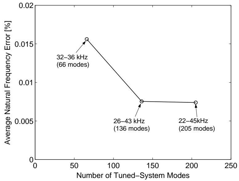
Figure 2.4: Convergence of average natural frequency error for the large mistuning case.
