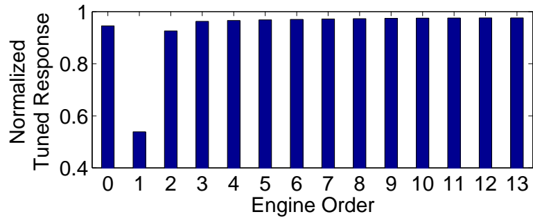
(b) Normalized tuned-system forced response at resonant frequencies
