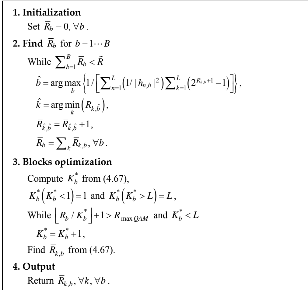
Figure 4.7: Mean BER minimization algorithm with variable constellation orders for LP-OFDM systems using a constant spreading code length.
