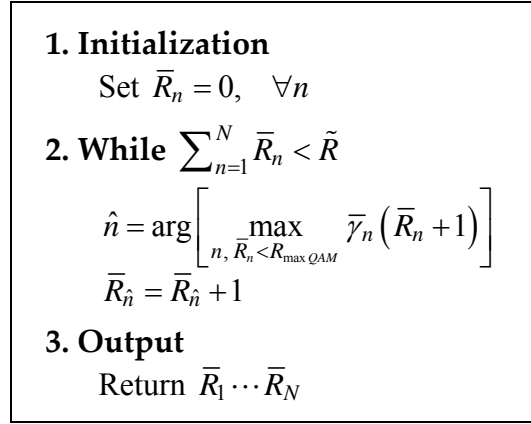
Figure 3.2: Margin maximization algorithm with integer bit allocation for OFDM systems.
