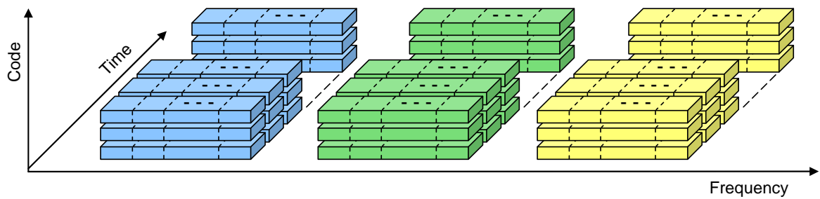
(c) F-CDM & TDM / FDMA (SS-MC-MA)
