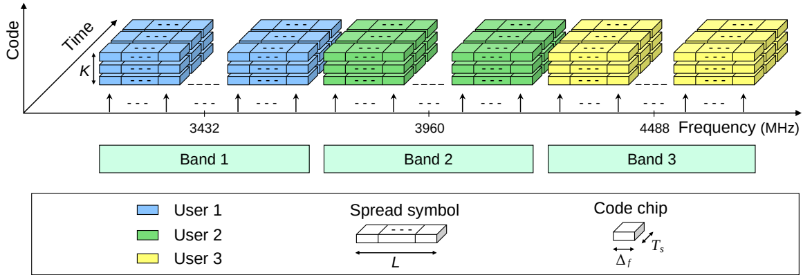
Figure 2.10: LP-OFDM schematic representation for three users occupying the first three bands of the MB-OFDM scheme.
