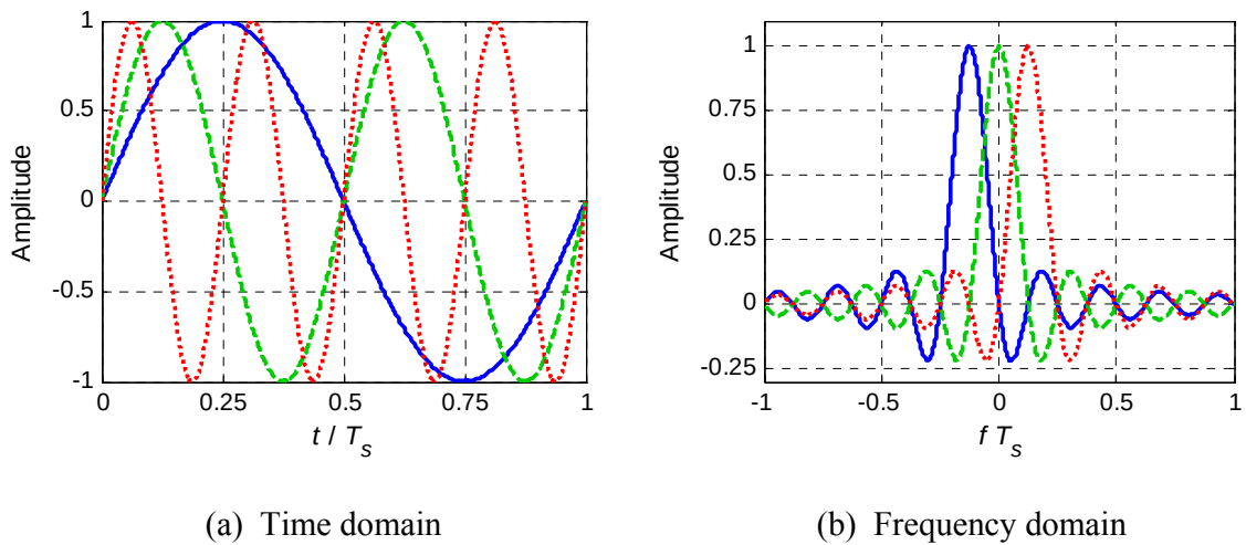
Figure 2.1: Example of three subcarriers within an OFDM symbol.
