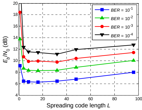
(a) E_b/N_0 variation with r = 3/4
