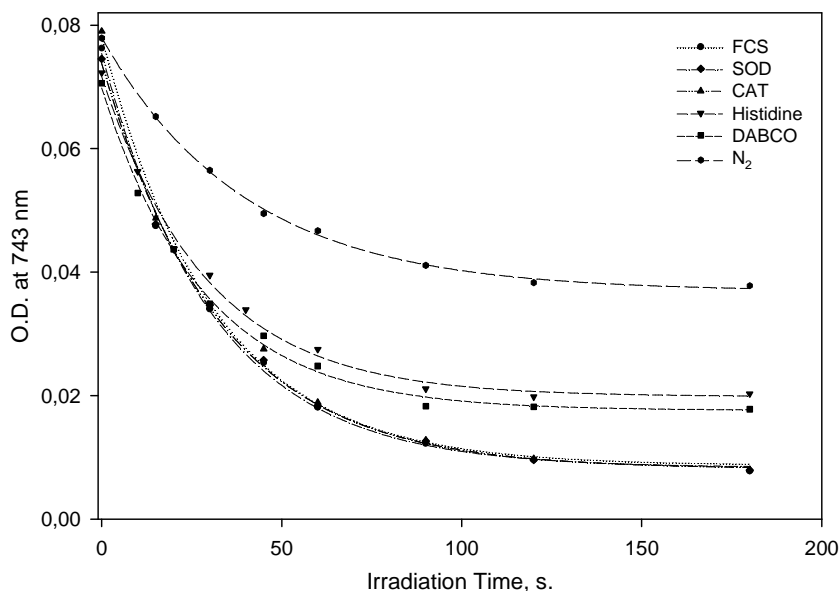
Figure 3.4. Effect of \text{N}_2 , antioxidant enzyme and singlet oxygen quenchers on the photobleaching of m-THPC in PBS solution supplemented with 10% FCS. Histidine and DABCO were added to a final concentration of 10mM, SOD concentration was 40 \mu\text{g mL}^{-1} , and CAT concentration was 45 \mu\text{g mL}^{-1} . Bubbling with nitrogen runs during 30 min.
