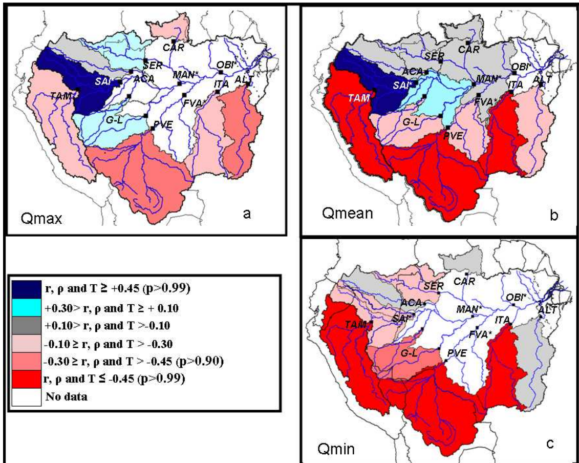
FIGURE 2.5 – Pearson ( r ), Spearman rho ( \rho ) and Kendall Tau ( T ) coefficients between runoff and time (1974-2004) in the sub-basin of the Amazon for a) the annual maximum values (Qmax), b) the mean annual values (Qmean), c) the minimum values (Qmin). Values above 0.30 are significant at the 90% level and above 0.45 at the 99% level. The colors indicate the sign and the strength of the trend : red is for negative trend and dark blue is for positive trend.
