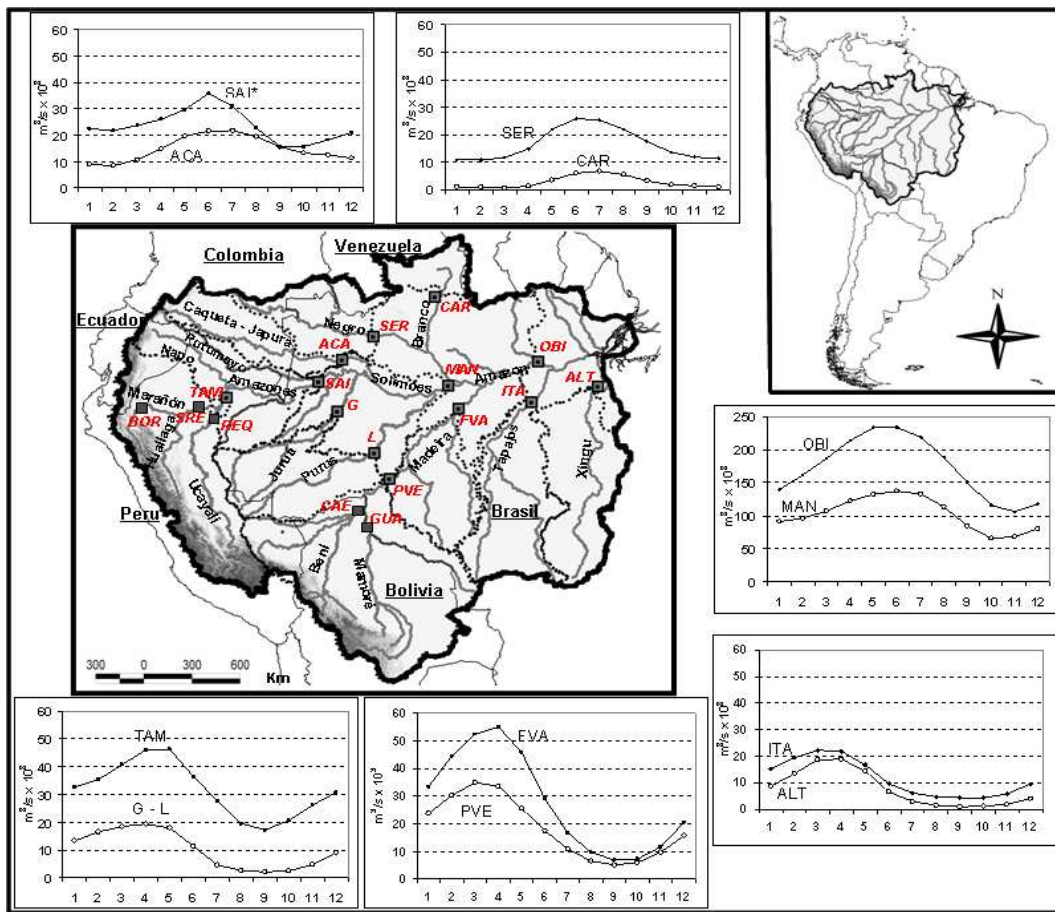
FIGURE 2.1 – Localization of the main sub-basins and hydrological stations of the Amazon Basin. The 1974-2004 mean monthly discharge ( m^3/s \times 10^3 ) is presented for each sub-basin. G–L data is the sum of Gavião and Labréa stations data. Altamira and Itaituba sub-basins, on the Xingu and Tapajós Rivers respectively, are not part of the Amazon basin in Óbidos. The X axis is from 1 for January to 12 for December. Andean mountainous regions are shaded.
