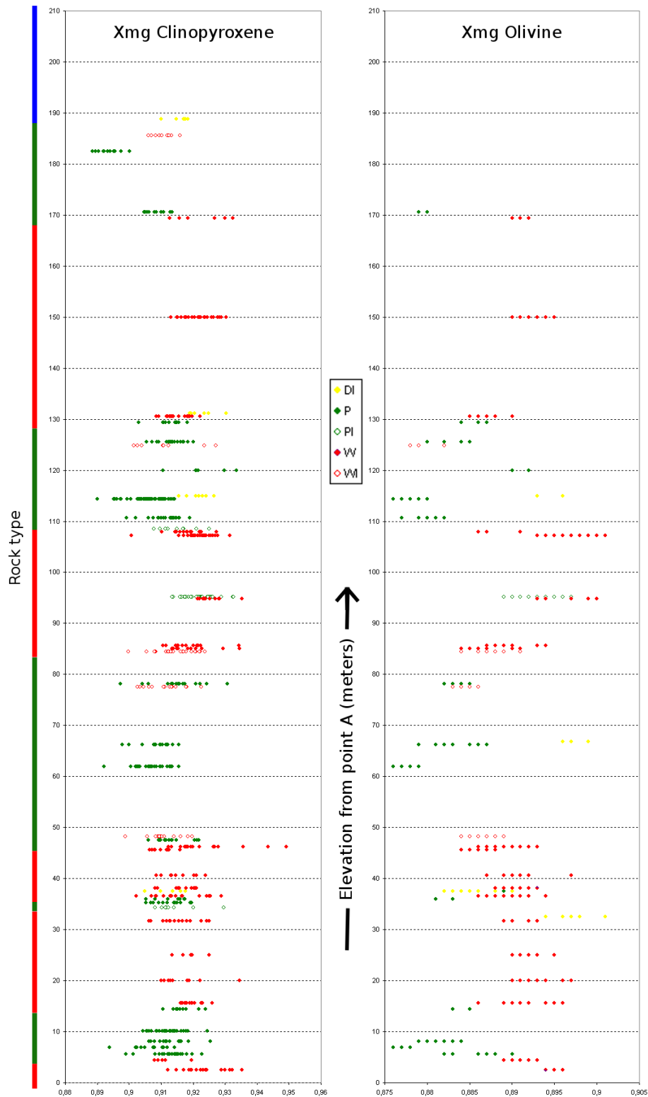
FIG. 7.41 – Stratigraphic variations of Mg# [100 x Mg/(Mg+Fetot)] in cpx (left) and olivine (right) from the southern outcrop. The color scale on the left shows dominant rock types (green : clinopyroxenite ; red : wehrlite ; blue : gabbro).
