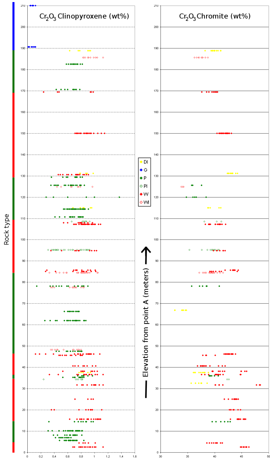
FIG. 7.42 – Stratigraphic variations of Cr 2 O 3 (wt%) in cpx (left) and Cr-spinel from the southern outcrop.
