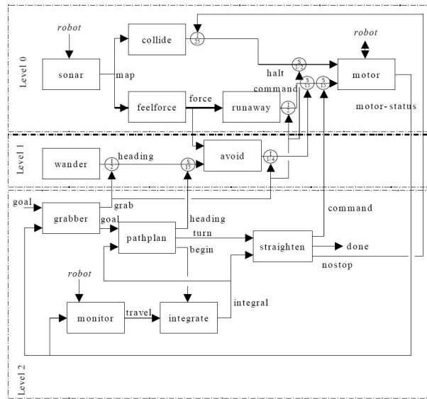
FIG. 2.4 – Architecture subsumption [20]
