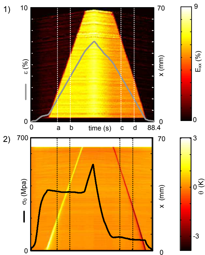
Figure 4.33: Tensile test T3_2 . 1) Temporal evolution of an axial profile of the Green-Lagrange strain E_{xx}(M,t) (colored map) superimposed with the sample deformation \varepsilon (curve). 2) Temporal evolution representation of the axial temperature variation \theta(M,t) (colored map) superimposed with the nominal stress curve.
