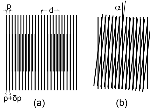
Figure 2.2: Examples of moiré pattern for two sets of parallel lines. a) The two sets are parallel and the first set has a grid step of length p , the second set p + \delta p . b) The two sets have the same grid step p , one is inclined by a small angle with the other.
