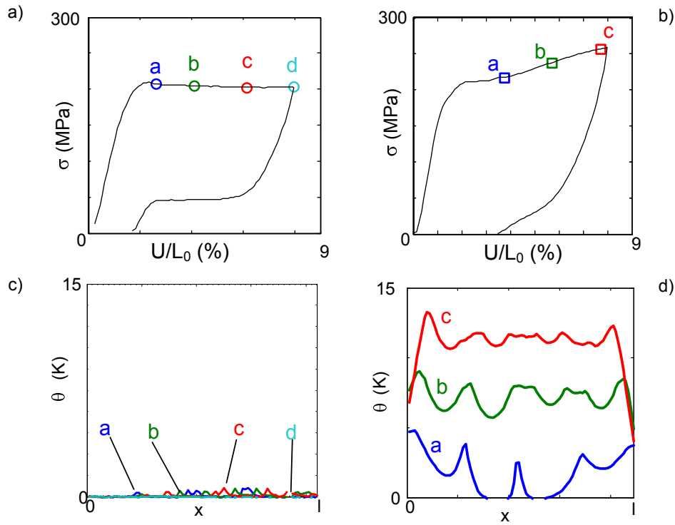
Figure 3.8: Thermo-mechanical response of tensile tests performed at \dot{\varepsilon}_0 = 2 \cdot 10^{-3} \text{ s}^{-1} with (left) and without (right) the temperature control system. a,b) Stress-strain curves. c,d) Temperature variation along the length of the sample.
