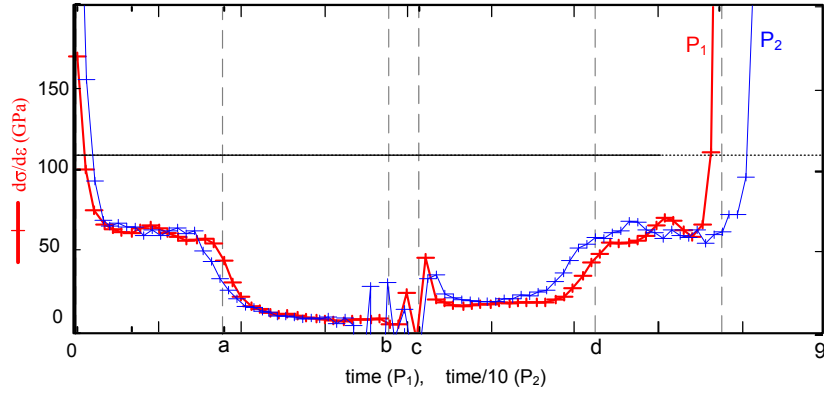
Figure 5.7: Evolution of the ratio d\sigma/d\varepsilon . The term d\varepsilon is the time derivative of the local axial strain \varepsilon = \Delta l/l_0 estimated from relative displacements of the two extreme points of the correlation area A and B . The markers represent the time of visible image acquisition. To be able to compare the two curves, the time has been normalised by the strain rate.
