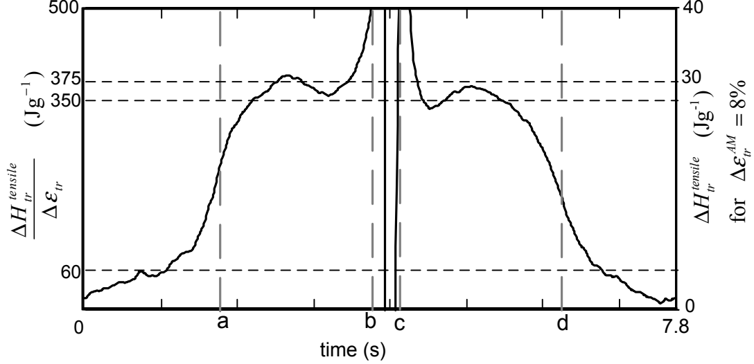
Figure 5.12: Test P_1 . Time evolution of \Delta H_{tr}^{tensile} / \Delta \varepsilon_{tr} (left axis) and \Delta H_{tr}^{tensile} (right axis) when taking \Delta \varepsilon_{tr} = \Delta \varepsilon_{tr}^{AM} = 8\% .
