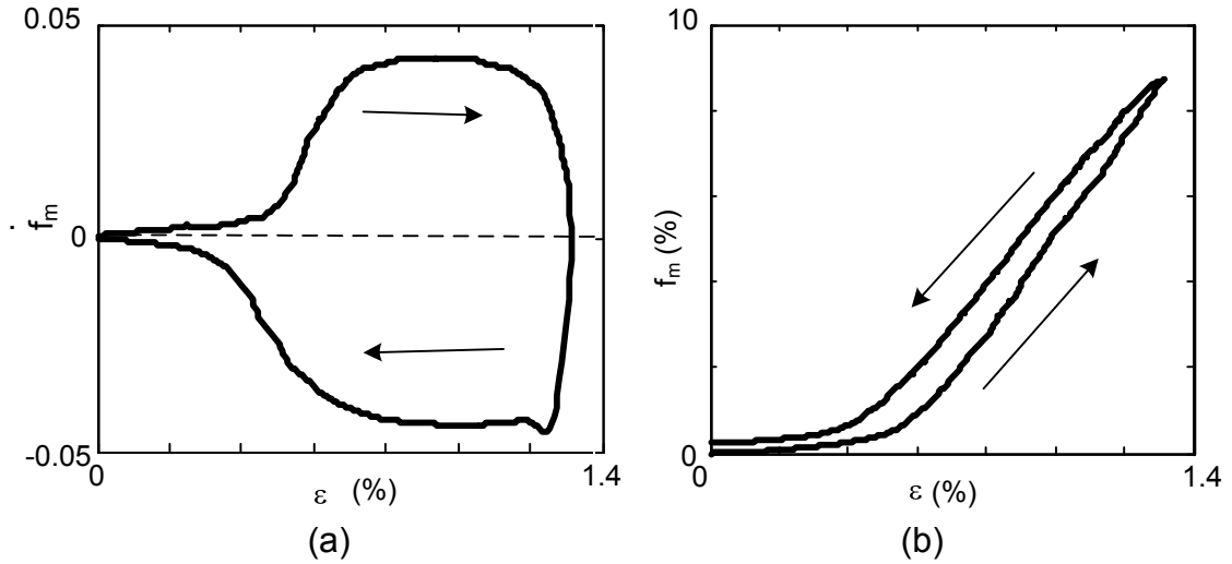
Figure 5.14: Martensite fraction estimated during test P_1 . a) f_m evolution as a function of strain. b) Martensite fraction f_m as a function of strain.
