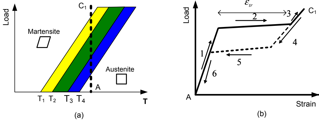
Figure 1.4: a) Load-temperature SMAs phase diagram. b) Simplified superelastic SMAs strain-stress curve corresponding to the path A \rightarrow C_1 \rightarrow A plotted in (a). Conventional understanding: (1) elastic deformation of austenite; (2) austenite to oriented martensite transformation; (3) and (4) elastic deformation of oriented martensite. (5) Oriented martensite to austenite reverse transformation; (6) elastic deformation of austenite.
