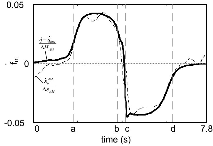
Figure 5.13: Test P_1 . Comparison of the martensite fraction estimated from the phase transformation strain rate ( \dot{f}_m = \dot{\epsilon}_{tr}^{AM} / \Delta \epsilon_{AM} ) and from the phase transformation heat sources ( \dot{f}_m = \dot{q}_{tr} / \Delta H_{AM} ) with \Delta H_{AM} = 30 \text{ J g}^{-1} .
