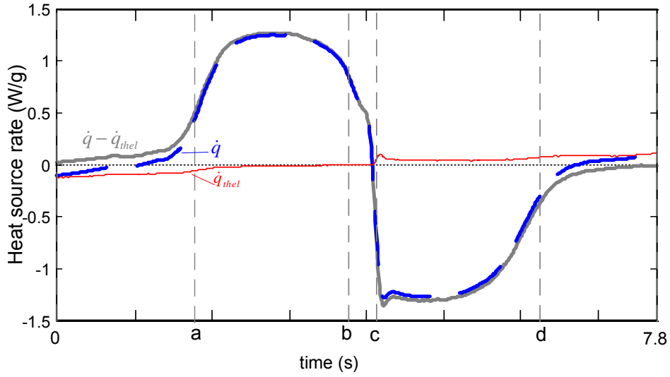
Figure 5.10: Test P_1 . Time evolution of the estimated heat source rate \dot{q} (dashed thick line), \dot{q}_{thel} the heat sources due to the thermoelastic coupling (red thin line), the remaining heat source rate ( \dot{q} - \dot{q}_{thel} ) (grey thick solid line).
