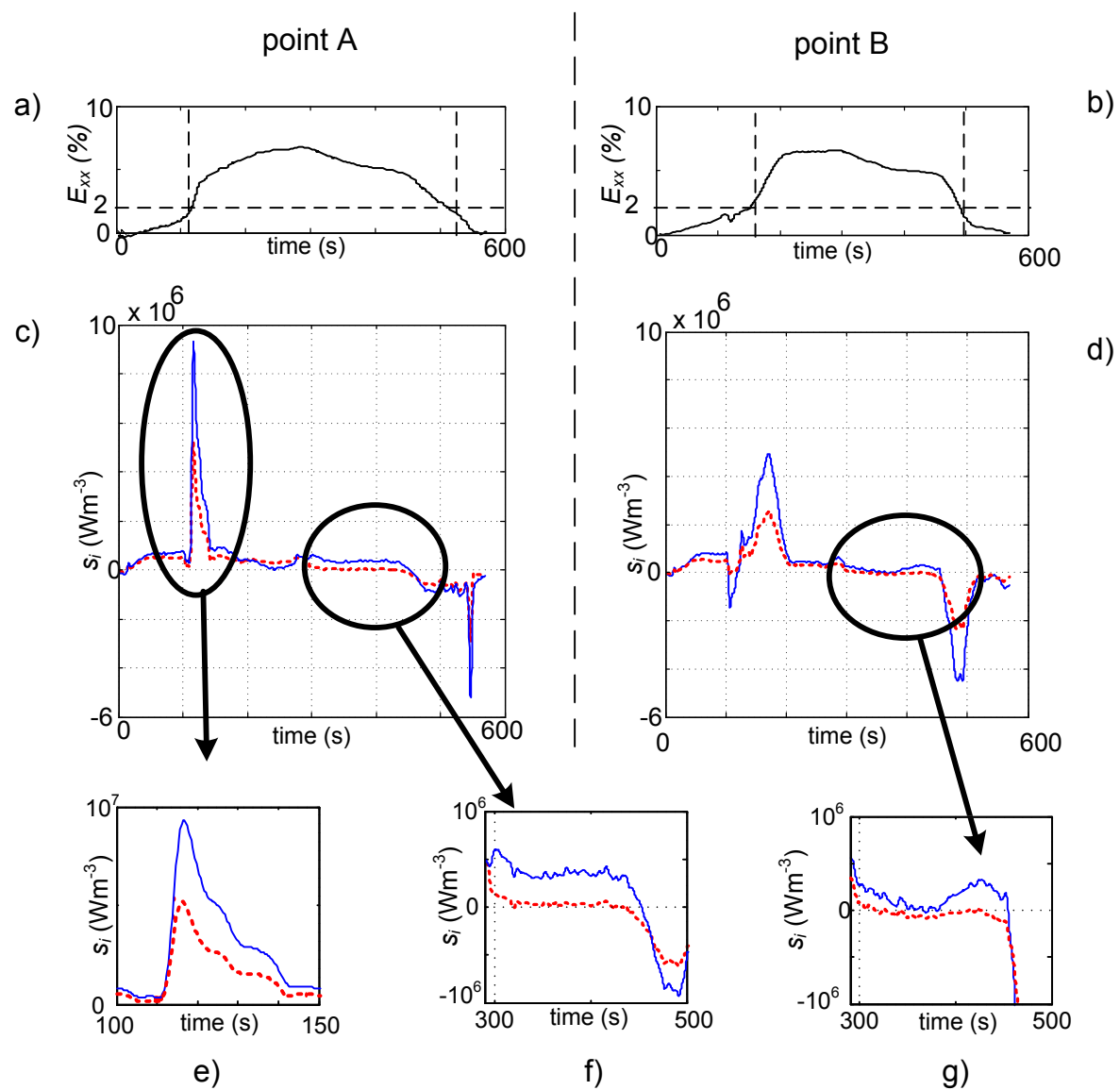
Figure 6.7: Influence of the thermal conductivity coefficient k on the heat source estimation for two points A and B (see Figure 6.3 time b). a-b) Temporal evolution of the Green Lagrange axial strain E_{xx}(A) and E_{xx}(B) . c-g) Temporal evolution of the heat source estimation using k = k_A (solid line) and k = k_M (dashed line).
