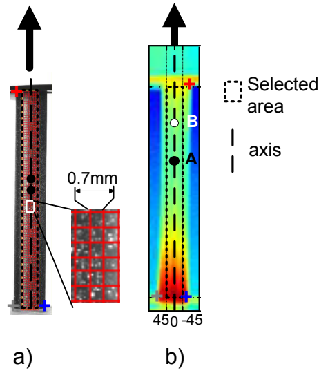
Figure 6.1: a) Visible photography of tube T2_1 with the image correlation grid. b) Infrared image of the same tube and position of the selected area used to estimate the heat sources. The “+” shows the position of the characteristic points used to estimate the transformation matrix and perform the spatial synchronisation. The vertical dashed axis is the position of the tube axis.
