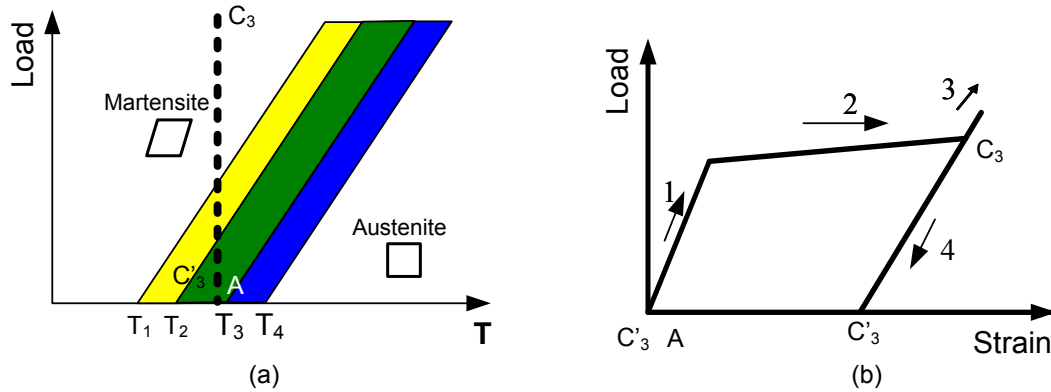
Figure 1.6: a) Load-temperature SMAs phase diagram. b) Simplified SMAs strain-stress curve corresponding to the path A_3 \rightarrow C_3 \rightarrow C'_3 plot in (a).
