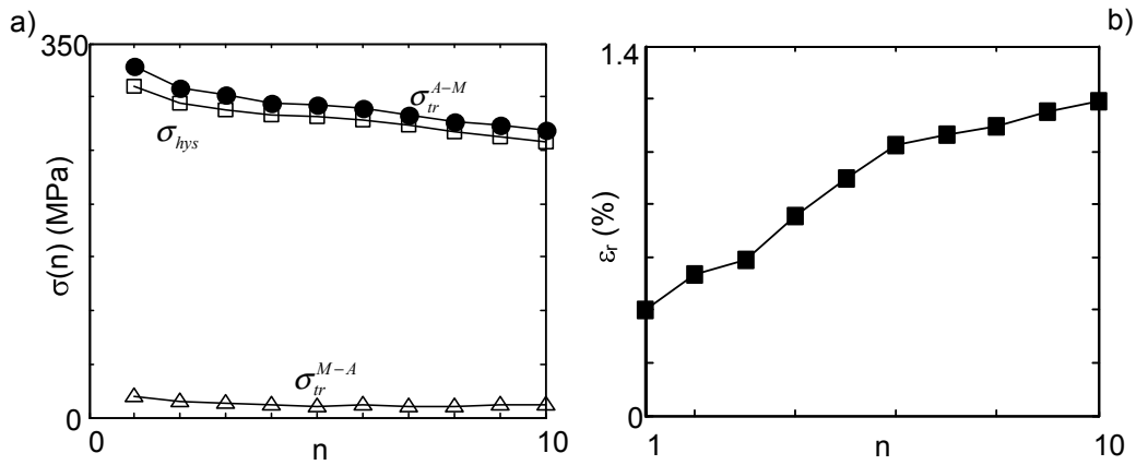
Figure 4.27: a) Evolution with the number of cycle n , of the stress plateau measured during loading \sigma_{tr}^{A-M} and unloading \sigma_{tr}^{M-A} respectively at \varepsilon_0 = 2\% and \varepsilon_0 = 4\% and the stress hysteresis \sigma_{hys} . b) Evolution of the residual strain \varepsilon_r at the end of loading.
