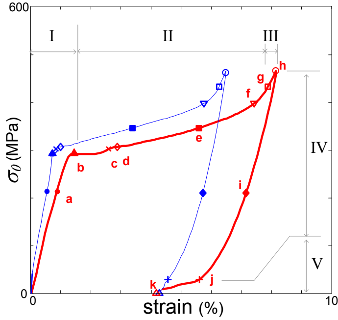
Figure 4.2: Nominal stress \sigma_0 vs. global axial strain \varepsilon_{L_0} (thin curve) and average axial strain \varepsilon_{l_0} (thick curve). \varepsilon_{L_0} is determined from the cross-head displacement U and the sample gauge length L_0 . \varepsilon_{l_0} is determined from the optical measurements of the displacements of the two points A and B in Figure 4.1.c. Markers and letters a to k indicate selected times in Figures 4.3 to 4.7.
