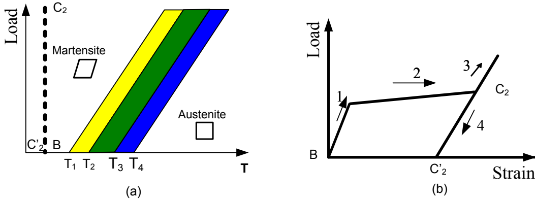
Figure 1.5: a) Load-temperature SMAs phase diagram. b) Simplified SMAs strain-stress curve corresponding to the path B \rightarrow C_2 \rightarrow C'_2 plot in (a).
