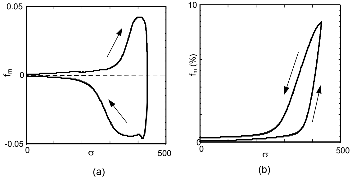
Figure 5.15: Martensite fraction estimated during test P_1 . a) \dot{f} evolution as a function of nominal stress. b) Martensite fraction f as a function of nominal stress.
