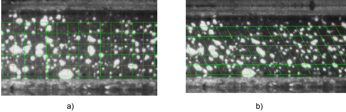
Figure 2.5: Example of images correlation grid prior (a) and after deformation (b) during a shear test.
