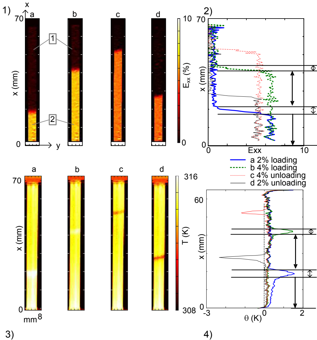
Figure 4.32: Tensile test T3_2 ( \dot{U}/L_0 = 2.10^{-3} s^{-1} , T_{fluid} = 315 K). Colored maps (1) and profiles (2) of the axial Green-Lagrange strain E_{xx} and the temperature at times a, b, c, d, (respectively \varepsilon = 2\% , 4\% during loading and then 4\% and 2\% during unloading (see Figure 4.30)). 3) Temperature fields T on the outer surface at the same time. 4) Temperature variations profile \theta along the same profile as E_{xx} .
