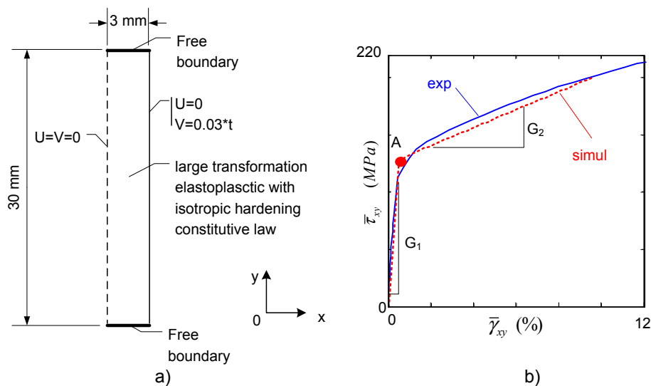
Figure 3.19: Simulation of the simple shear test. a) Geometry and boundary conditions. b) Mechanical response of the feasibility test obtained in the experiment (continuous blue line) and numerical model (dotted line), with its coefficients.
