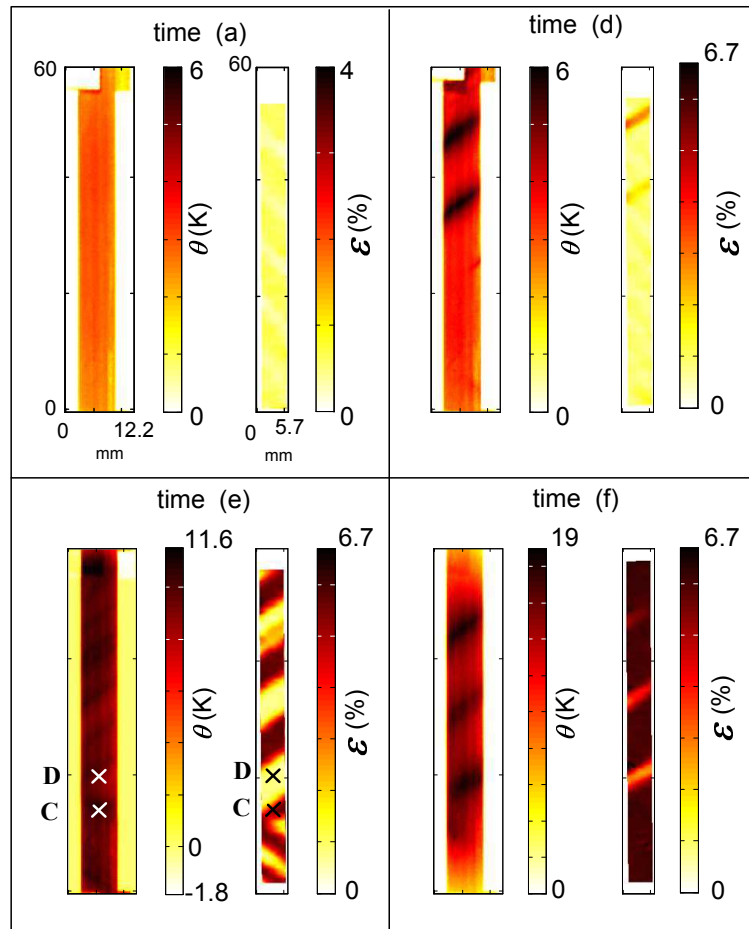
Figure 4.3: Coloured maps showing the temperature variation \theta(M) (left) and the local strain \epsilon(M) (right) fields on the surface of the deformed tube at four selected times marked in Figure 4.2.
