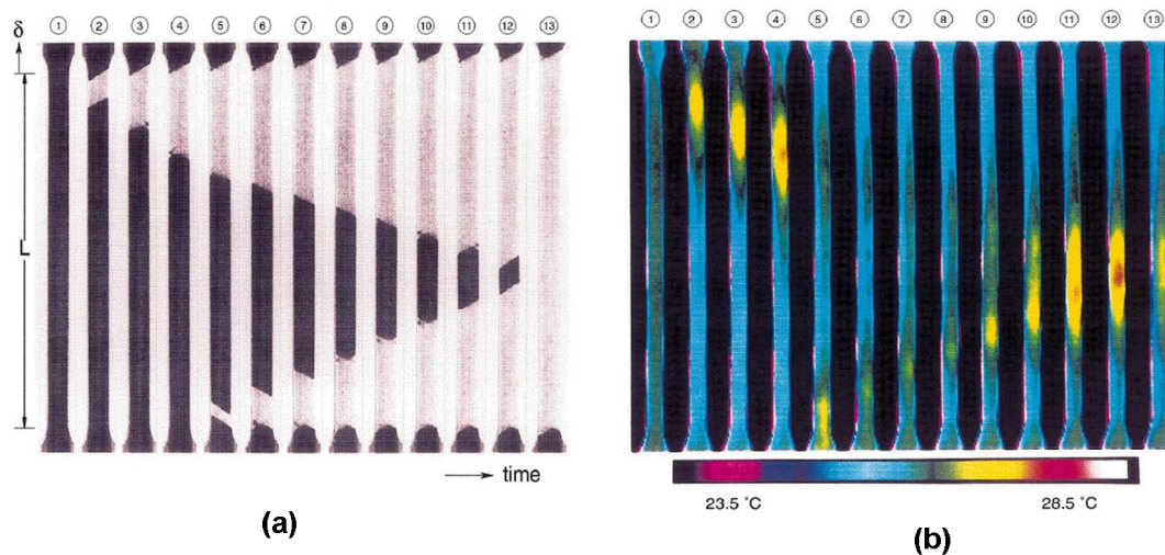
Figure 1.13: Observation of localised A \rightarrow M phase transformation during a tensile test, performed at \dot{\delta}_f/L = 10^{-4}\text{ s}^{-1} at ambient temperature, by taking a) visible photo and b) temperature fields measured by an infrared camera (Shaw and Kyriakides, 1997).
