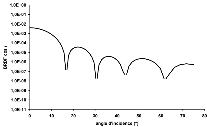
Figure 120 : r = 5 \cdot 424 = 2119 \text{ nm} et h = 100 \text{ nm}
