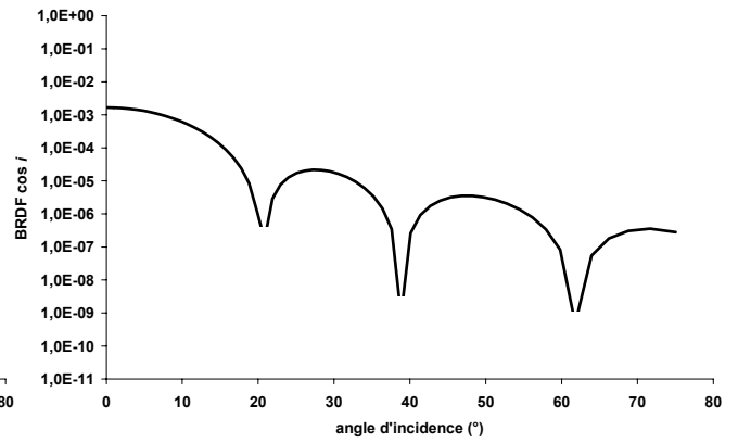
Figure 122 : r = 4 \cdot 424 = 1695 \text{ nm} et h = 100 \text{ nm}
