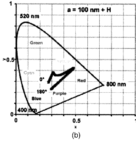
Fig. 10. Chromaticity diagram of a 100 nm radius silica sphere covered with an H layer (a) for diffuse scattering by reflection and transmission and (b) for each scattering angle \theta .
