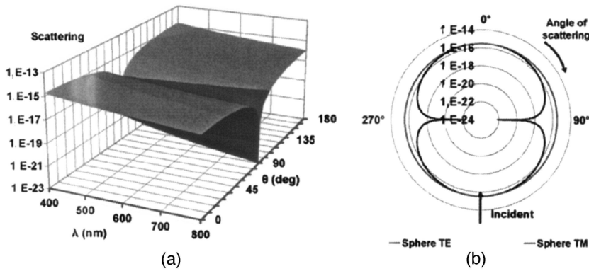
Fig. 1. (a) Angular scattering and (b) polar diagram at \lambda = 633 nm of a 10 nm radius silica sphere.
