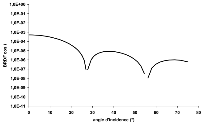
Figure 119 : r = 3 \cdot 424 = 1272 \text{ nm} et h = 100 \text{ nm}
