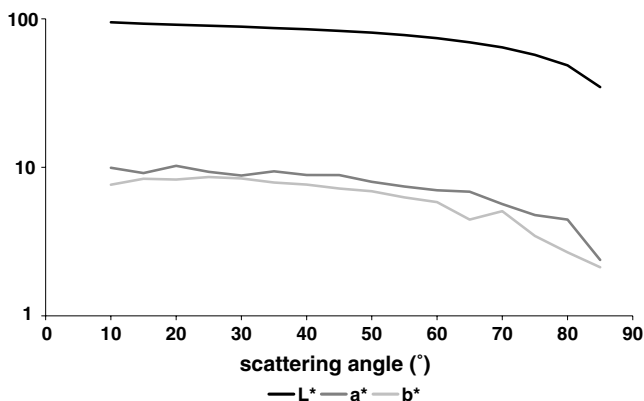
Fig. 4. L^* , a^* , b^* coordinates for a powder sample as a function of the scattering angle.
