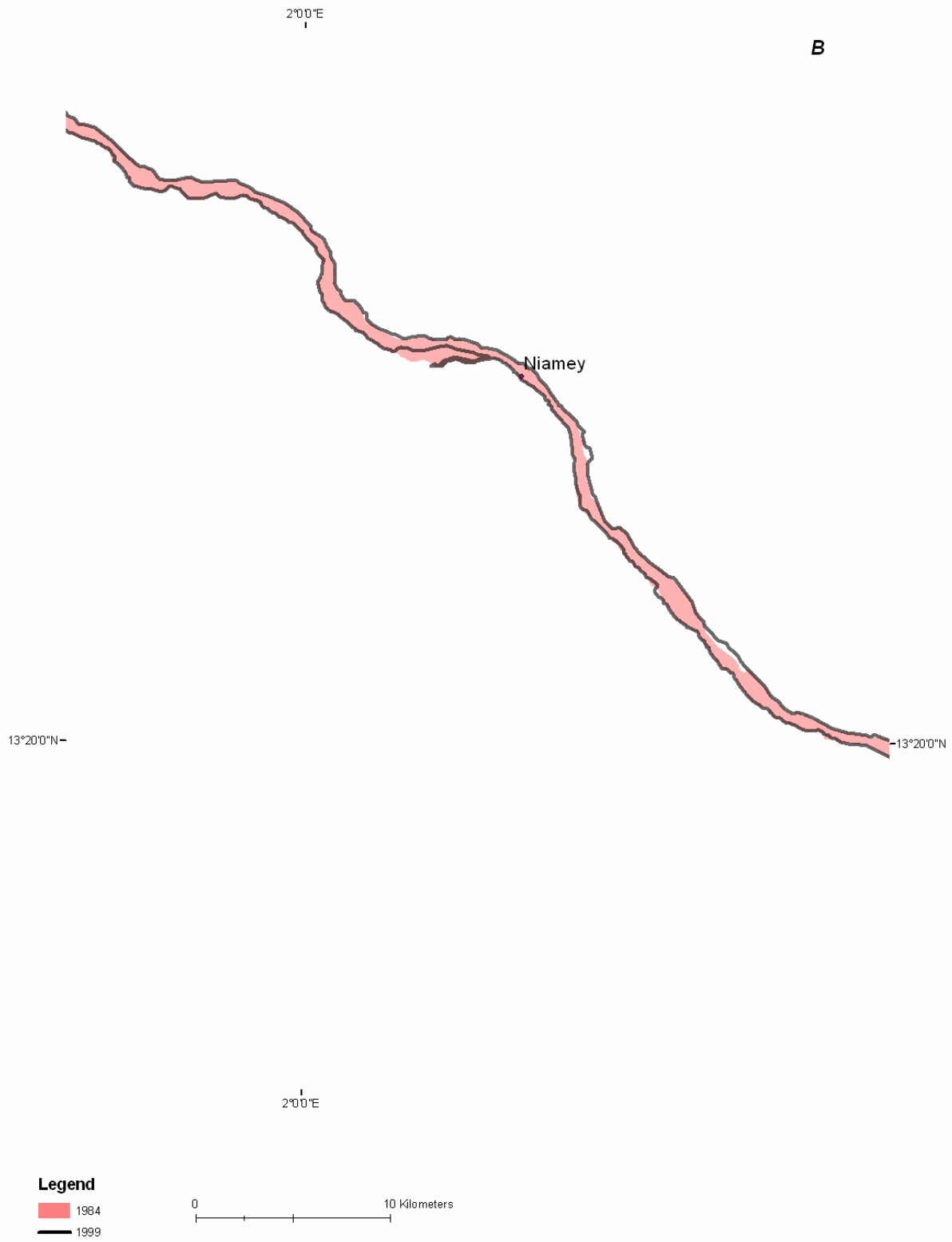
Figure B- 38B: Channel change in Reach 2 (1984-1999)
