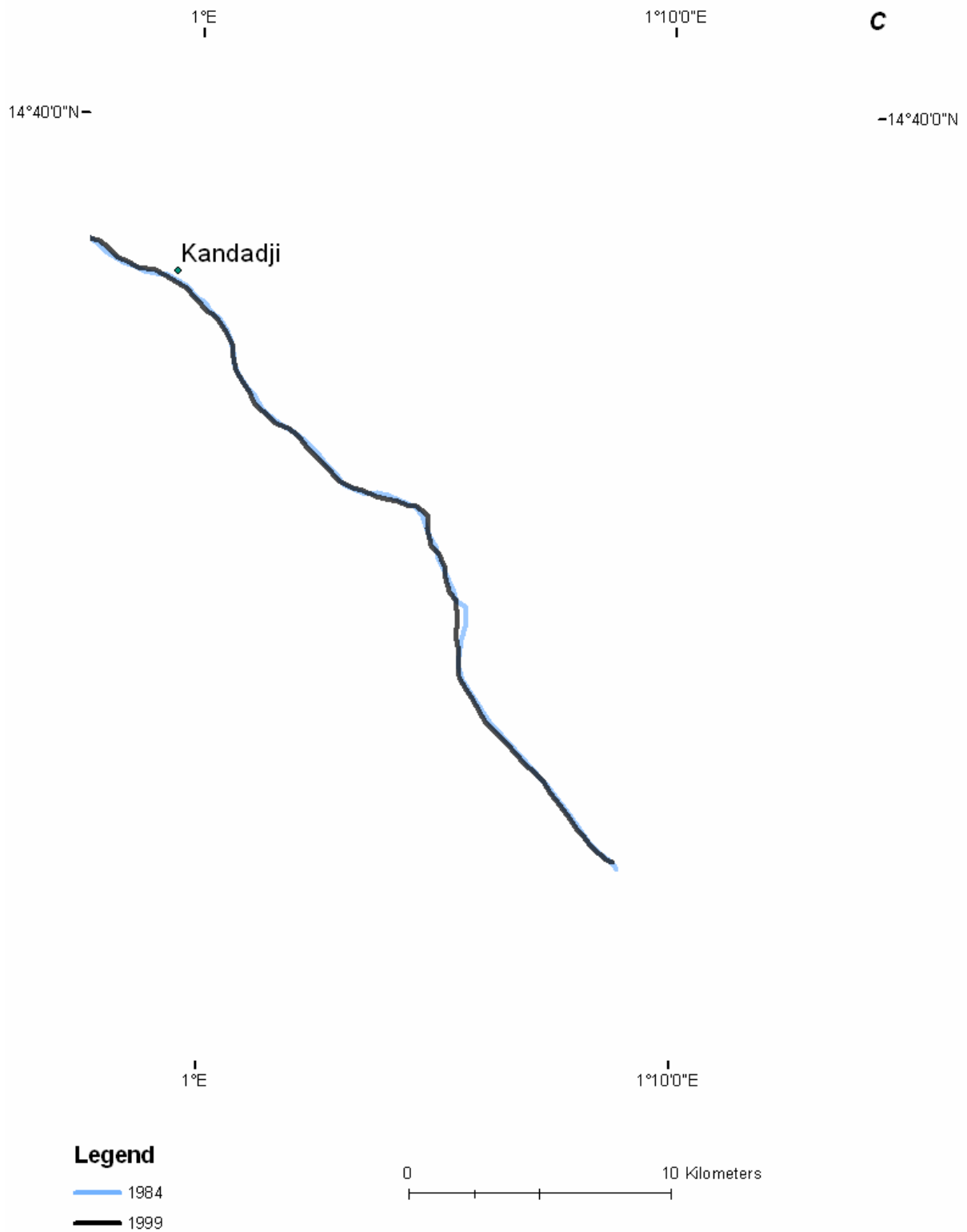
Figure B- 19C: River centre line change in reach 1 (1984 – 1999)
