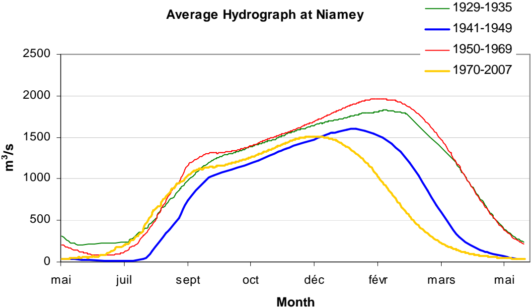
Figure IV- 14: Average hydrographs of the Niger River at Niamey
