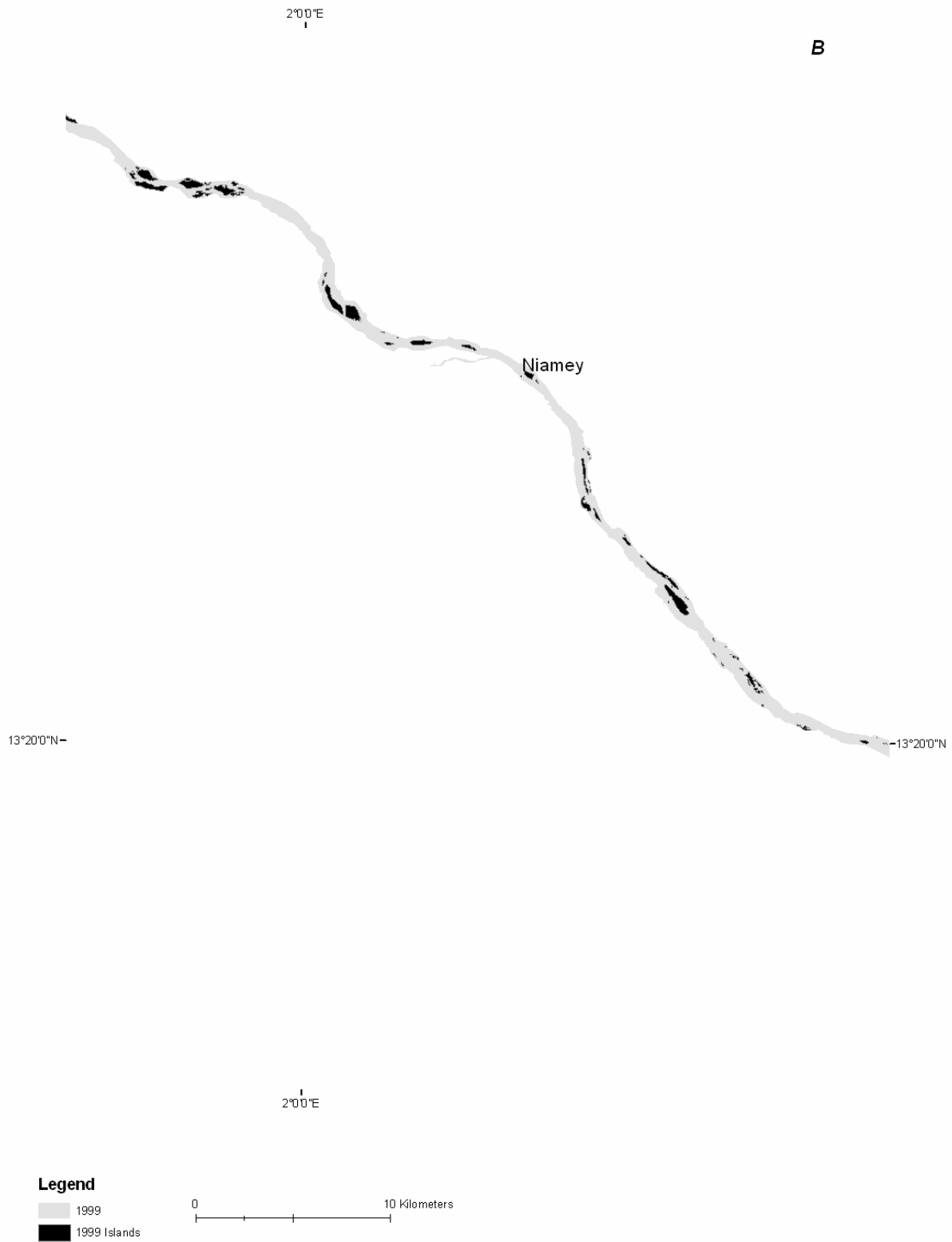
Figure B- 60B: Reach 2 channel bank and island extents in 1999
