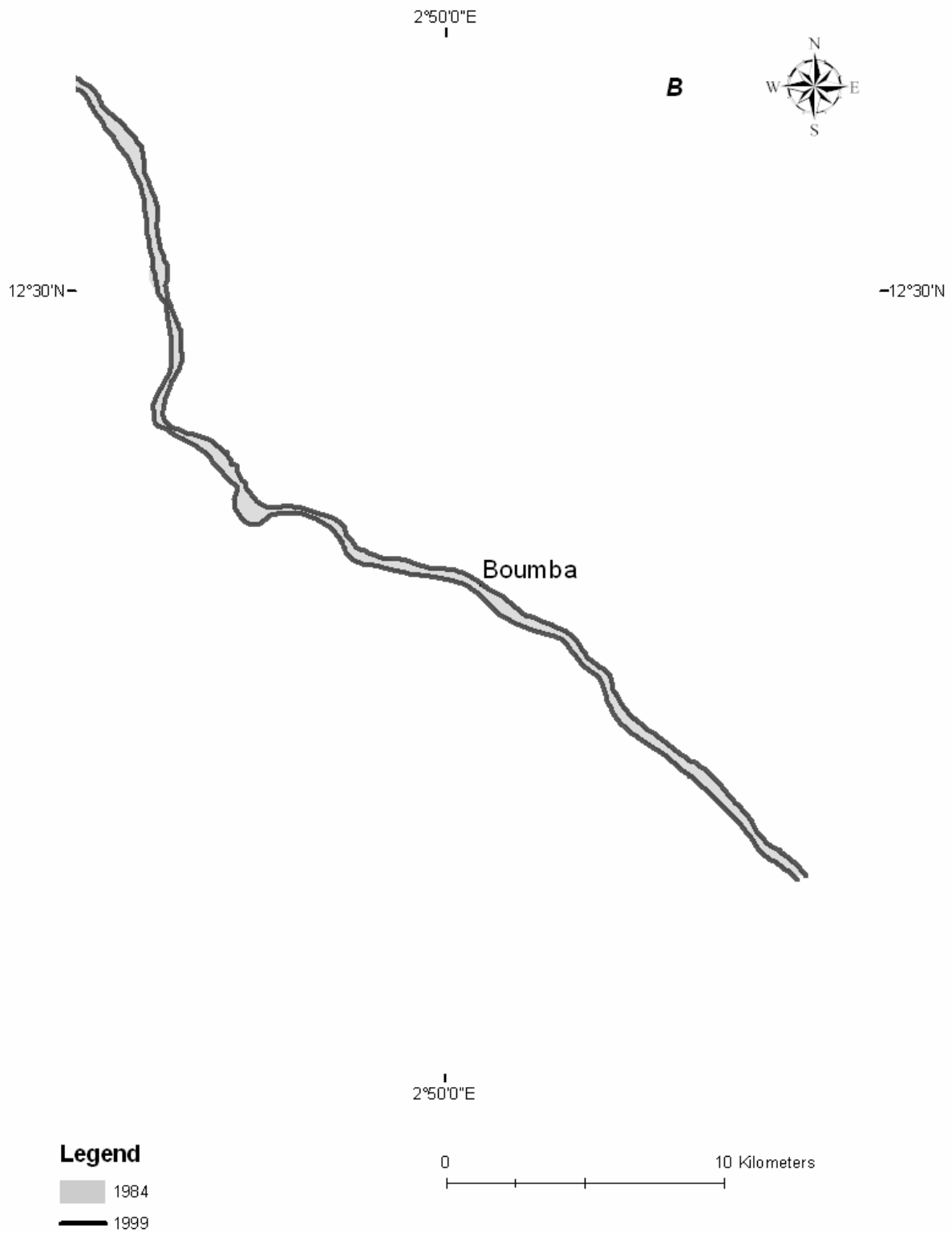
Figure B- 77B: Channel change in Reach 3 (1984-1999)
