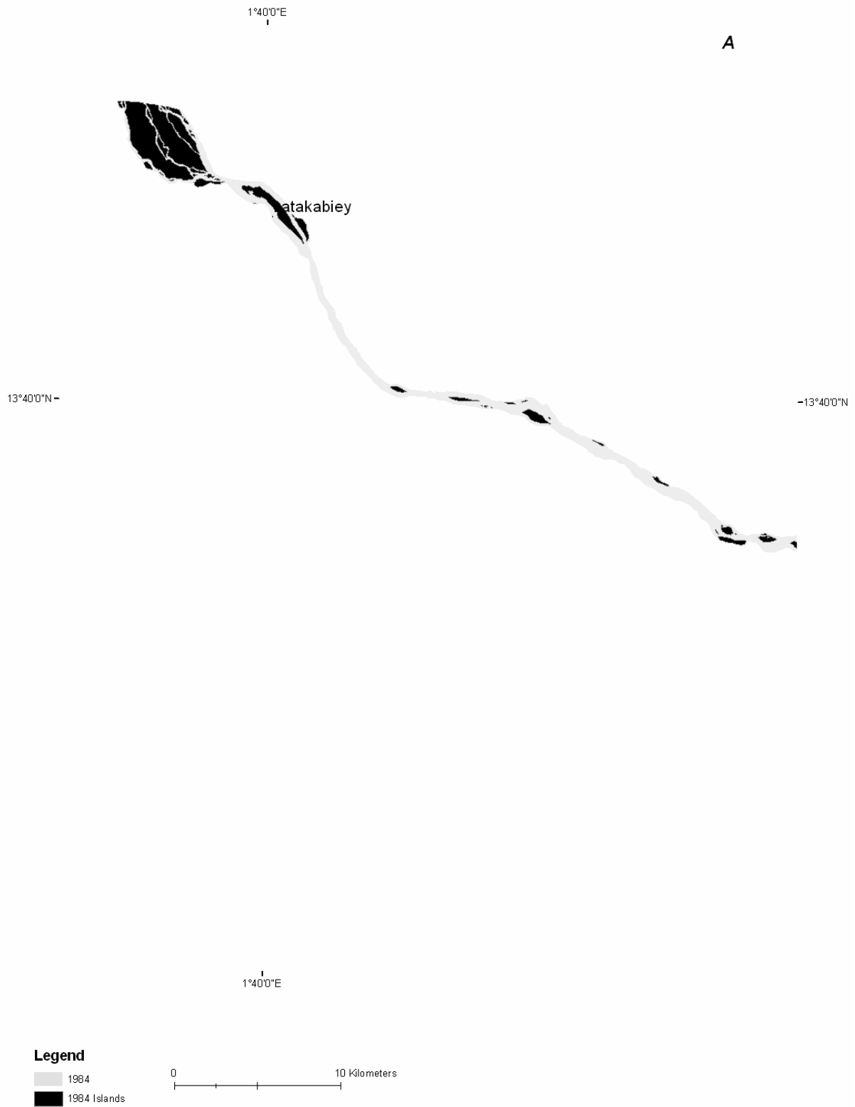
Figure B- 54A: Reach 2 channel bank and island extents in 1984
