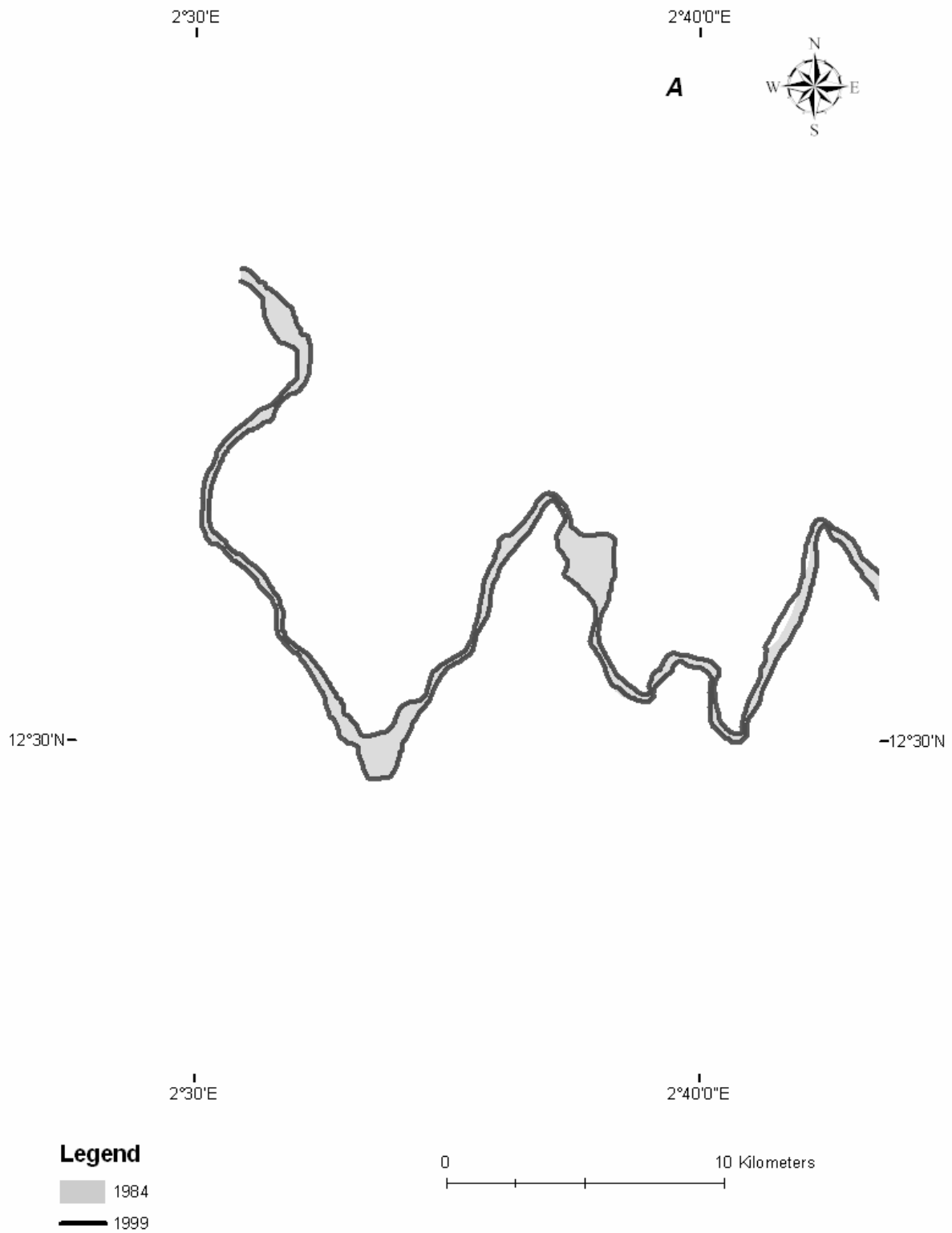
Figure B- 75A: Channel change in Reach 3 (1984-1999)
