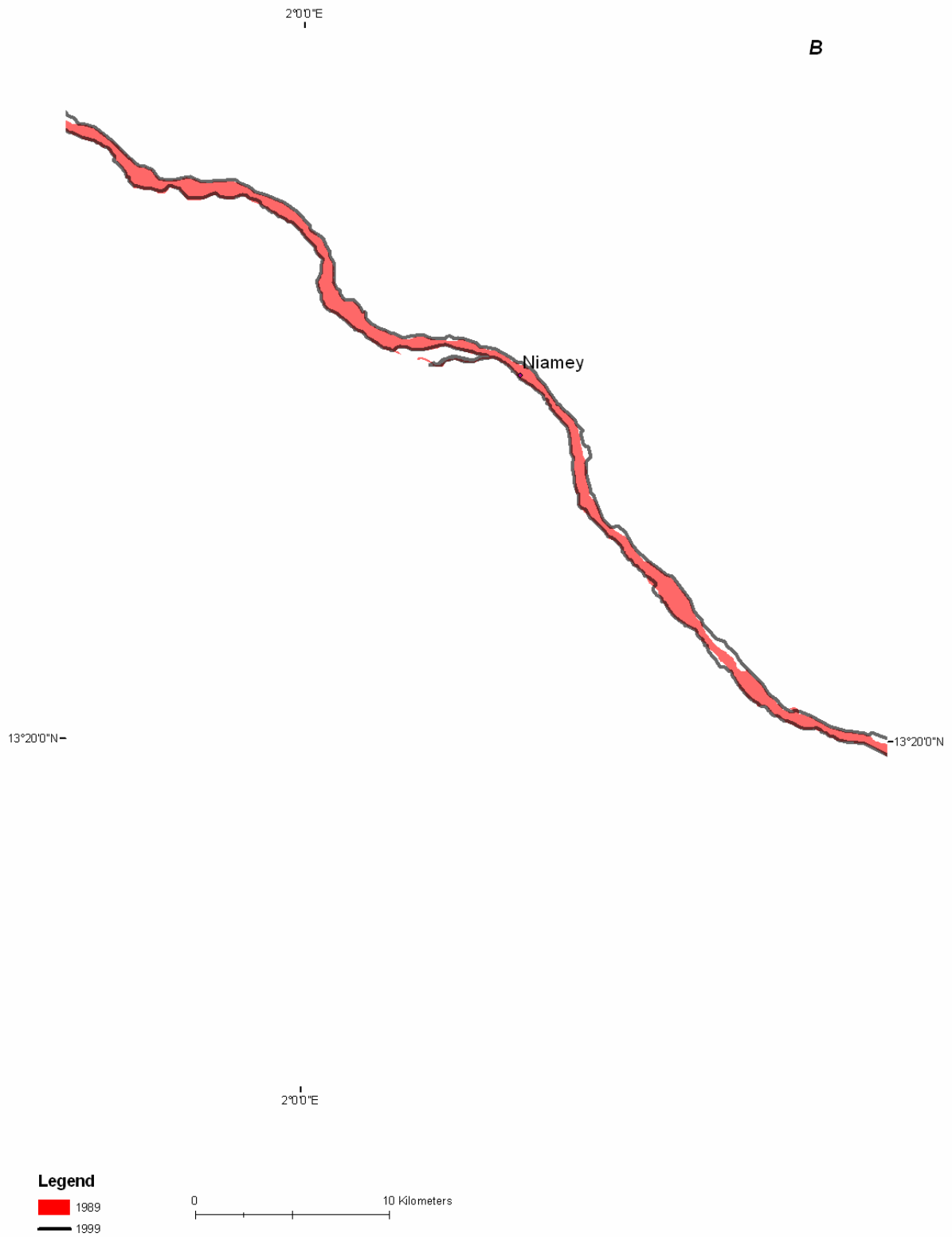
Figure B- 39B: Channel change in Reach 2 (1989-1999)
