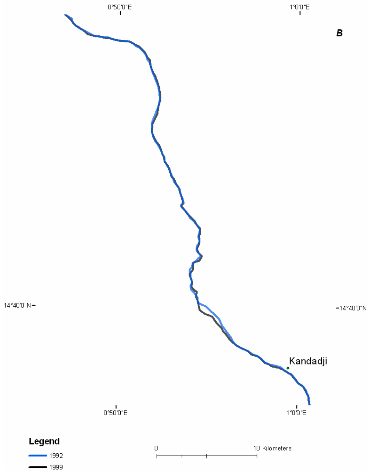
Figure B- 17B: River centre line change in reach 1 (1992 – 1999)
