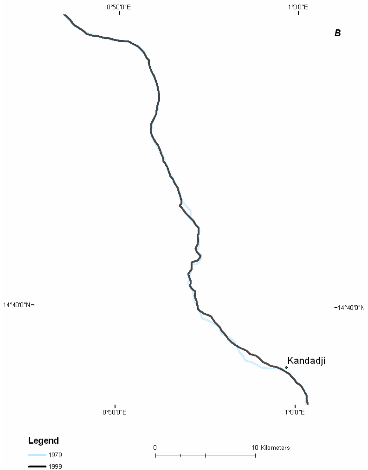
Figure B- 15B: River centre line change in reach 1 (1979 – 1999)
