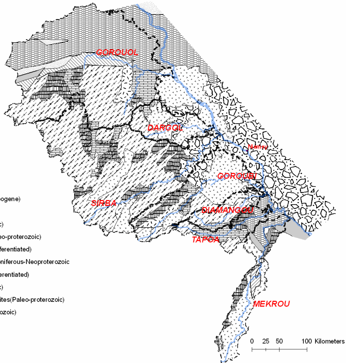
Figure I- 8: Geology of the Middle Niger basin adapted from Schlüter (2006)
