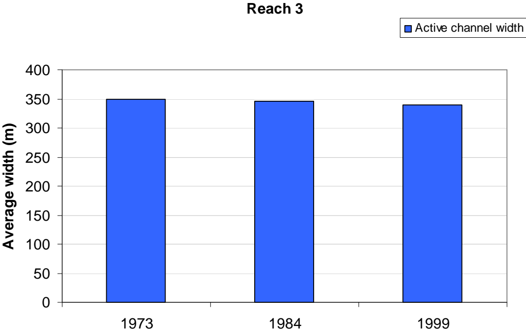
Figure II- 14: Channel width change in reach 3
