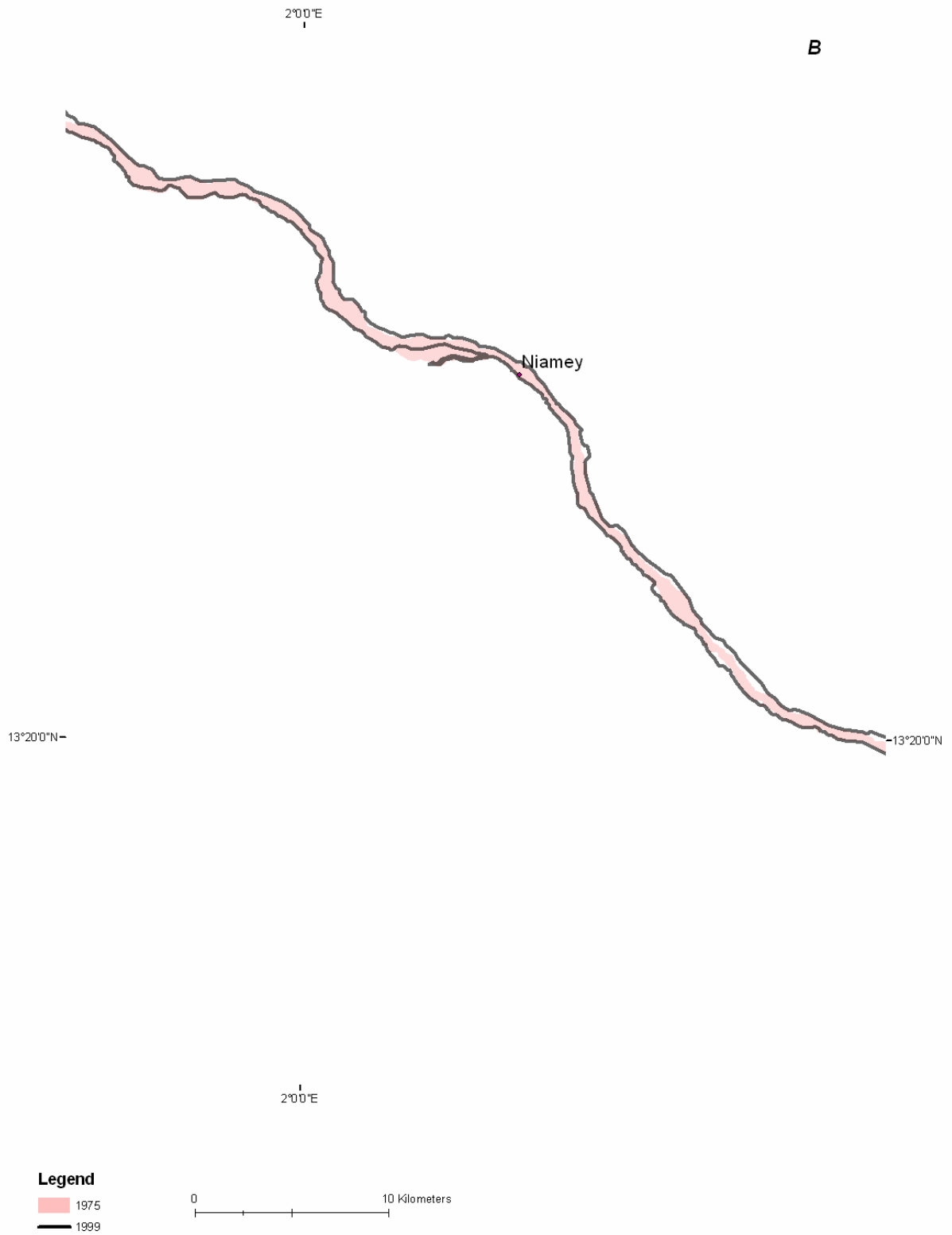
Figure B- 37B: Channel change in Reach 2 (1975-1999)
