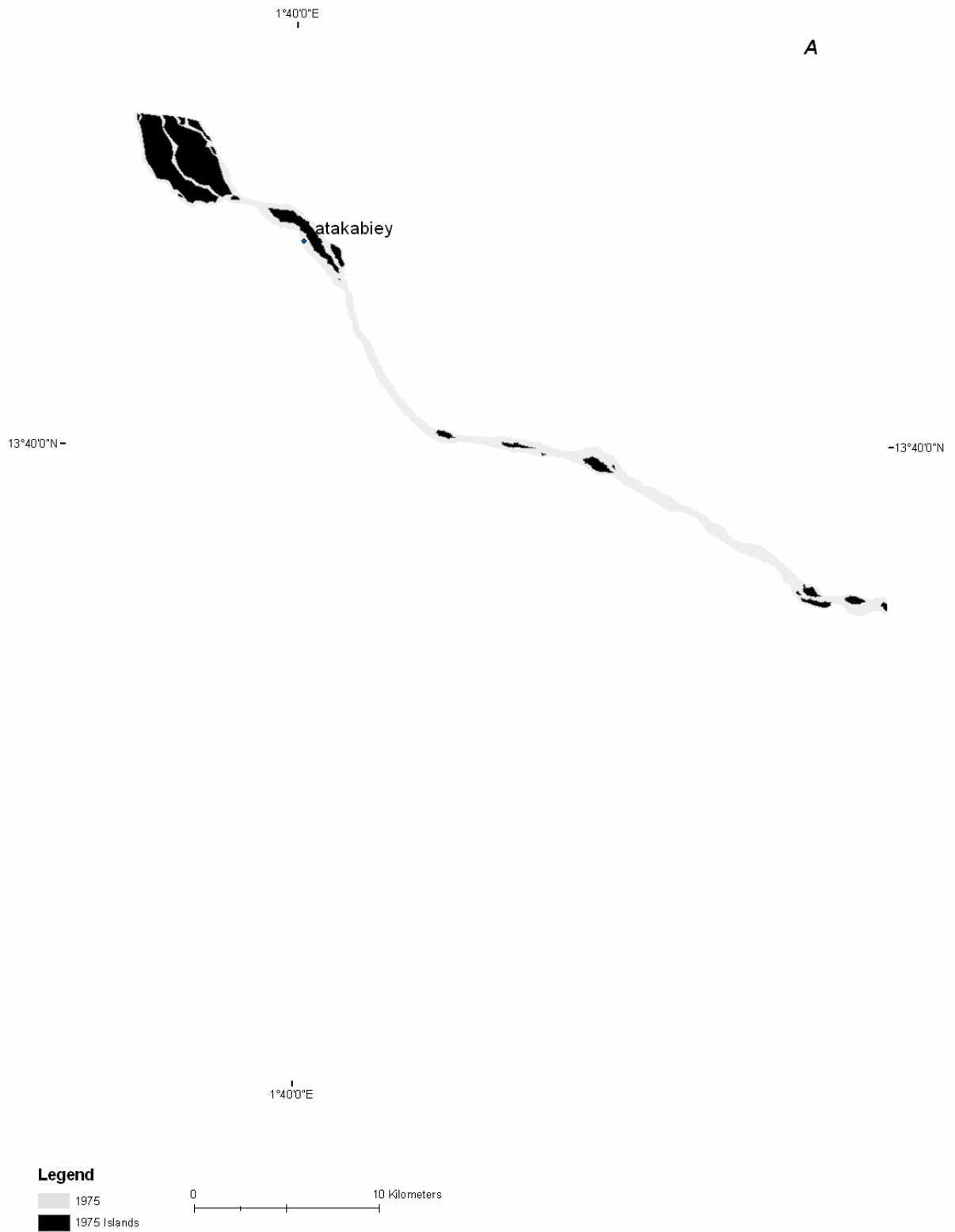
Figure B- 53A: Reach 2 channel bank and island extents in 1975
