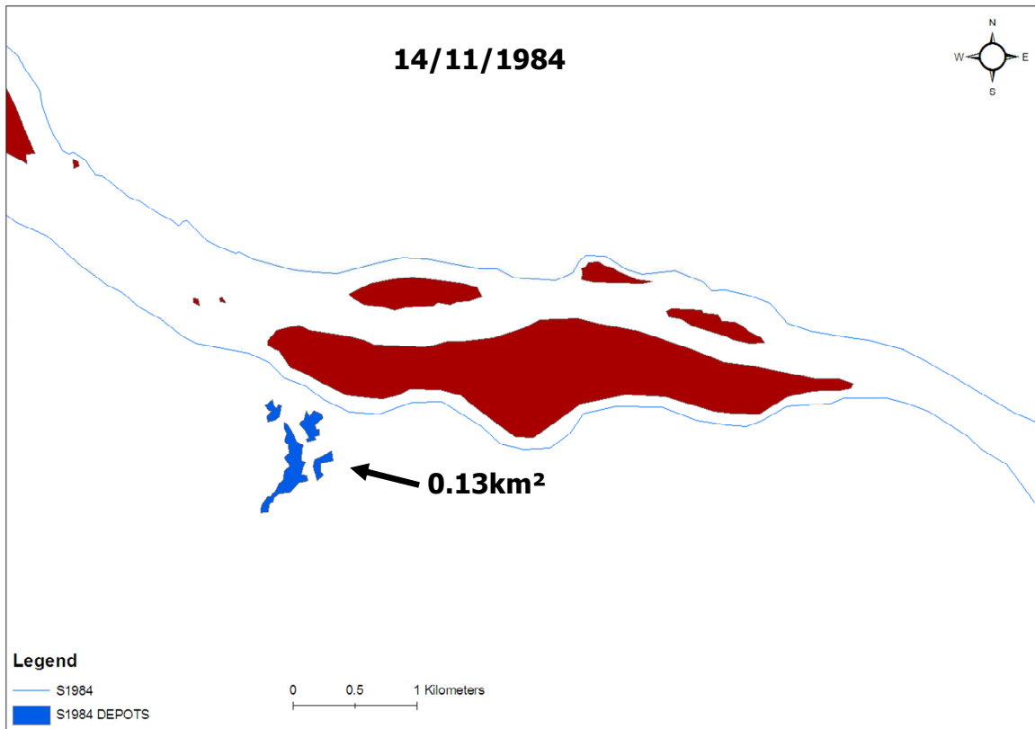
Figure II- 18: Alluvial deposits 1984
