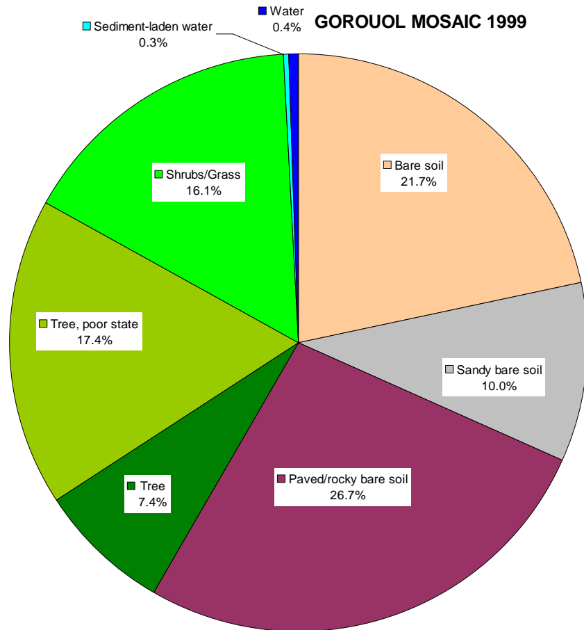
Figure III- 14: Percentage land cover composition for the Gorouol basin in 1999.
