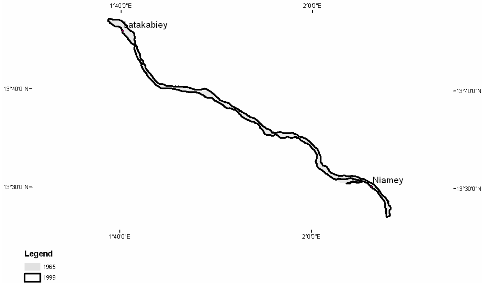
Figure B- 67: Channel change in a stretch of Reach 2 (1965-1999)
