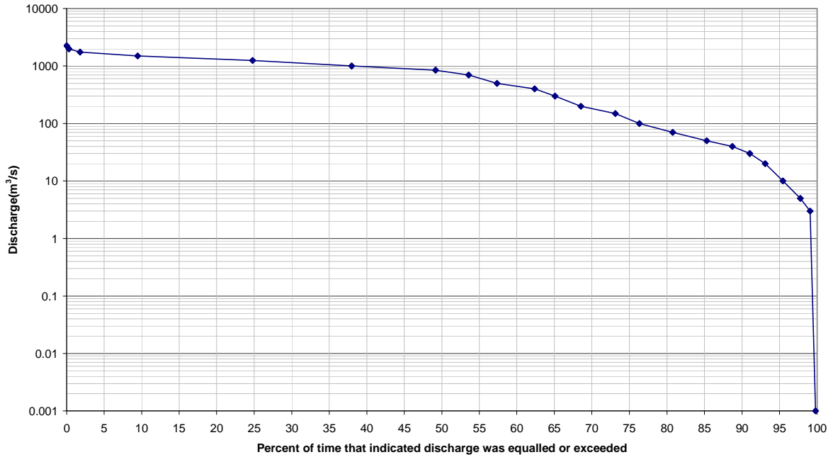
Figure D- 1: Flow duration curve, Niger at Niamey (1929-2006)
