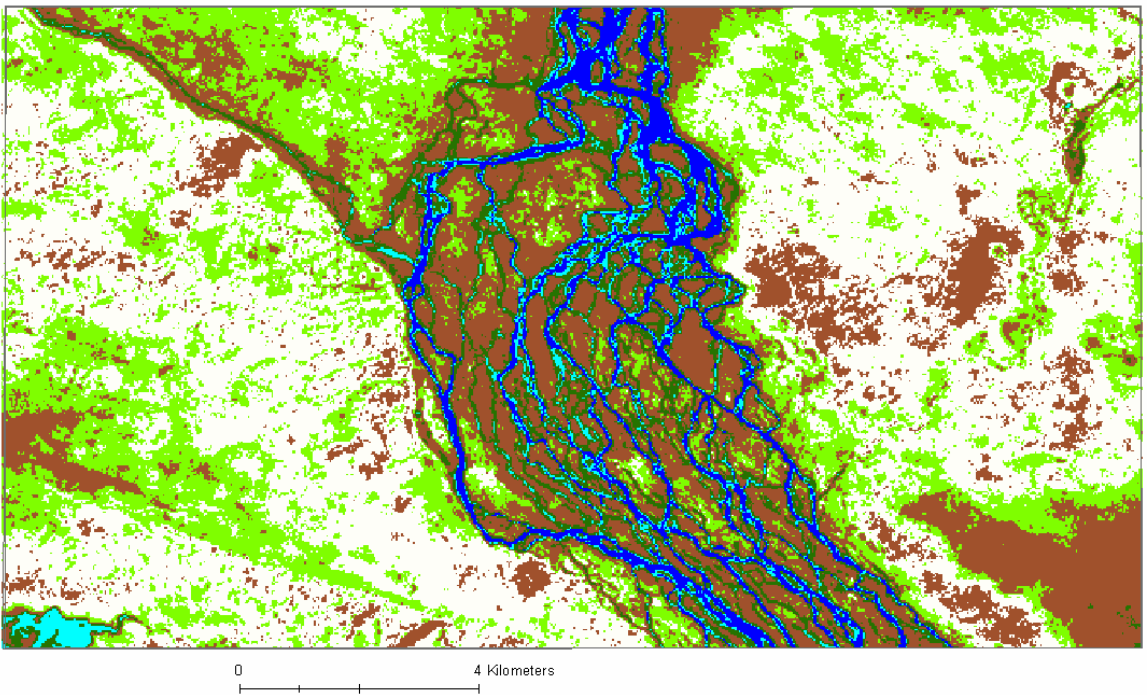
Figure II- 6: Example of the results of unsupervised classification
