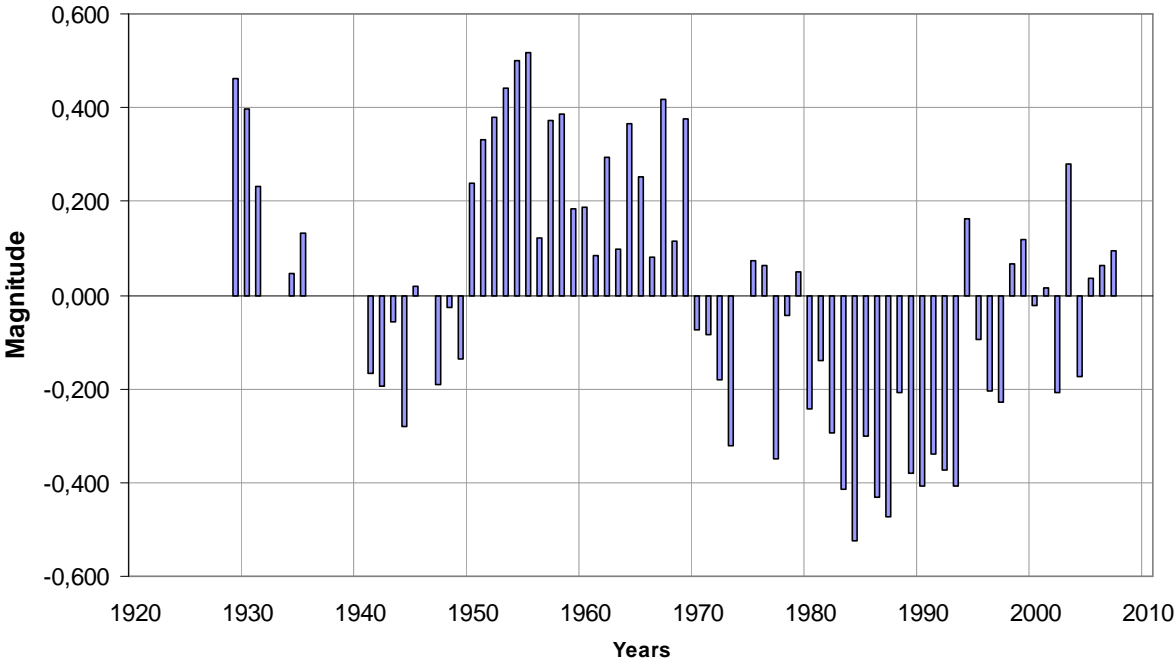
Figure IV- 12: Drought characterisation of river discharge of the Niger at Niamey (1929/30 to 2007/08) based on annual volume discharged
