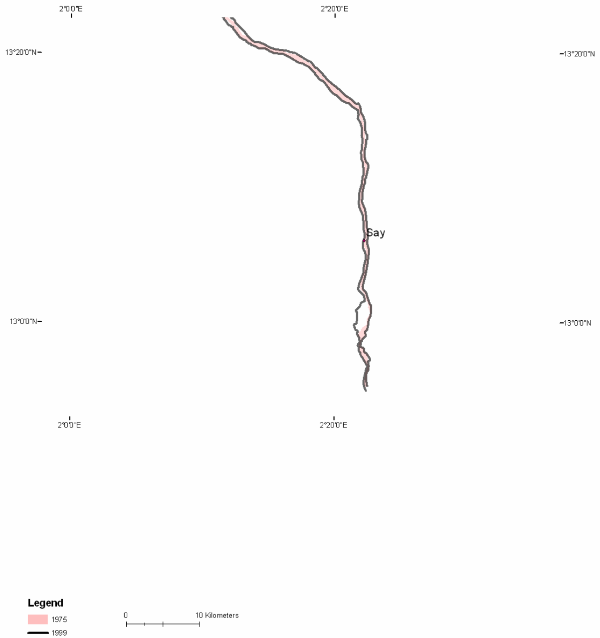
Figure B- 40C: Channel change in Reach 2 (1975-1999)
