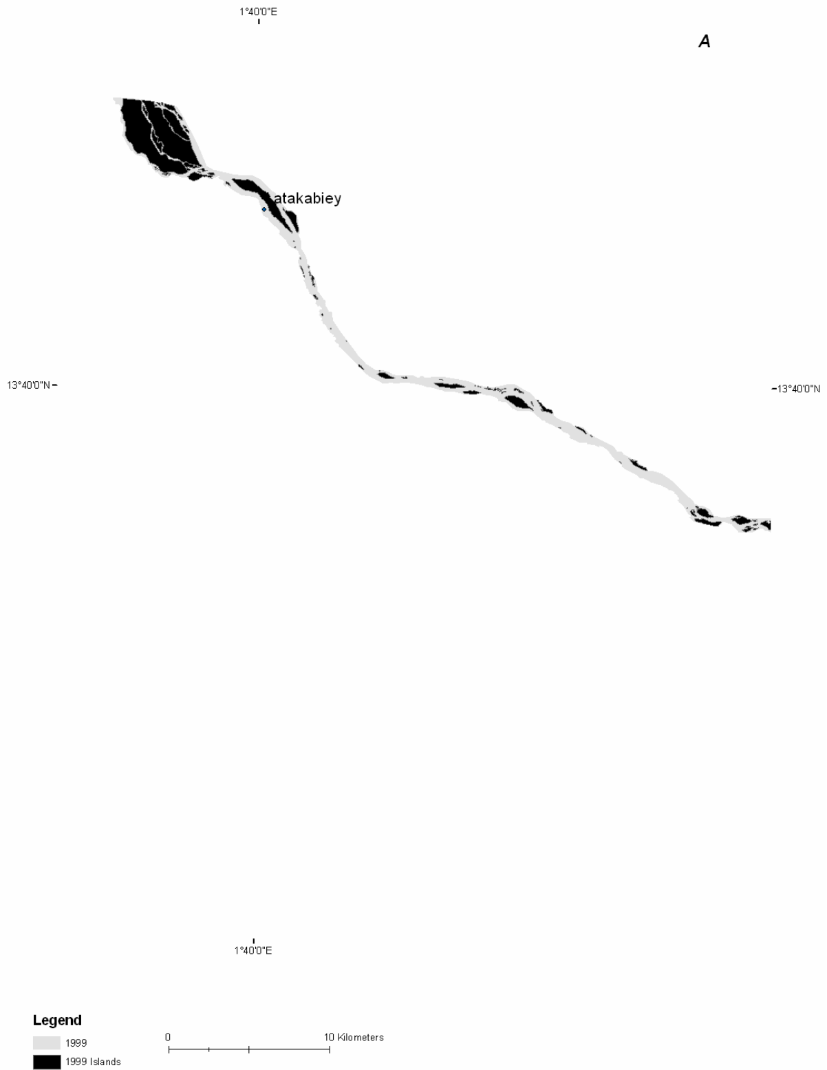
Figure B- 56A: Reach 2 channel bank and island extents in 1999
