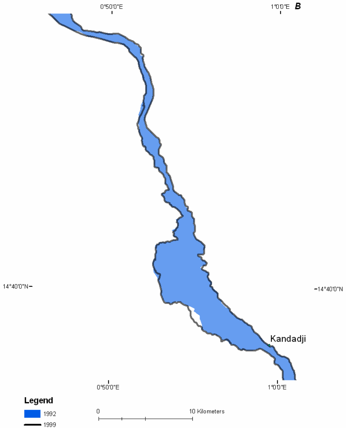
Figure B- 7B: Channel change in Reach 1 (1992-1999)
