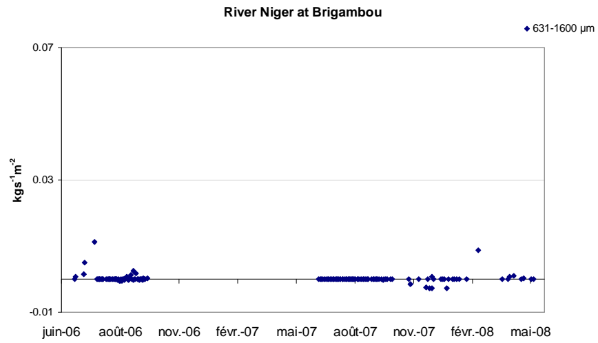
Figure V- 35: Deposition trend of suspended sediment (631-1600 μm) for the middle Niger River
