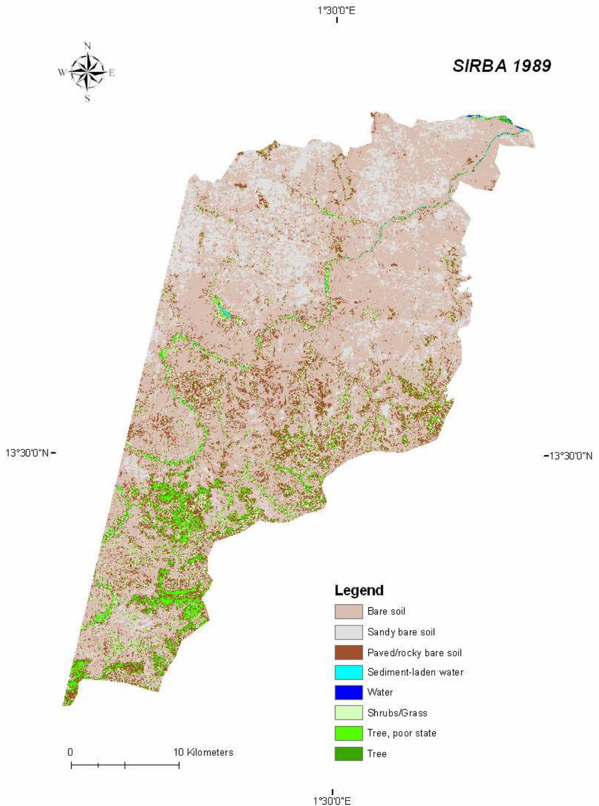
Figure III- 29: Sirba basin land cover.20/11/1989 (1105 km 2 )
