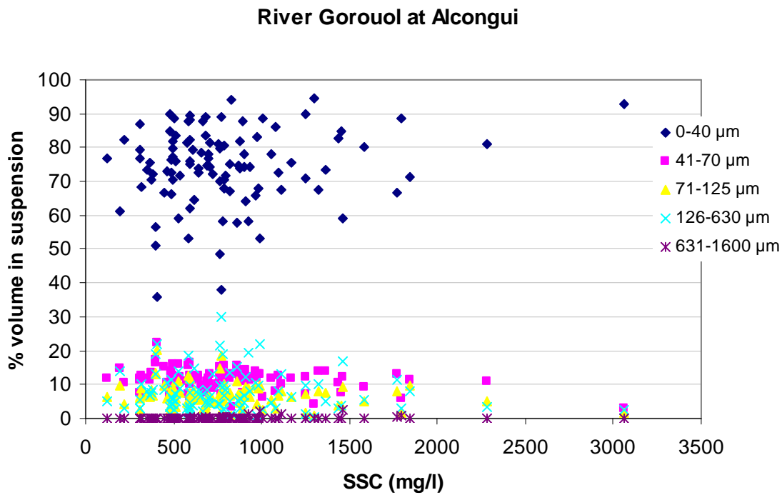
Figure V- 12: SSC and particle size data for the River Gorououl at Alcongui
