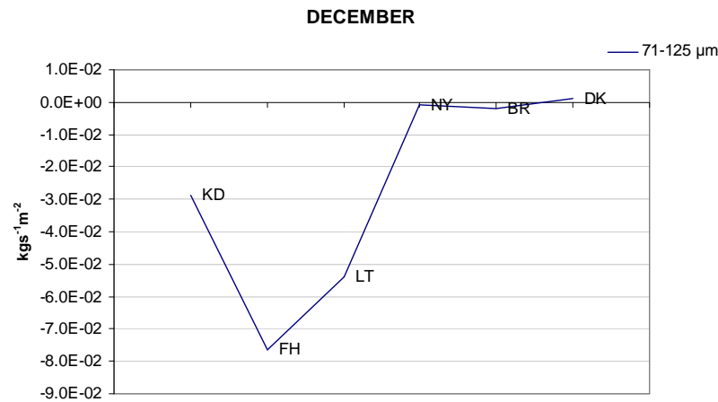
Figure V- 37: Suspended sediment dynamics of the 71-125 μm size class
