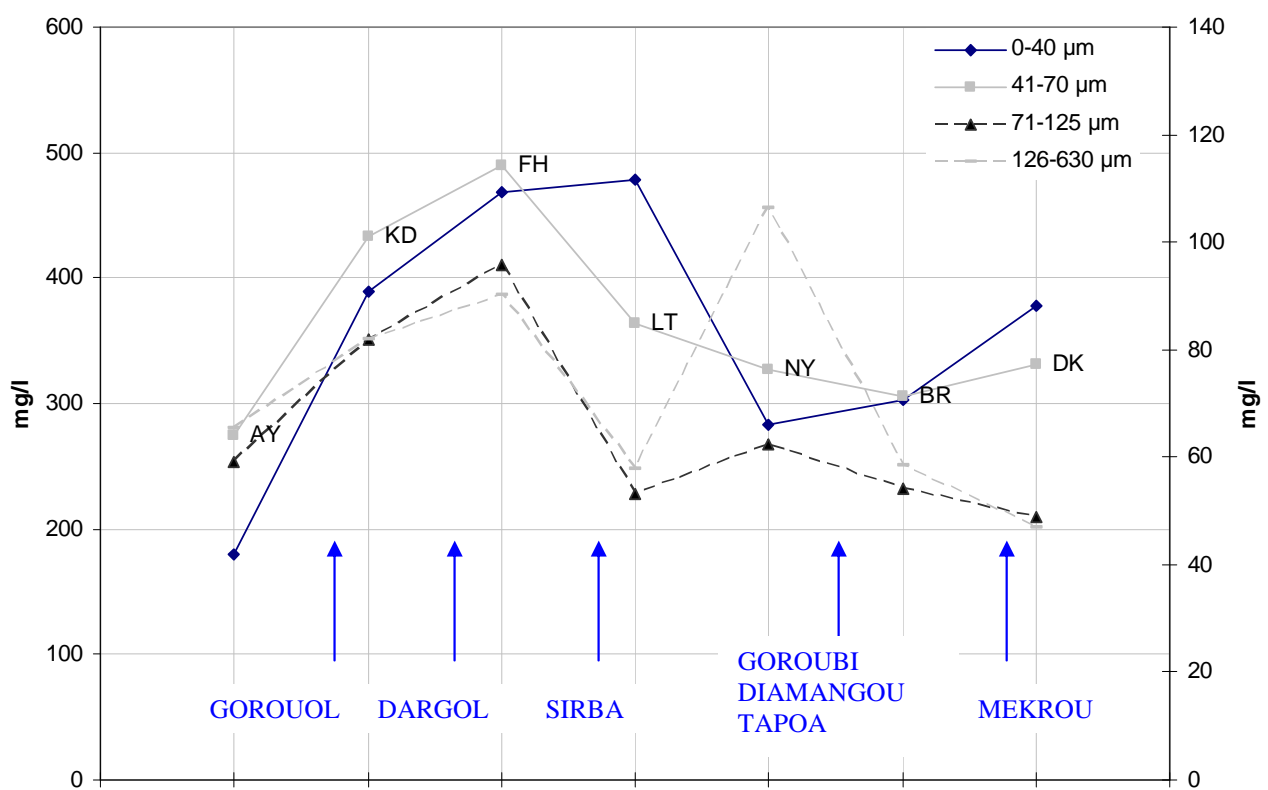
Figure V- 26 : Mean SSC values transported along the middle Niger River (0-630 \mu\text{m} )
