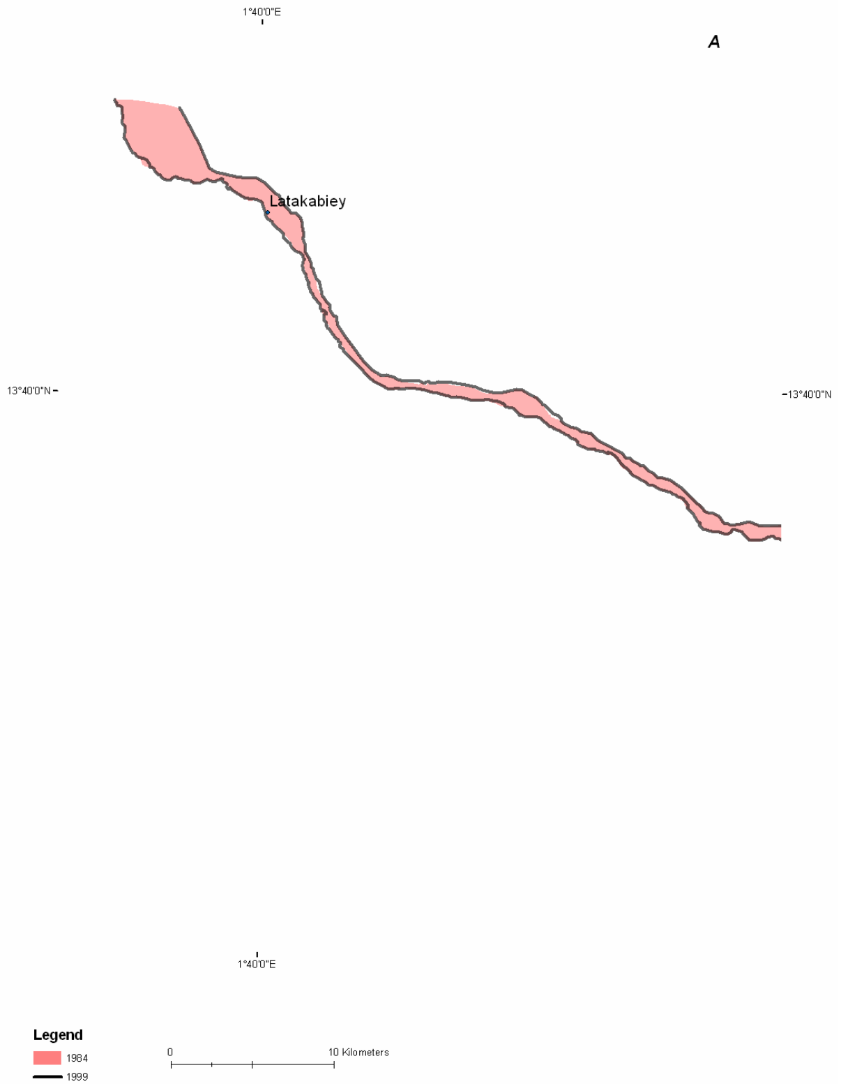
Figure B- 35A: Channel change in Reach 2 (1984-1999)
