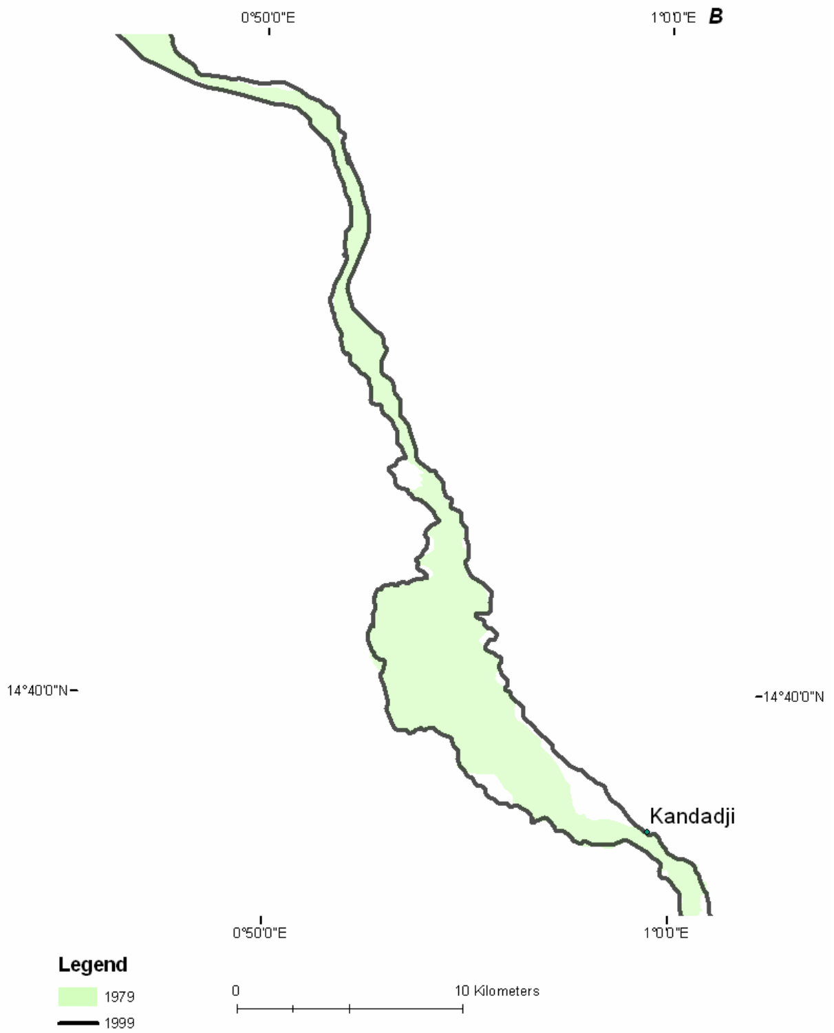
Figure B- 5B: Channel change in Reach 1 (1979-1999)
