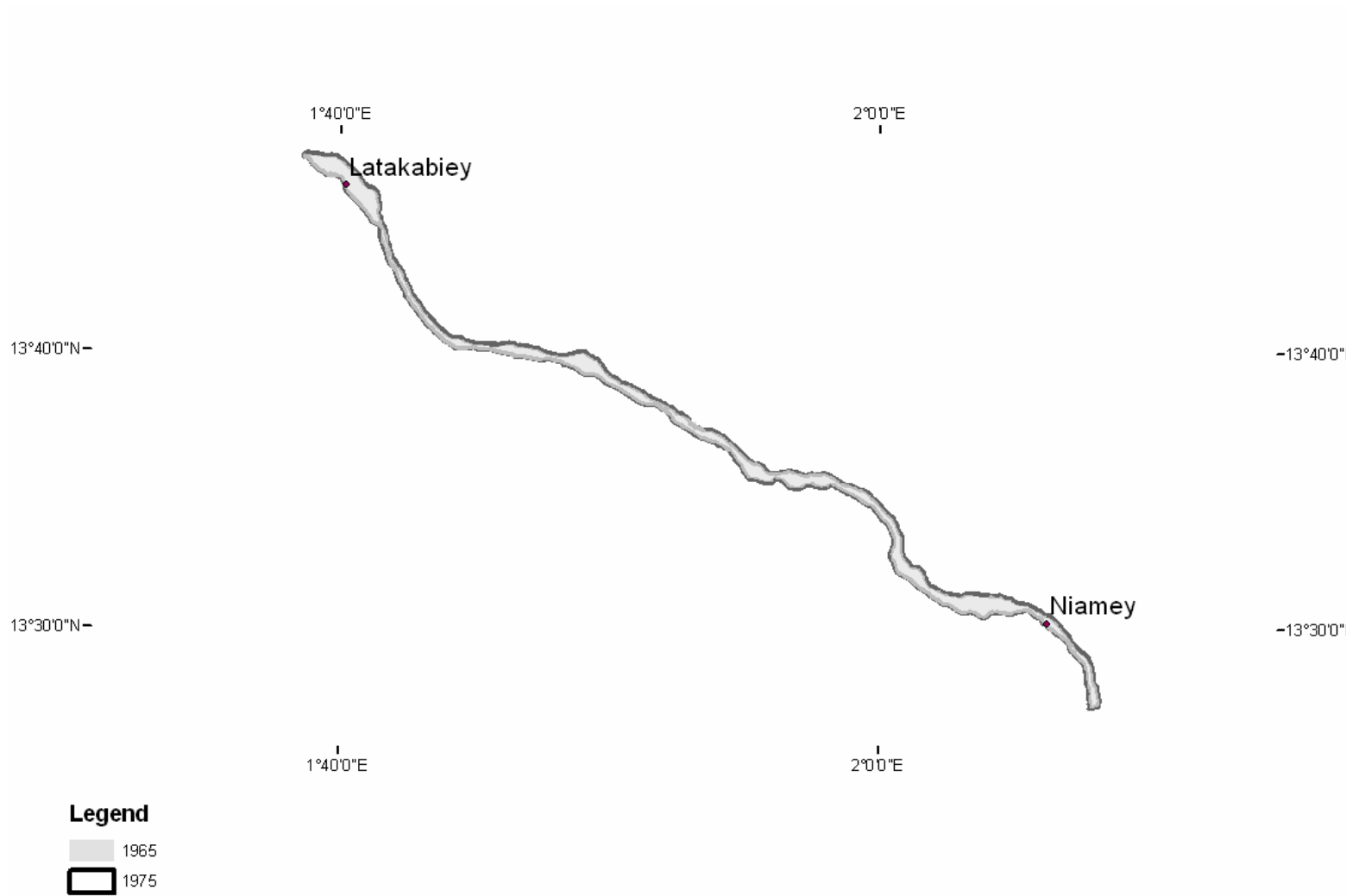
Figure B- 66: Channel change in a stretch of Reach 2 (1965-1975)
