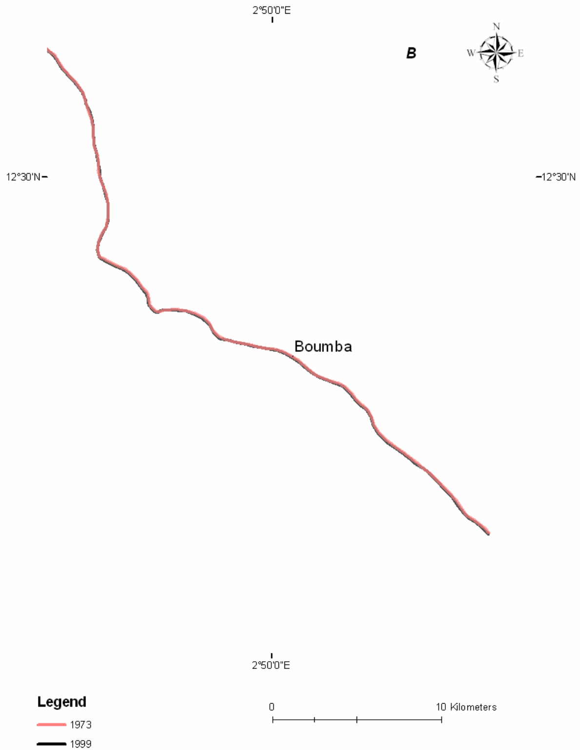
Figure B- 80B: River centre line change in reach 3 (1973 – 1999)
