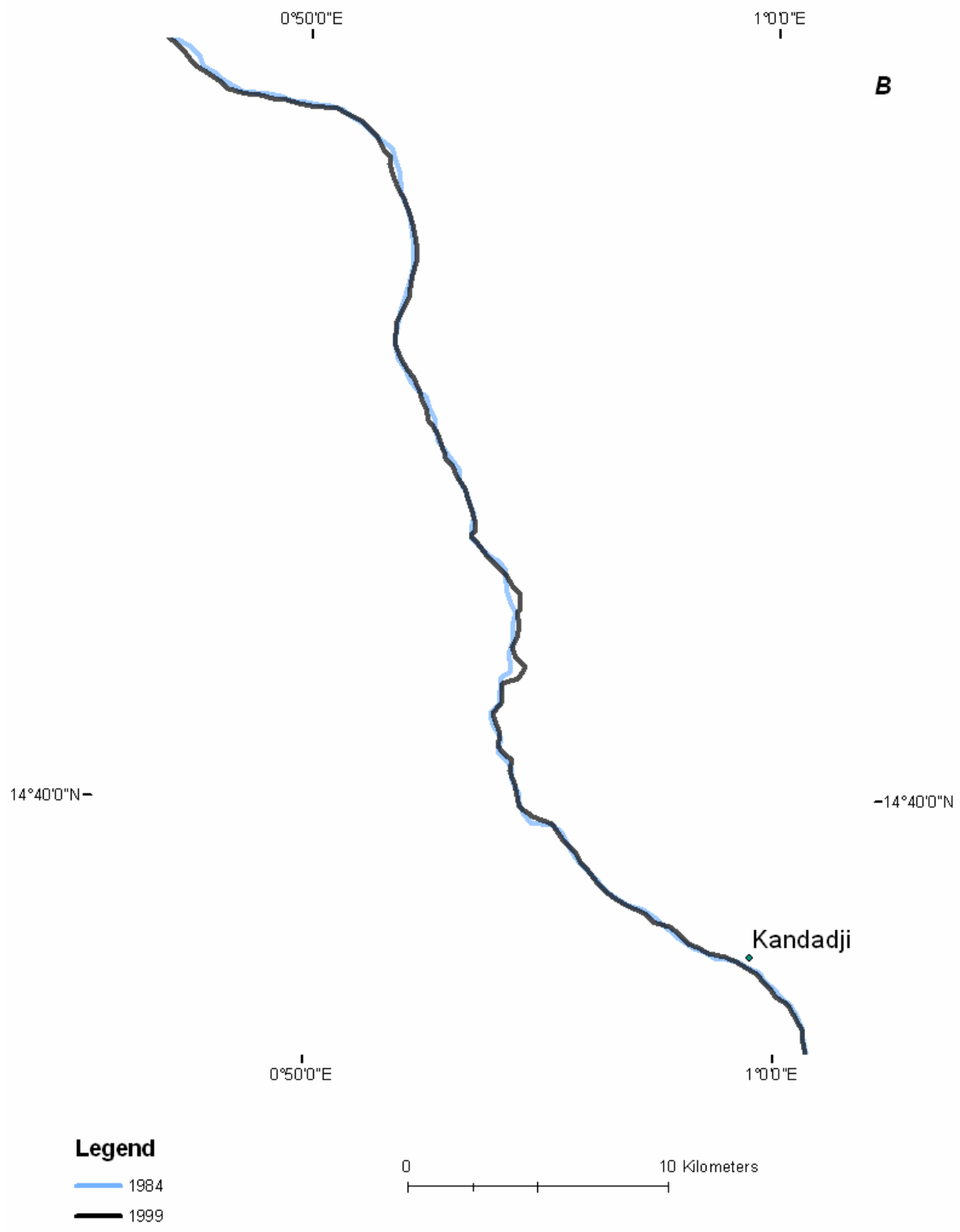
Figure B- 16B: River centre line change in reach 1 (1984 – 1999)
