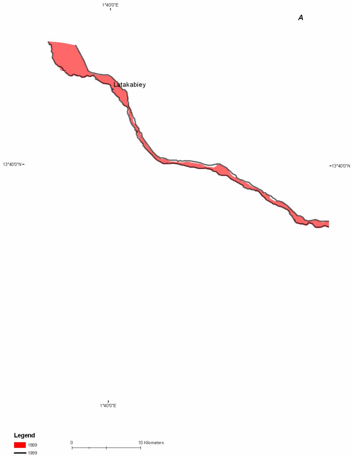
Figure B- 36A: Channel change in Reach 2 (1989-1999)
