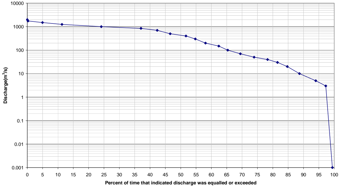
Figure D- 5: Flow duration curve, Niger at Niamey (Dry spell)
