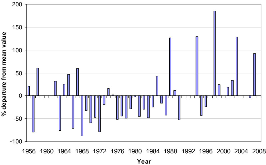
Figure IV- 16: Percentage departure from mean annual cumulative discharge for the Sirba River
