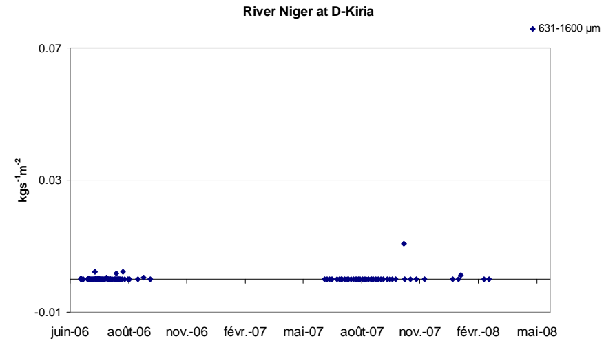
Figure V- 35: Deposition trend of suspended sediment (631-1600 μm) for the middle Niger River
