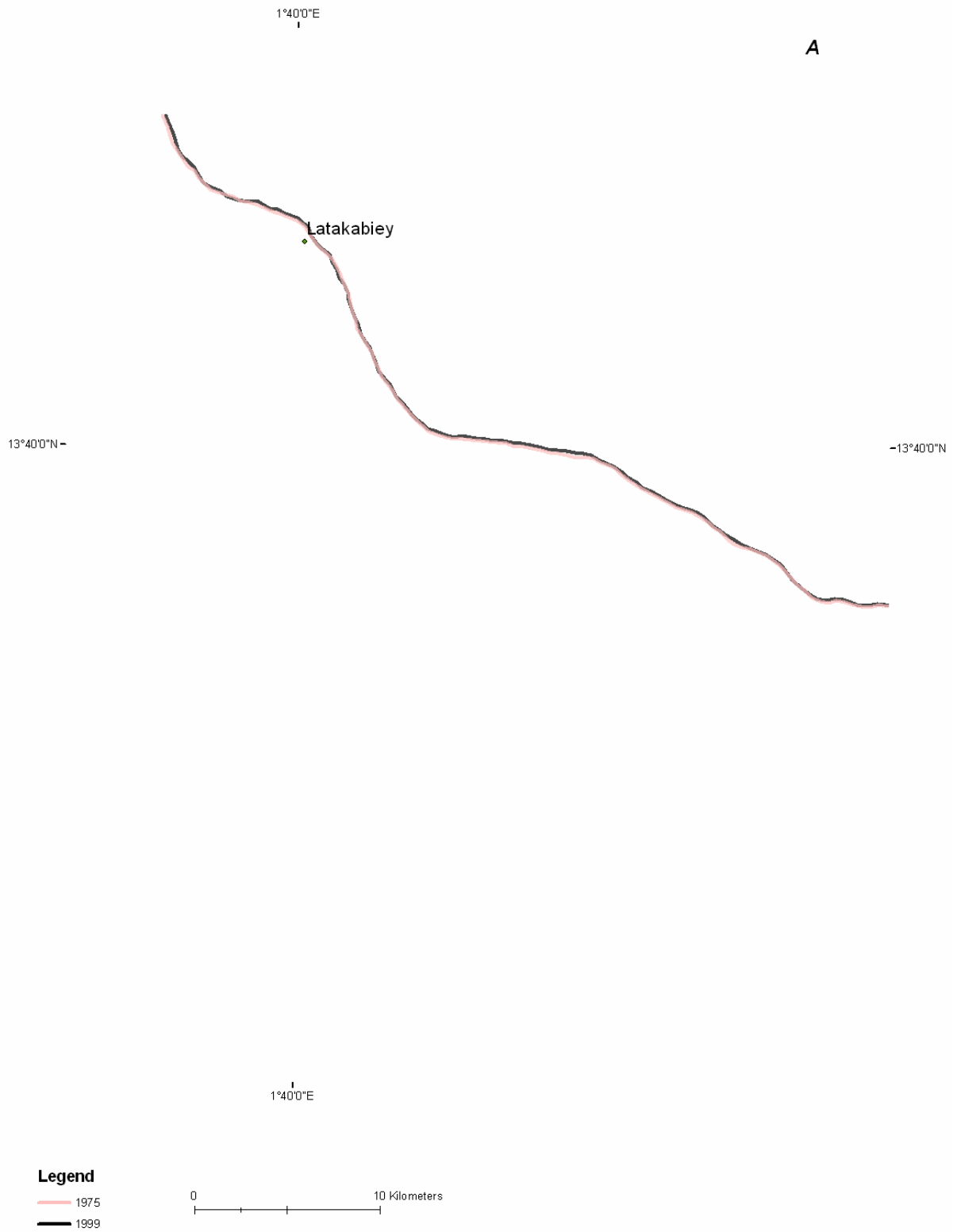
Figure B- 44A: River centre line change in reach 2 (1975 – 1999)
