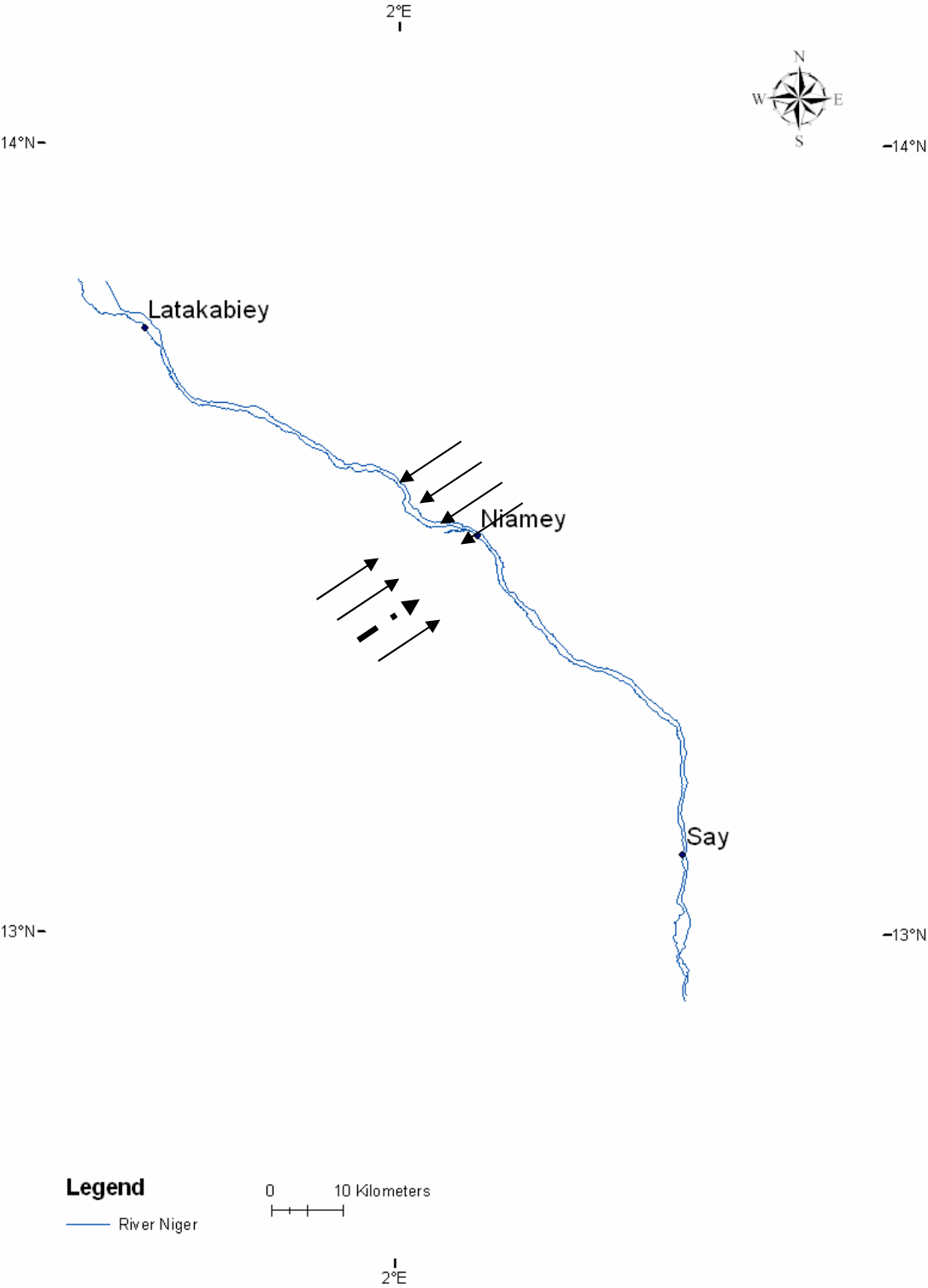
Figure II- 16: Lateral sediment sources of the middle Niger River
