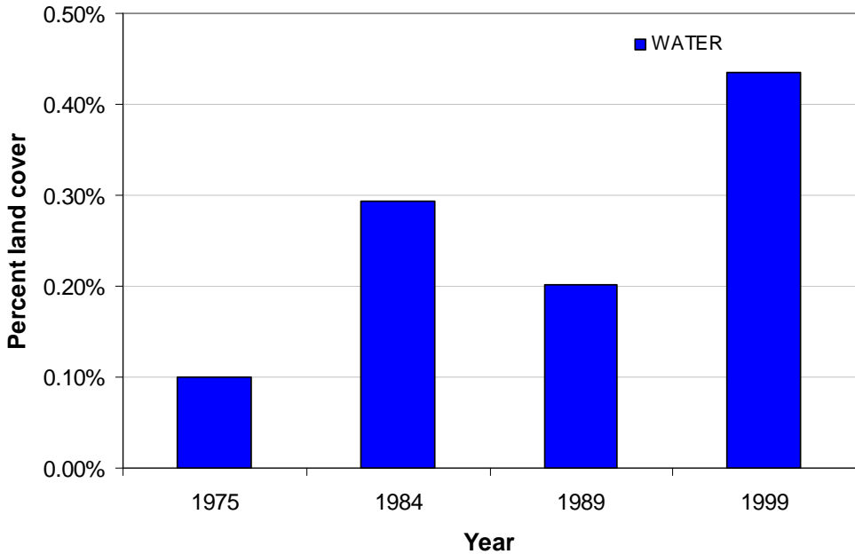
Figure III- 32: Water surface area in the Sirba basin (1975-1999)
