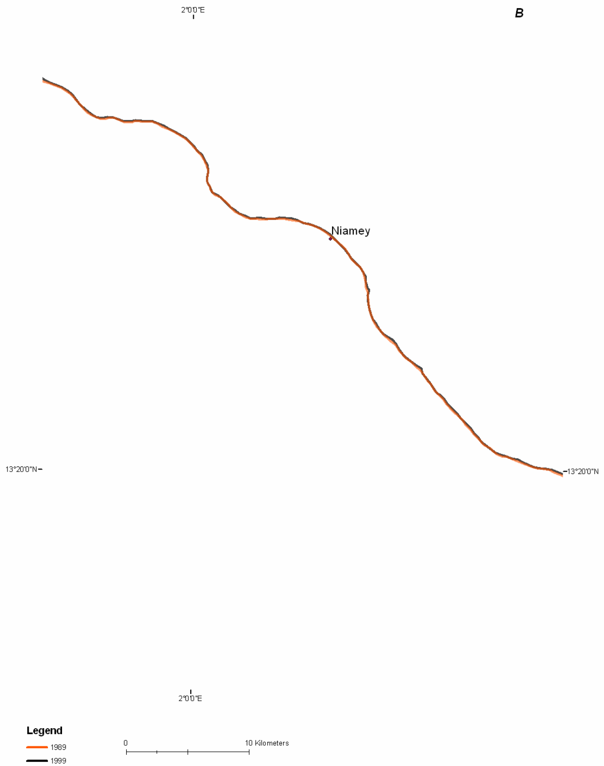
Figure B- 49B: River centre line change in reach 2 (1989 – 1999)
