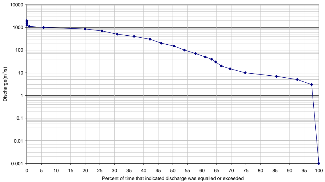
Figure D- 6: Flow duration curve, Niger at Niamey (Driest year)
