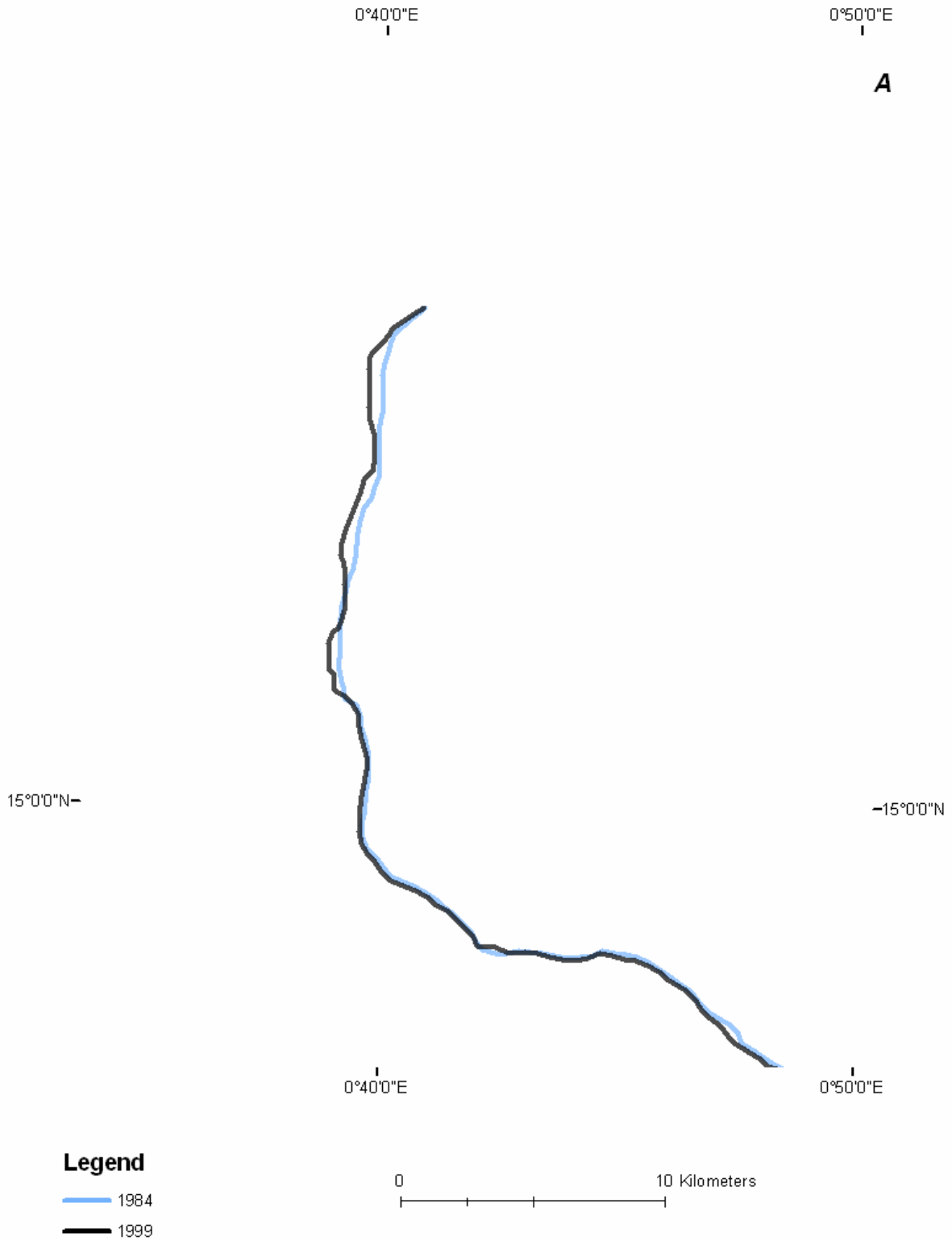
Figure B- 13A: River centre line change in reach 1 (1984 – 1999)
