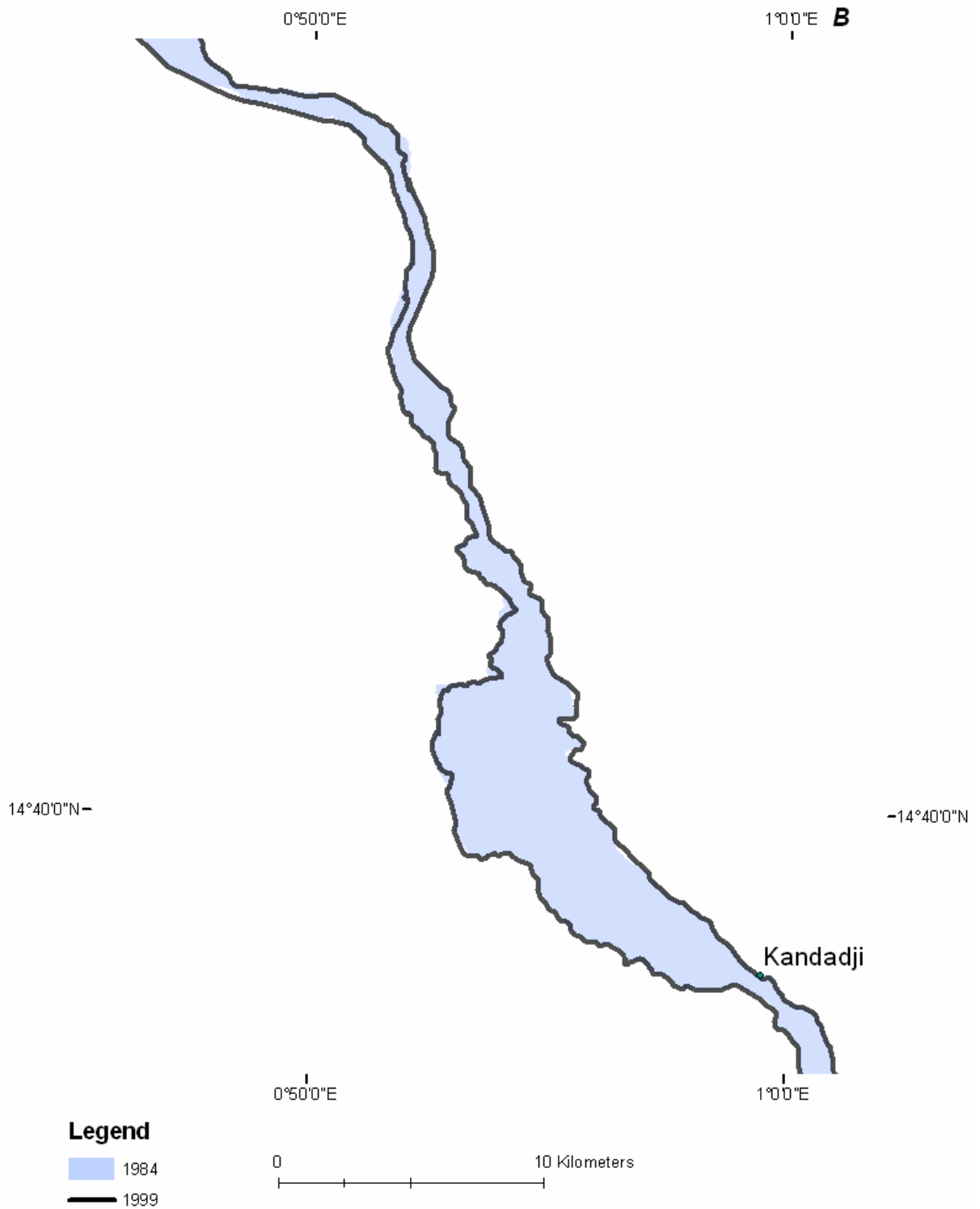
Figure B- 6B: Channel change in Reach 1 (1984-1999)
