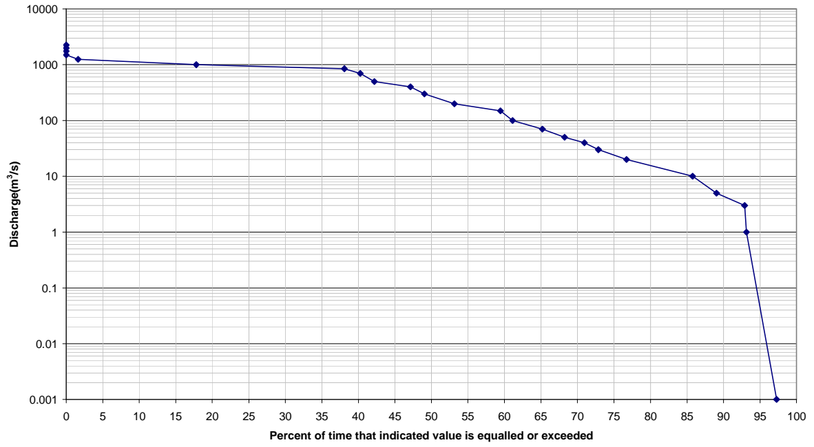
Flow duration curve(log interval) for River Niger at Niamey(1985/86)
