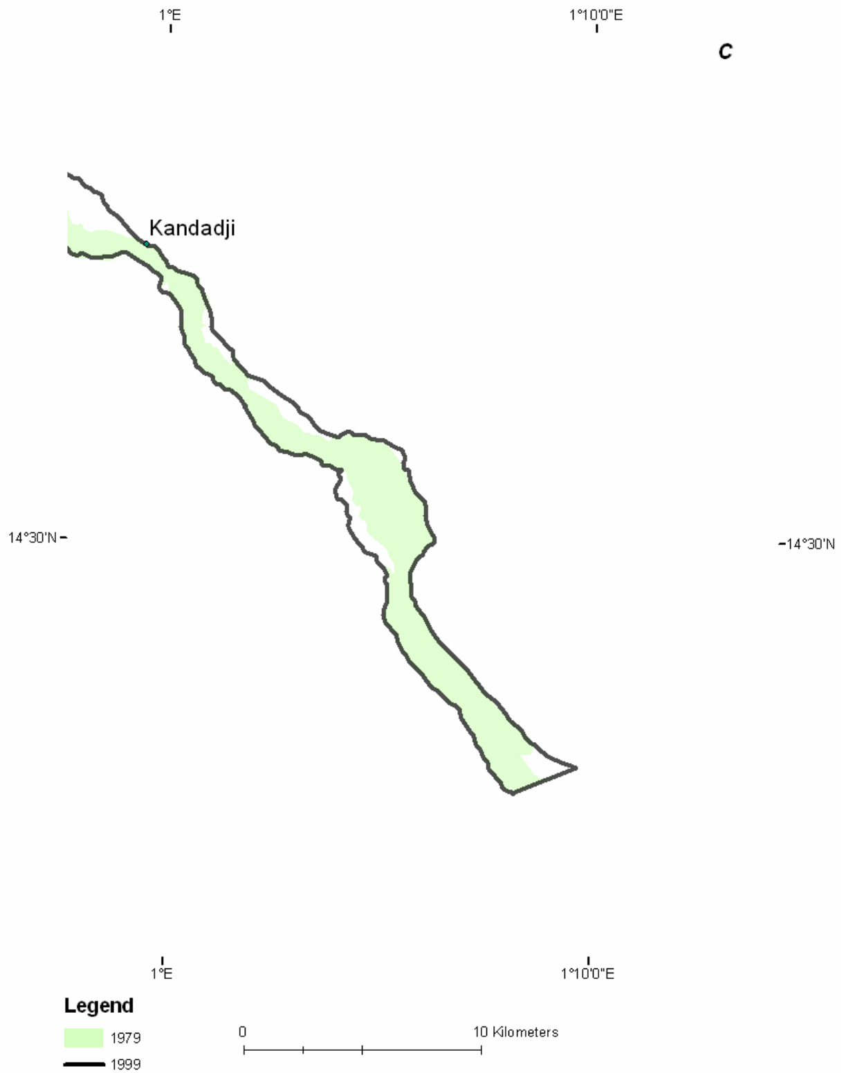
Figure B- 8C: Channel change in Reach 1 (1979-1999)
