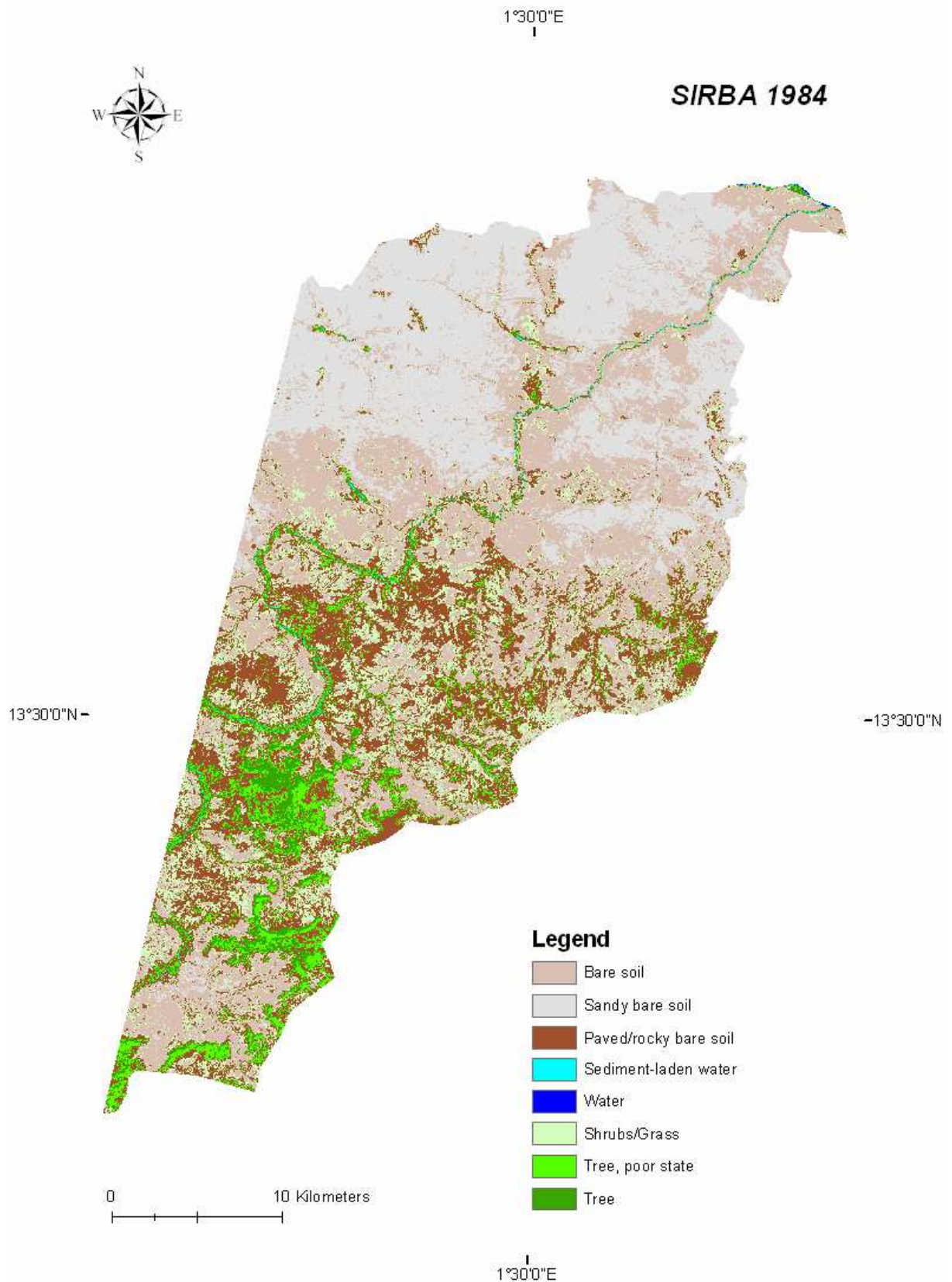
Figure III- 28: Sirba basin land cover.14/11/1984 (1105 km 2 )
