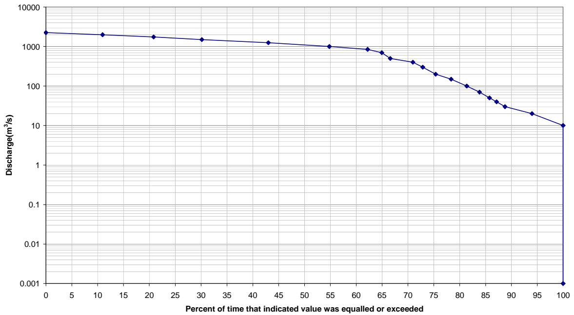
Figure D- 4: Flow duration curve, Niger at Niamey (Maximum daily discharge)
