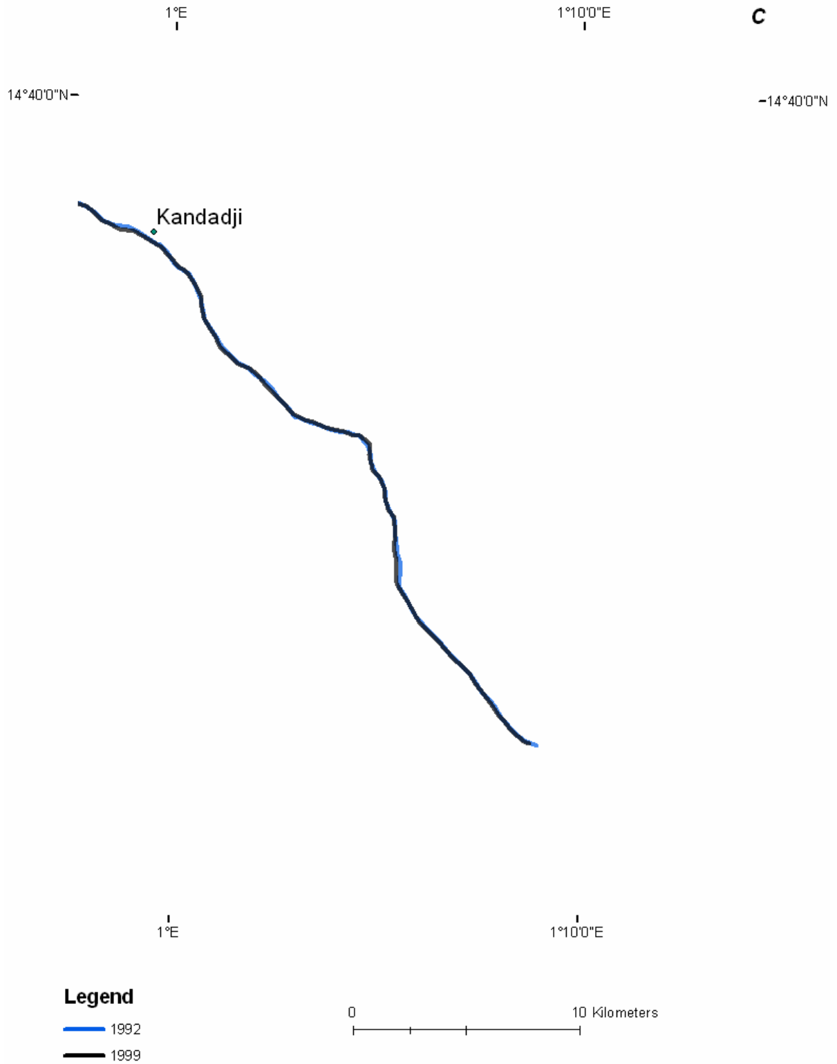
Figure B- 20C: River centre line change in reach 1 (1992 – 1999)
