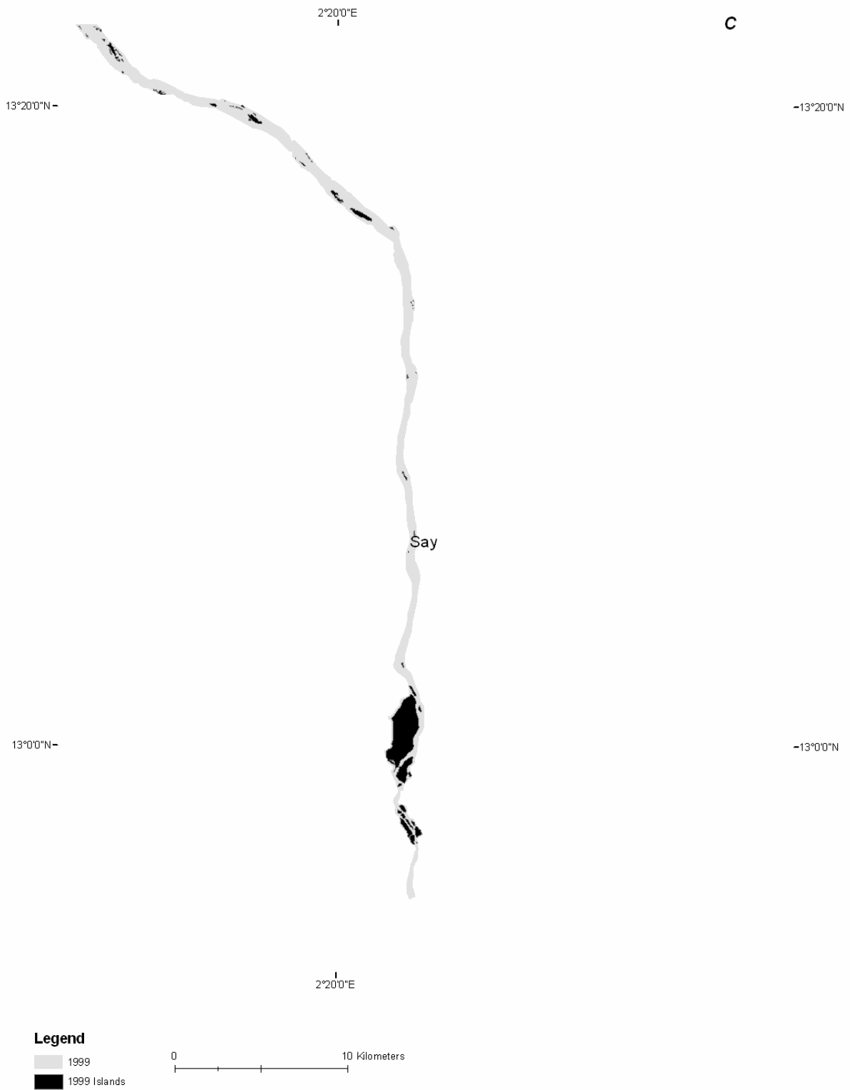
Figure B- 64C: Reach 2 channel bank and island extents in 1999
