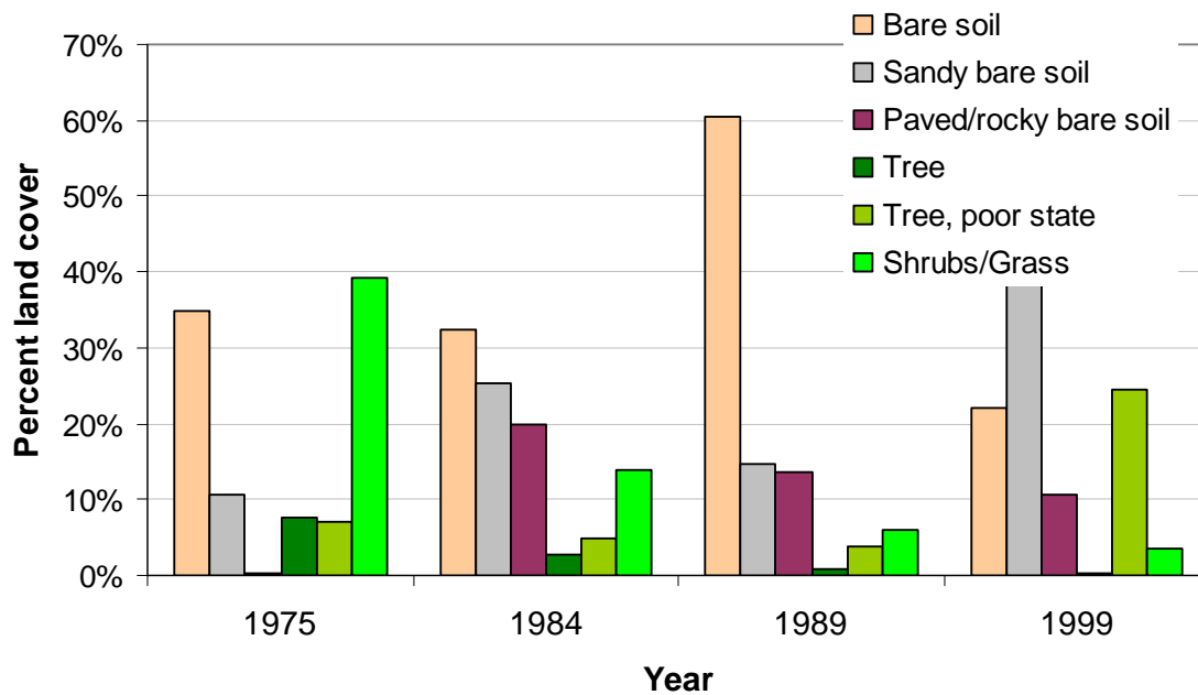
Figure C- 9: Percentage land cover Sirba 1975-1999
