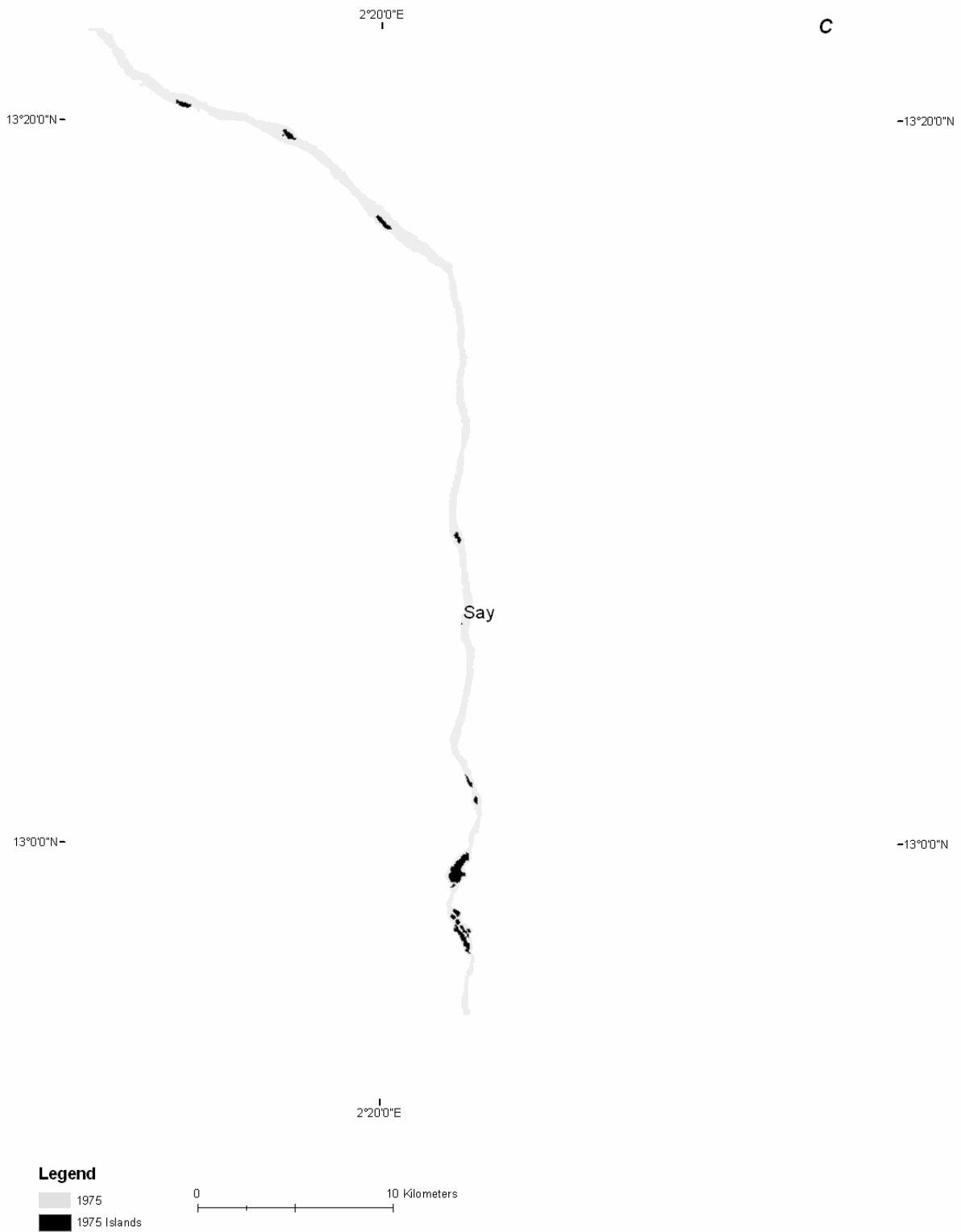
Figure B- 61C: Reach 2 channel bank and island extents in 1975
