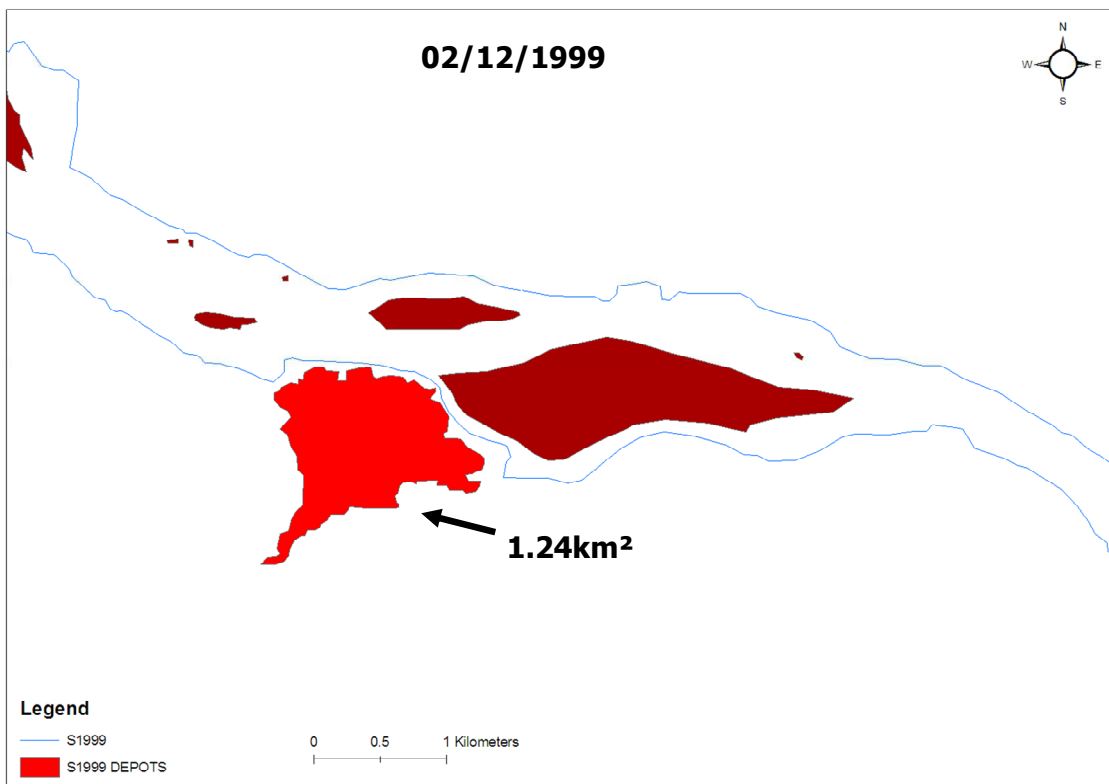
Figure II- 20: Alluvial deposits 1999
