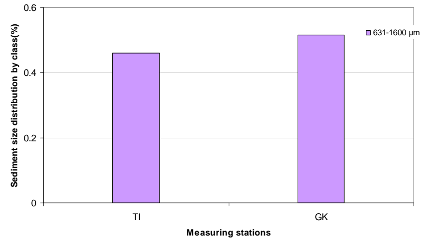
Figure V- 19 : Mean suspended sediment size distribution by percent transported by the River Sirba at Tiambi (n=123 samples) and G-Kourou (n=168 samples)
