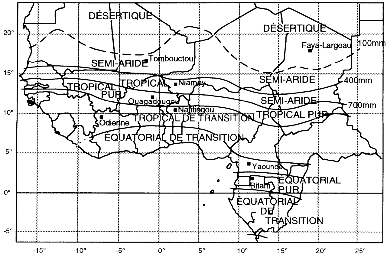
Figure IV- 1: West and central African climates after L'Hôte et al. [1996]
