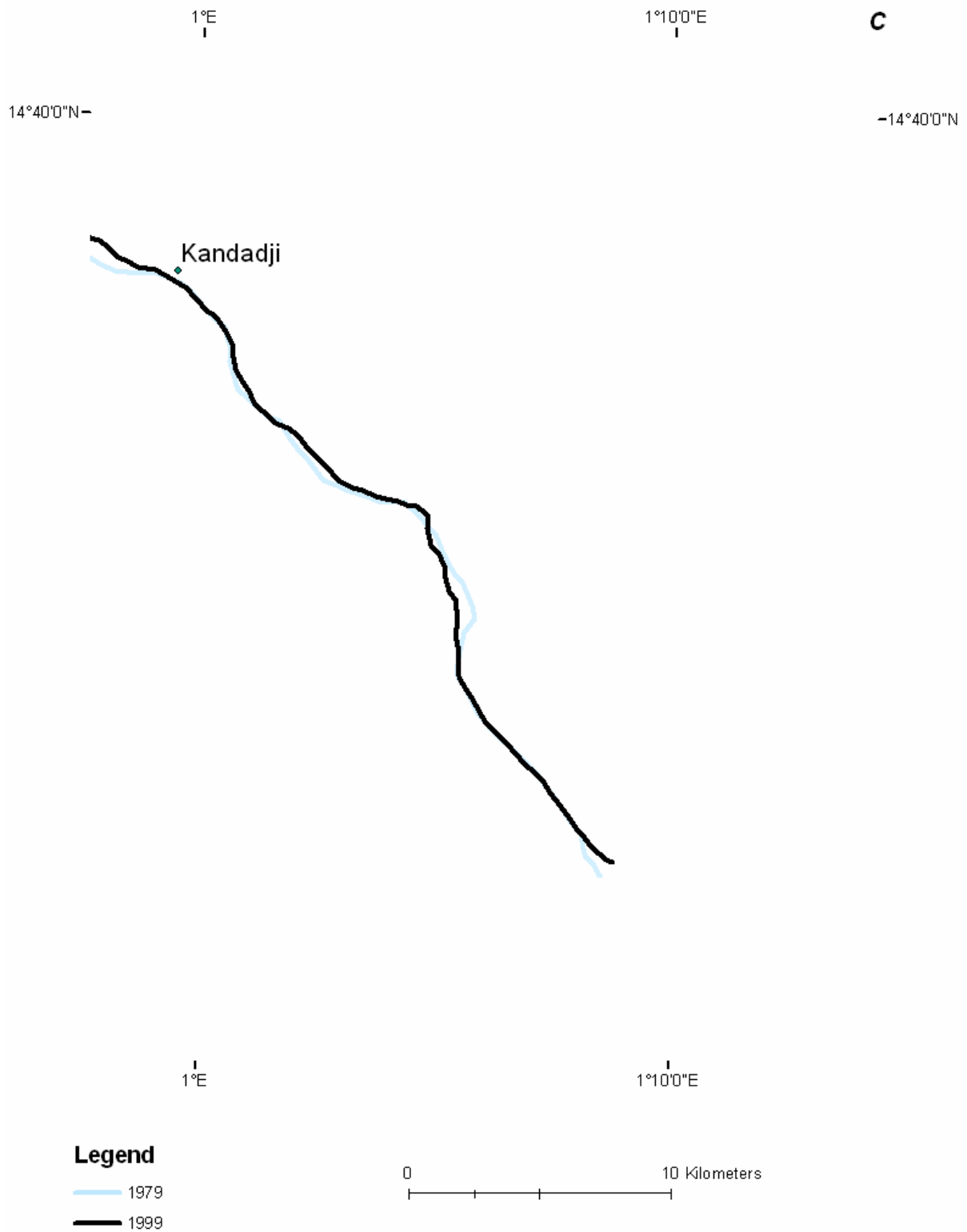
Figure B- 18C: River centre line change in reach 1 (1979 – 1999)
