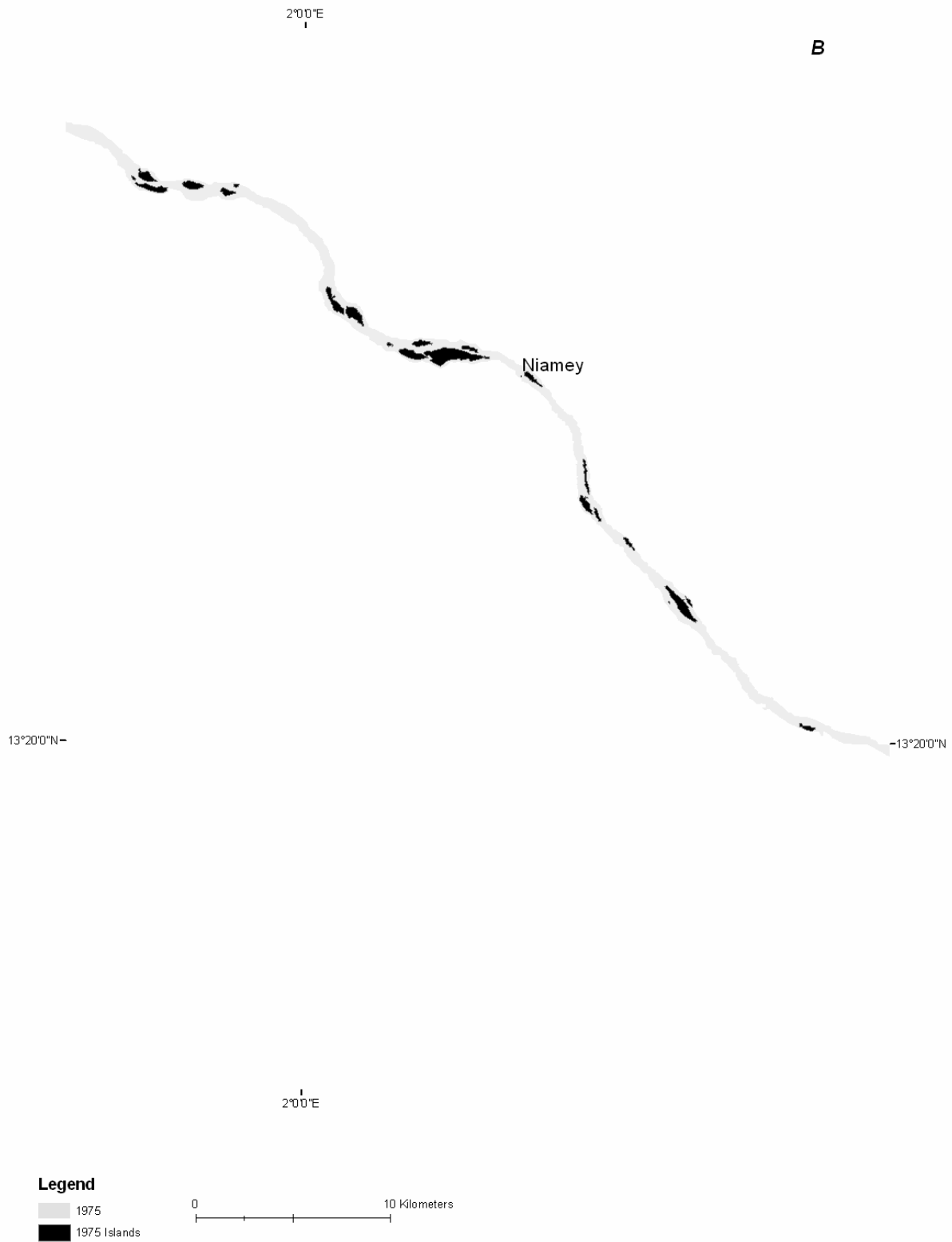
Figure B- 57B: Reach 2 channel bank and island extents in 1975
