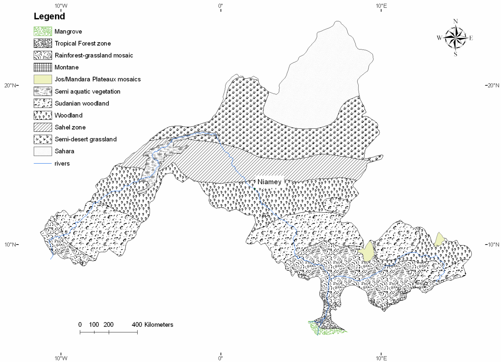
Figure I- 4 : Generalized vegetation map of the Niger River basin (after White, 1983)
