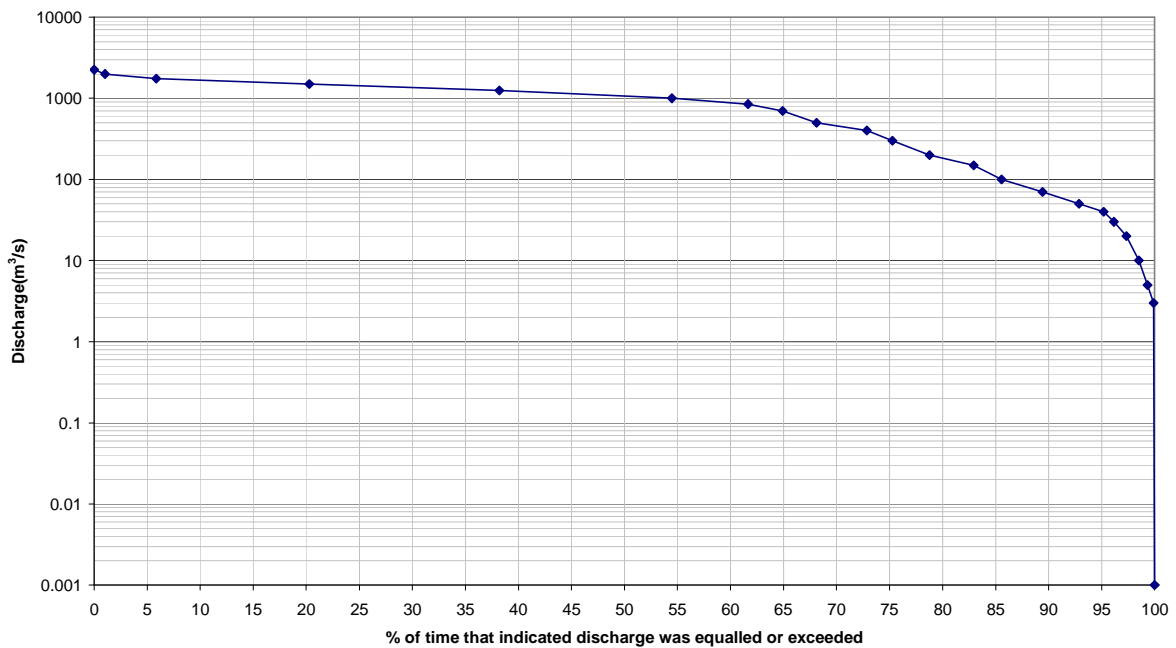
Figure D- 2:Flow duration curve, Niger at Niamey (Wet spell)
