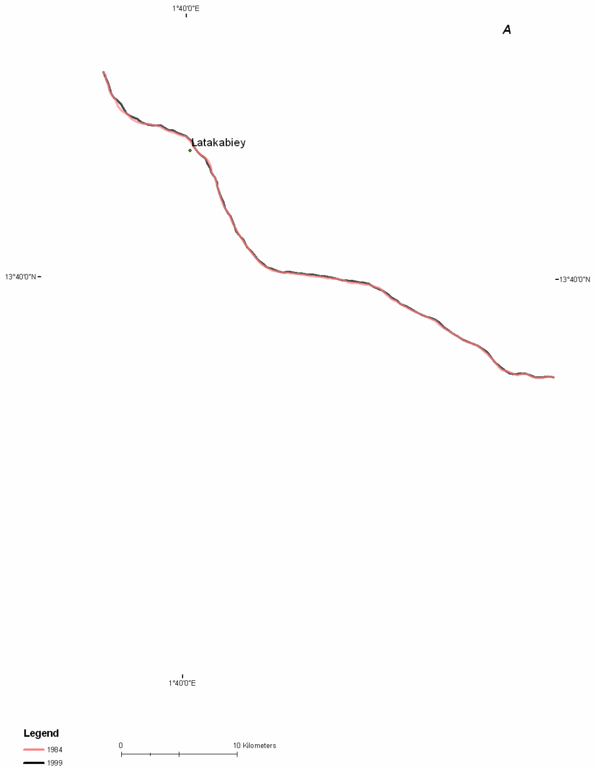
Figure B- 45A: River centre line change in reach 2 (1984 – 1999)
