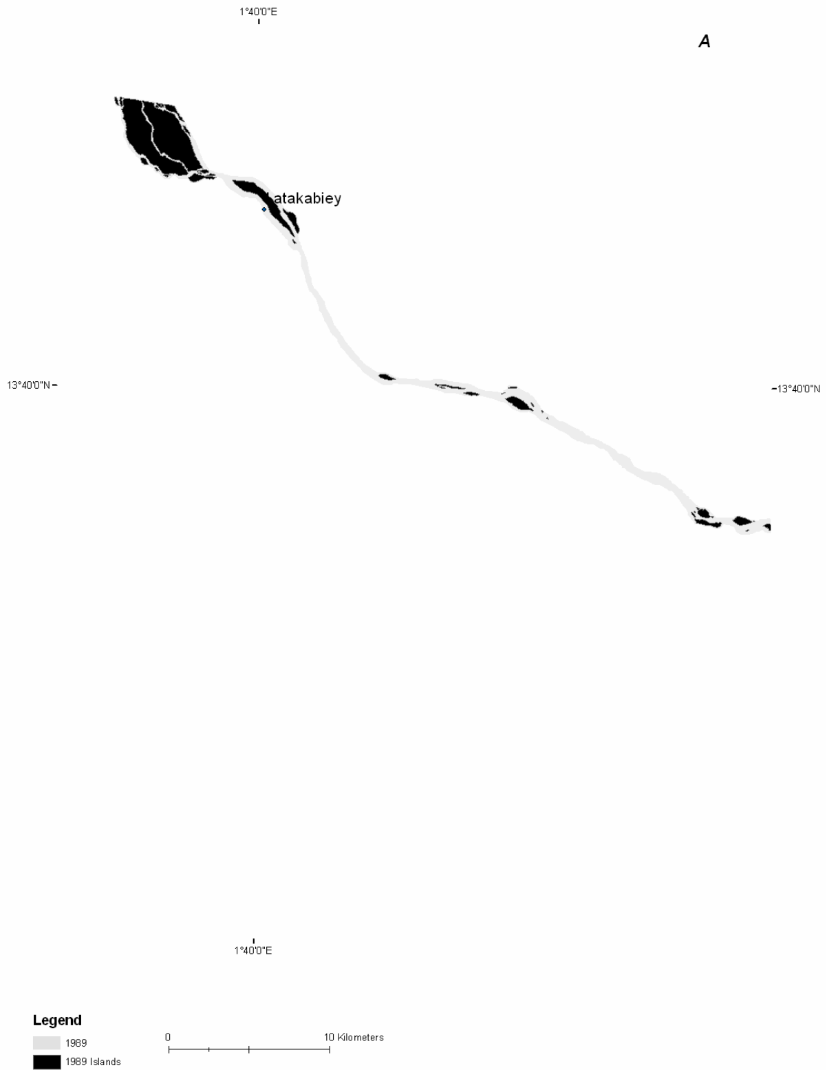
Figure B- 55A: Reach 2 channel bank and island extents in 1989
