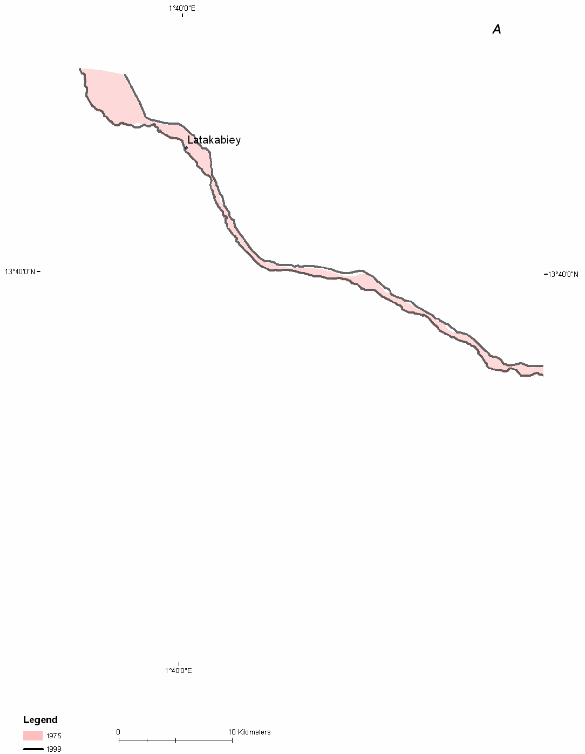
Figure B- 34A: Channel change in Reach 2 (1975-1999)
