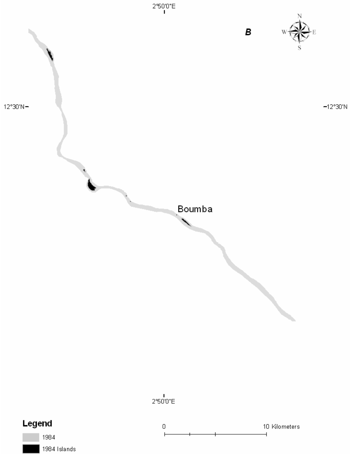
Figure B- 86B: Reach 3 channel bank and island extents in 1984
