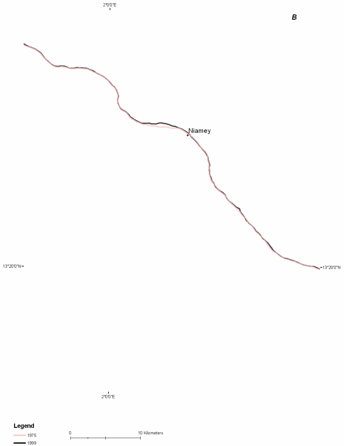
Figure B- 47B: River centre line change in reach 2 (1975 – 1999)
