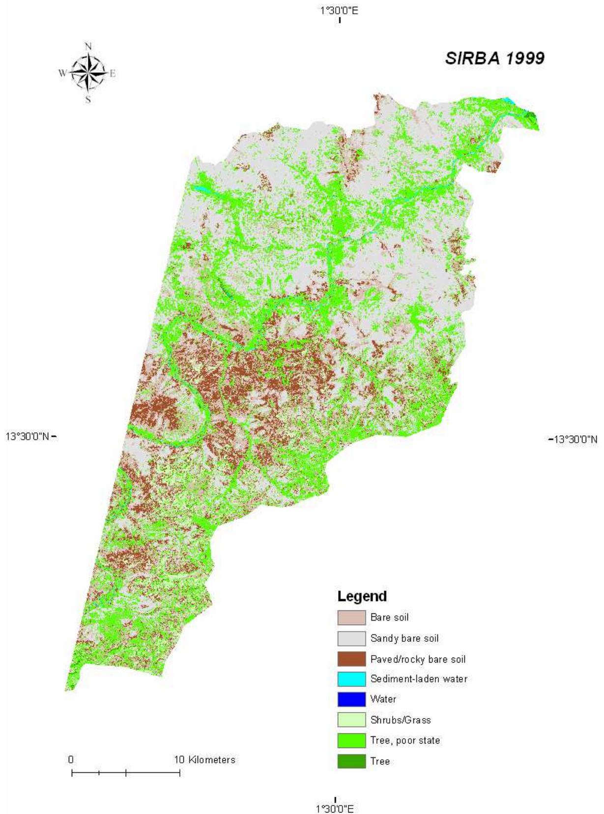
Figure III- 30: Sirba basin land cover.31/10/1999 (1105 km 2 )
