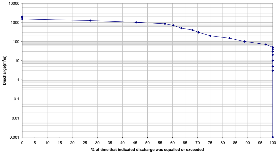
Figure D- 3: Flow duration curve, Niger at Niamey (Wettest year)
