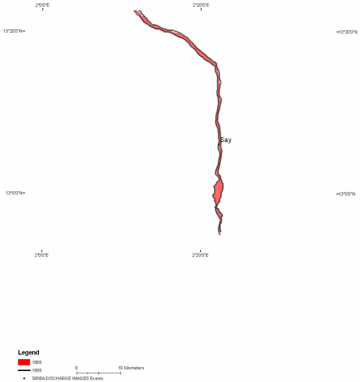
Figure B- 42C: Channel change in Reach 2 (1989-1999)
