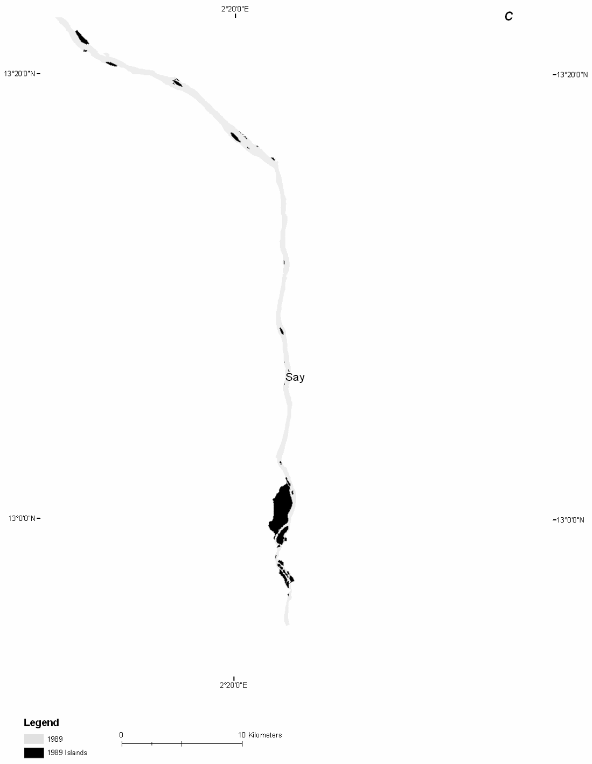
Figure B- 63C: Reach 2 channel bank and island extents in 1989
