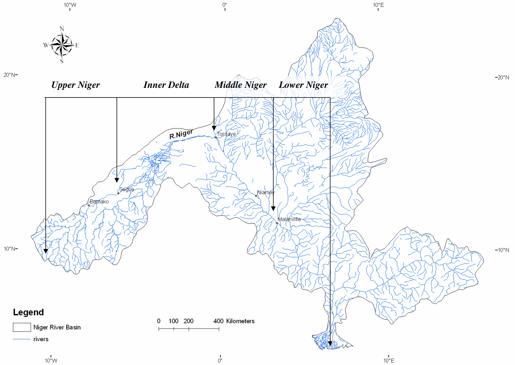
Figure I- 2 : The Niger River Basin
