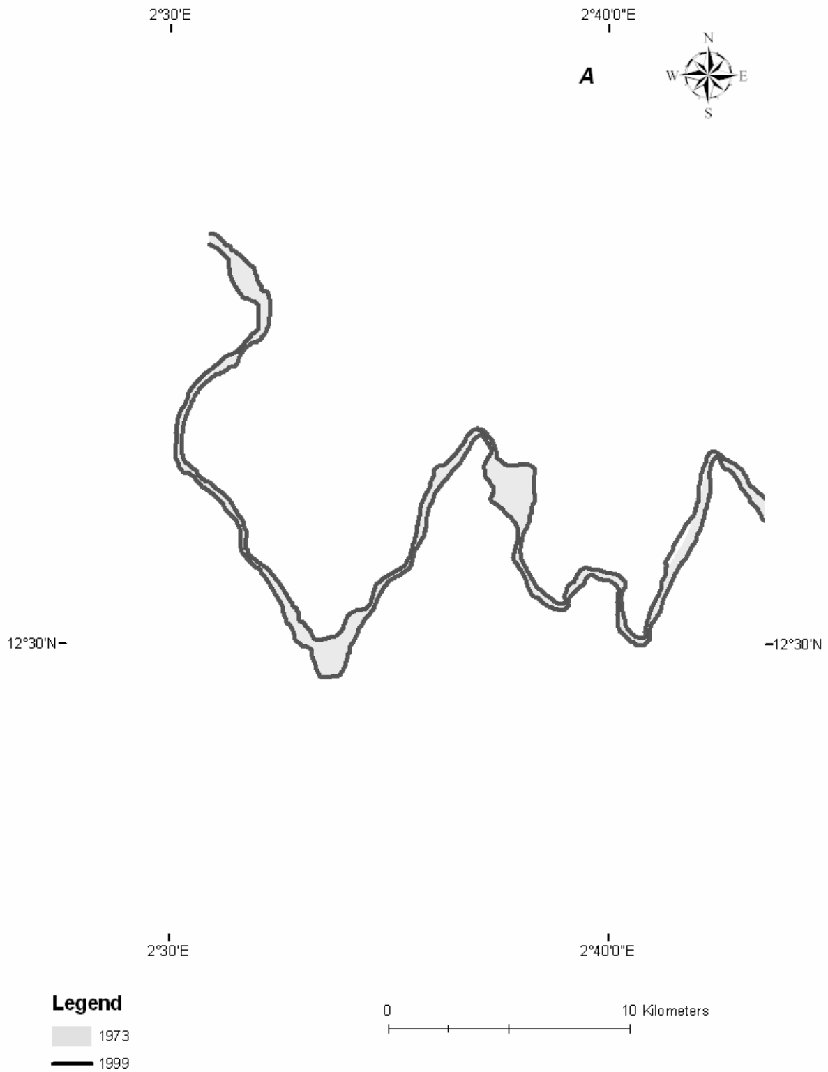
Figure B- 74A: Channel change in Reach 3 (1973-1999)
