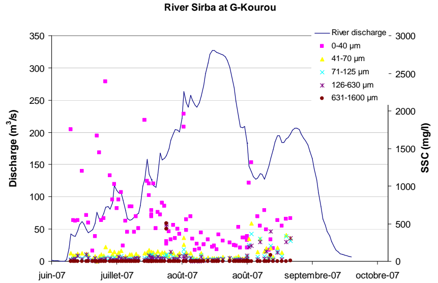
Figure V- 18: River discharge and SSC relationship for the River Sirba (according to size class) at Tiambi and G-Kourou (2006 and 2007)
