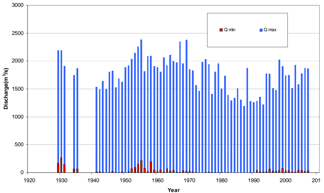
Figure IV- 11: Annual minimum ( Q_{\text{MIN}} ) and maximum ( Q_{\text{MAX}} ) daily mean discharge of the Niger River at Niamey (1929/30 – 2007/08)
