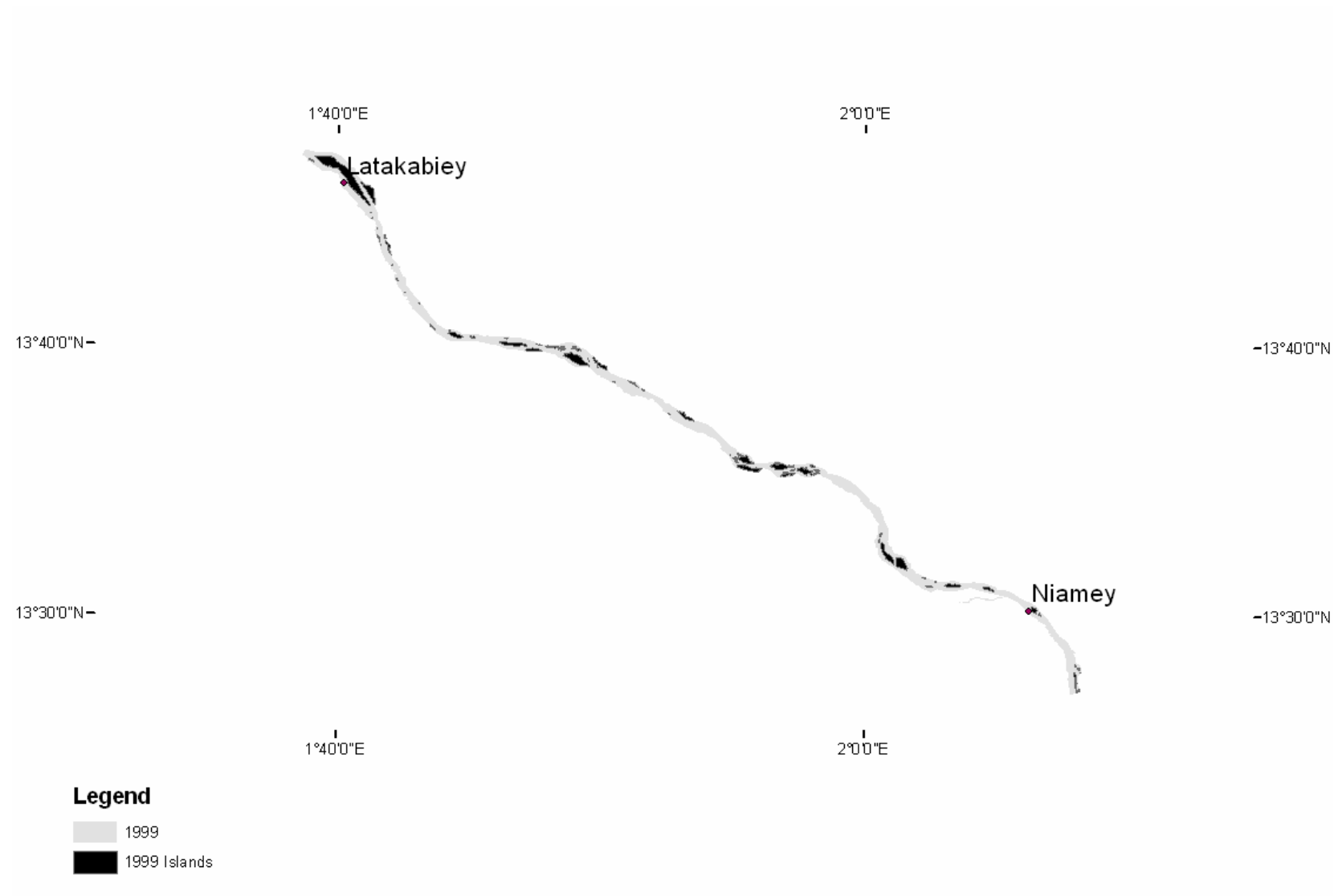
Figure B- 72: Reach 2 channel bank and island extents in 1999
