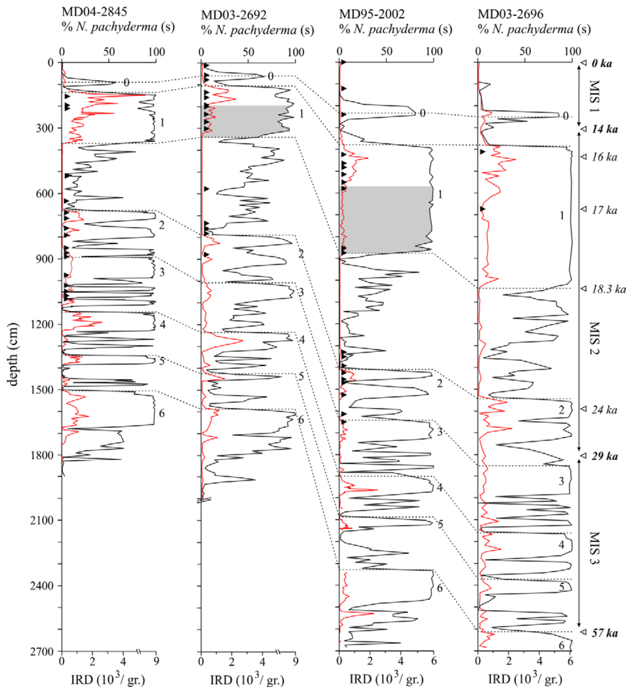
Figure 2. Abundance of planktic foraminifers N. pachyderma (s) (continuous black line - %) and of IRD (red line - 10^3/\text{gr.} ) from sediment cores MD04-2845, MD03-2692, MD95-2002 and MD03-2696. Dashed black lines and associated numbers represent core-to-core correlations using the upper limit of the Heinrich events (HE) 0 (i.e. Younger Dryas), HE 2, HE 3, HE 4, HE 5 and HE 6 and the lower and upper limits of the HE 1. AMS 14C dated samples are marked by black triangles on the depth scale. Bold ages and associated open triangles delimit the Marine Isotope Stages (MIS) boundaries according to the chronology of Lisiecki and Raymo (2005). Intermediate ages and associated open triangles within the MIS 2 make reference to the ages used in the Figure 6. Grey shading corresponds to the laminated facies deposited between ca. 18.3 and ca. 17 ka at site MD03-2692 and MD95-2002.
