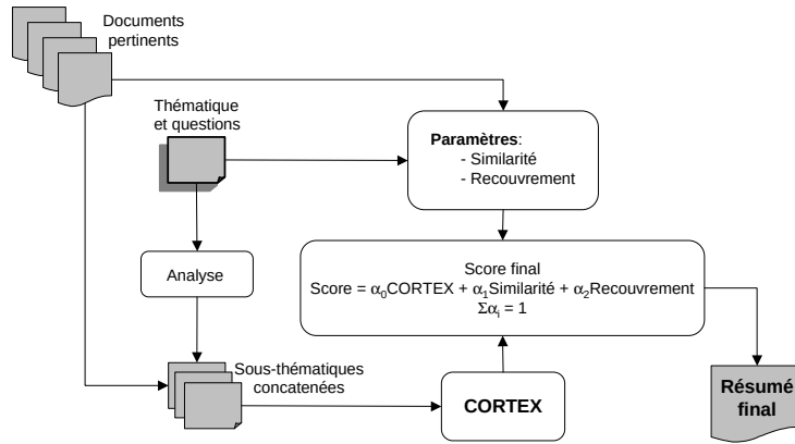
FIG. 6.1: Architecture de Neo-Cortex
