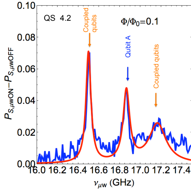
Fig. 3.11. Spectroscopic lines of sample QS 4.2 when the two quantroni- um are in resonance, i.e. at \Phi/\Phi_0 = 0.1 on Fig. 3.9. The central peak corresponds to the excitation of the transition |0\rangle \rightarrow |1\rangle of qubit A uncoupled to qubit B, whereas the two other peaks corresponds to the transition |\Psi_0\rangle \rightarrow |\Psi_1\rangle (left) and |\Psi_0\rangle \rightarrow |\Psi_2\rangle (right). The blue lines corresponds to the measured switching probability variations, whereas the red lines is a fit with three lorentzian lines of amplitude x , y , and z (from left to right).
