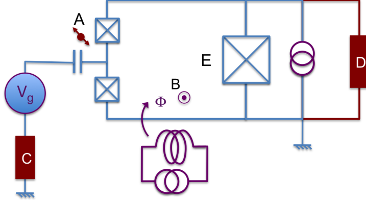
Fig. 1.8. Main decoherence sources in a qunatronics device. Noise in N_g is generated by charged two-level fluctuators (A) in the vicinity of the island and by voltage fluctuations of series impedance (C) in the gate line. Noise in \delta is generated by fluctuations in the flux \phi (B), by current fluctuations in the finite impedance (D) of the readout bias source. Noise in E_J is induced by critical current fluctuations of the CPB junctions (E).
