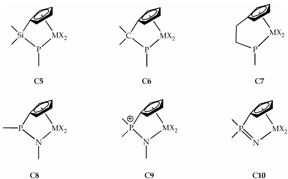
Figure 12 Phosphorus-containing constrained geometry complexes C5-10 (M = Ti, Zr, Hf).
