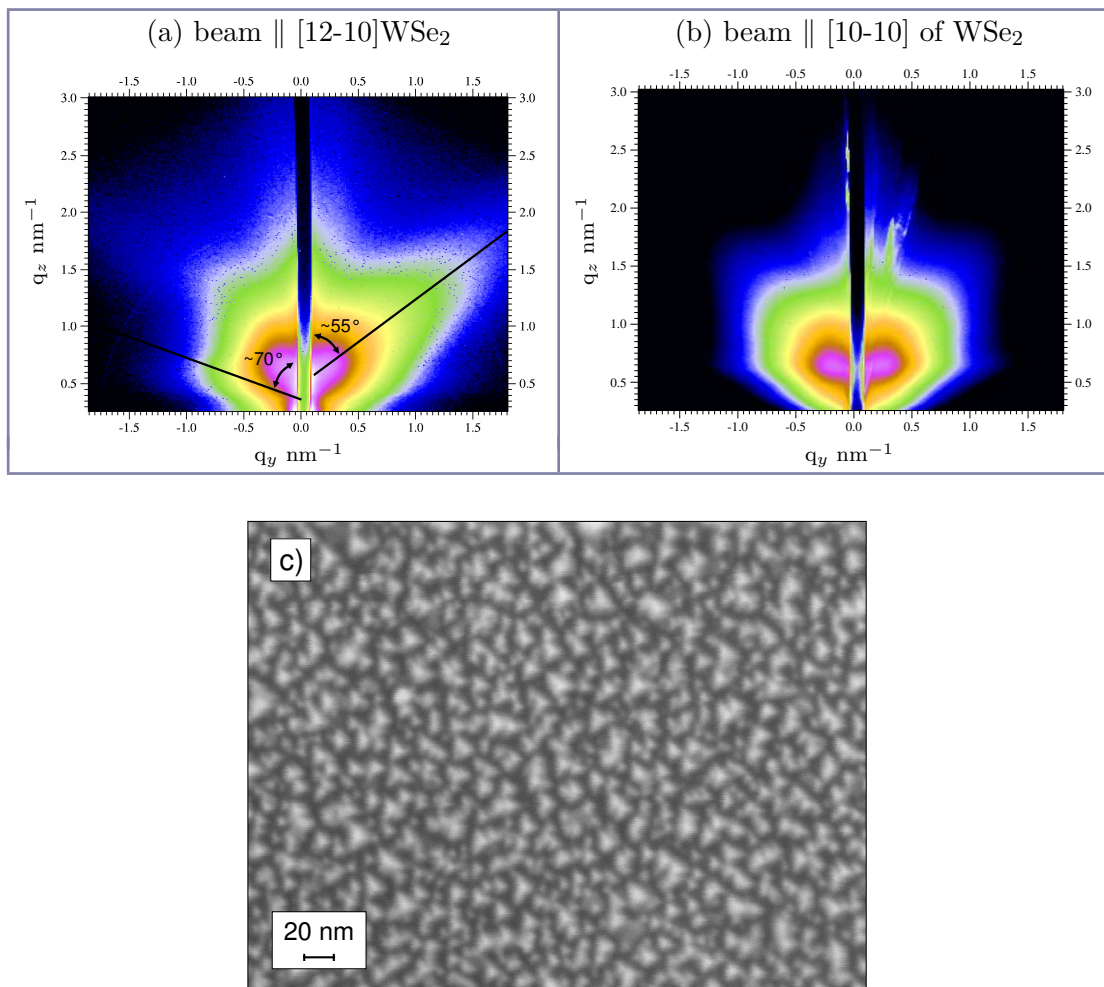
Figure 3.27: 2D GISAXS experimental intensity for a 3.0 nm thick CoPt 3 (111)/WSe 2 (0001) deposit at 700 K with the beam aligned along the [12-10] WSe 2 (0001) corresponding the [1-10] CoPt 3 (111) (a) and the beam aligned along the [10-10] WSe 2 (0001) corresponding the [11-2] CoPt 3 (111) (b).
