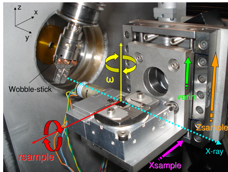
Figure 2.24: Interior of the sample chamber. The principal movement degrees are reported: the rotation of the sample holder around the normal to the surface, \omega and around the x-axis, r_{sample} ; the big, Z_{sample} , and small, verin , vertical translation; the horizontal translation, X_{sample} , along x-axis.
