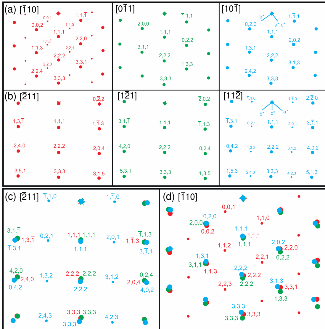
Figure 5.3: The intensity contribution of the diffraction pattern of each of the three variants along the chosen azimuths (a) [-110] and (b) [-210\ 1] directions. The definition of the directions is given with respect to the variant presented in figure 5.2(a). (c, d) The superimposition of the reflections coming from the three variants. The segments a^* , b^* , c^* correspond to the projections of the primitive vectors of the reciprocal lattice.
