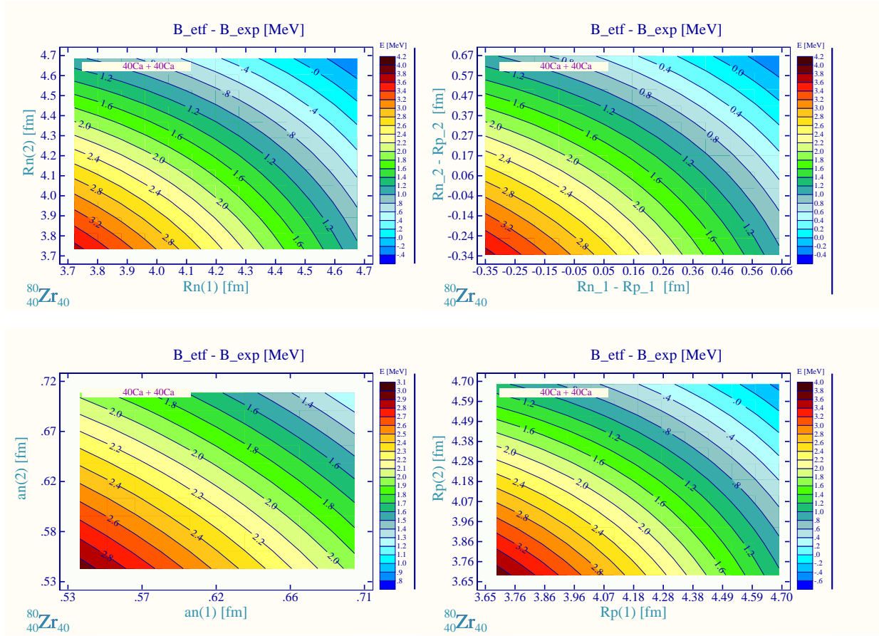
Figure 4.11: Same study as in Fig. 4.10 but for the very light system ^{40}\text{Ca} + ^{40}\text{Ca}
