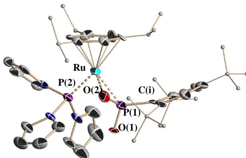
Figure 3 : Structure RX de \text{Ru}(\eta^6\text{-}1,3,5\text{-tri-}i\text{-propylbenzène})(\text{P}(\text{NC}_4\text{H}_4)_3)(\eta^2\text{-OPOMes}^*) ( 67c )
