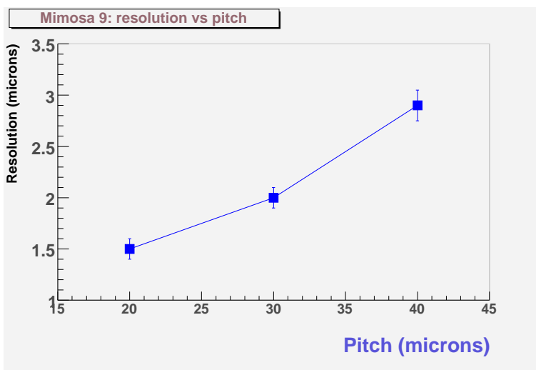
Figure 2.10.: The spatial resolution of MAPS (MIMOSA-9) as a function of the pixel pitch. From [26].
