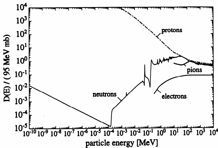
Figure 4.2.: The NIEL-Factors of different particles as a function of their energy. The factors are normalized with respect to a 1 MeV neutron. From [25].
