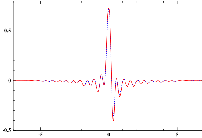
Figure 5.4: Density \rho_{Q^h} obtained with 28 MLWFs (line in red). The reference is a supercell calculation in a basis set of size 1224 (dashed line in blue).
