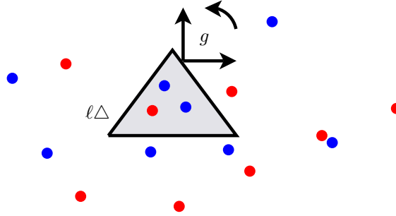
Figure 3.3: The Graf-Schenker inequality: the total Coulomb interaction of the charged particles is bounded below by an average over translations and rotations of a term corresponding to the Coulomb interaction of the particles which are in the simplex only, plus an error term.
