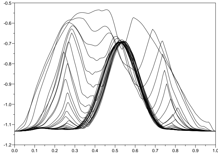
Figure 1.3: Energy along the successive deformed paths generated by the algorithm of [10] for the computation of the first singlet excited state of H_2 , with R = 1 \text{ \AA} .
