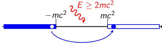
Figure 4.1: Creation of an electron-positron pair.
