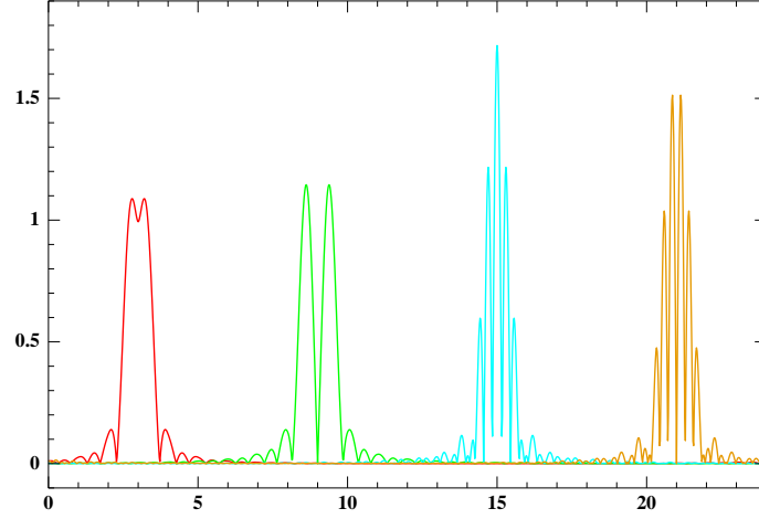
Figure 5.3: Modulus of MLWFs associated with the two occupied bands (left) and with the lowest two virtual bands (right).
