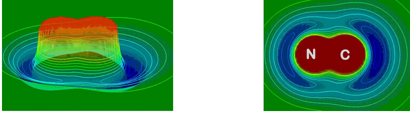
Figure 1.5: The Potential Energy Surface of HCN with C and N fixed (i.e. the value of the first Schrödinger eigenvalue when varying the position of H in the plane containing the three atoms), calculated in [81] using an MCSCF method.
