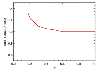
Fig. 12. Malmquist-Eddington bias. Ratio of simulated source counts to simulated observed source counts. Due to flux uncertainties, the number of counts is overestimated at low flux levels.
