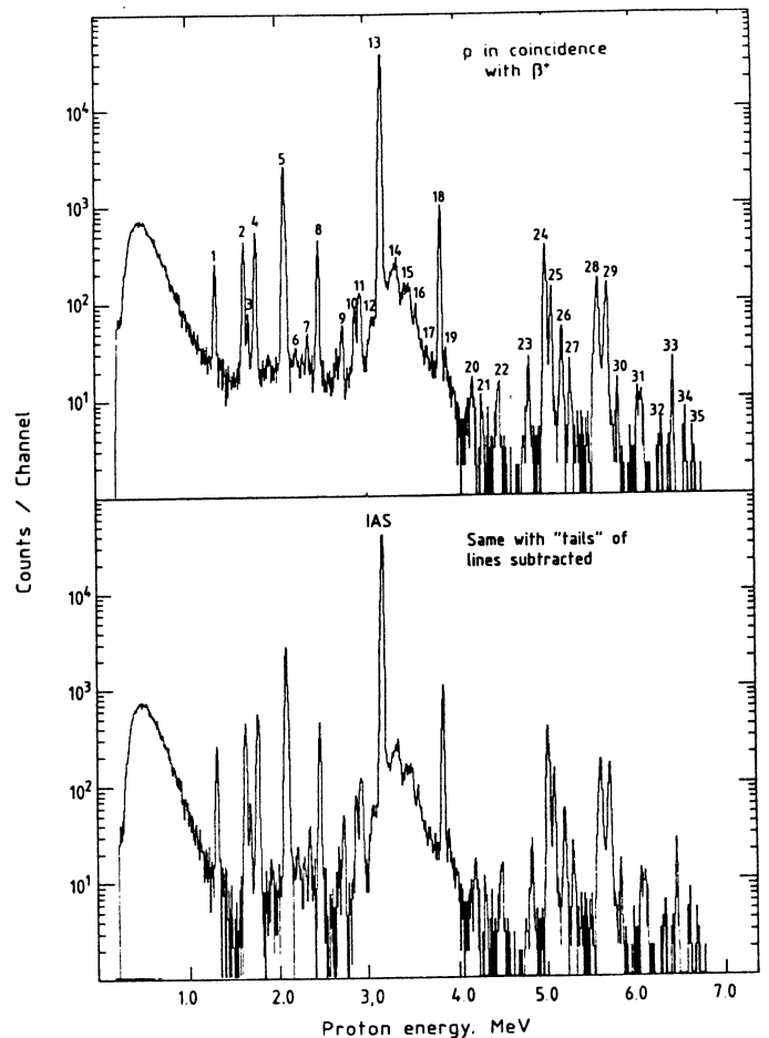
Fig. 2. Spectrum of \beta^+ delayed protons from ^{33}\text{Ar} measured with a 500 \mu\text{m} , 300 \text{mm}^2 Si surface barrier detector (FWHM 25 keV at 5 MeV) operated in coincidence with an annular Si detector placed upstream from the collection point. This coincidence requirement eliminates, in the recorded spectra, both the \beta^+ p summing and the background from long-lived \alpha -activities. The energies and intensities for the peaks marked with numbers are given in Table II. The lower part of the figure shows the same spectrum unfolded with the response function for protons of the Si detector (see text).
