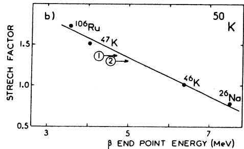
Fig. 3. Beta end-point calibration lines.
