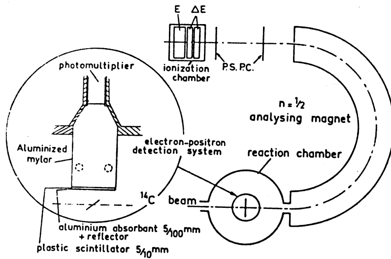
Fig. 1. — Experimental set-up.
