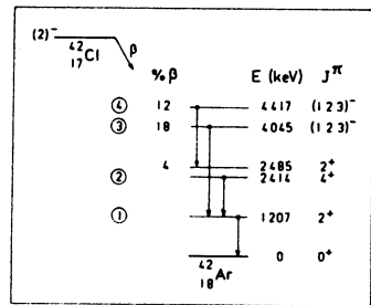
Fig. 2. Partial decay schemes of ^{40,42}\text{Cl} .
