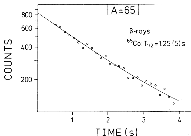
Fig. 7. The time spectrum of \beta -rays, measured with a 0.5 mm thick 4\pi plastic detector at A = 65 . The beam intensity was 12 particle \cdot nA, the cycle time 4 s. The main part of the \beta -spectrum belongs to the new isotope ^{65}\text{Co} . The half-life was calculated fitting a small background from long-lived activities. The figure shows the resulting decay curve and the measured count rates without subtraction of background.
