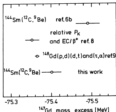
Fig. 3. Comparison of the experimental ^{147}\text{Gd} mass-excess values (cf. Table 1)
