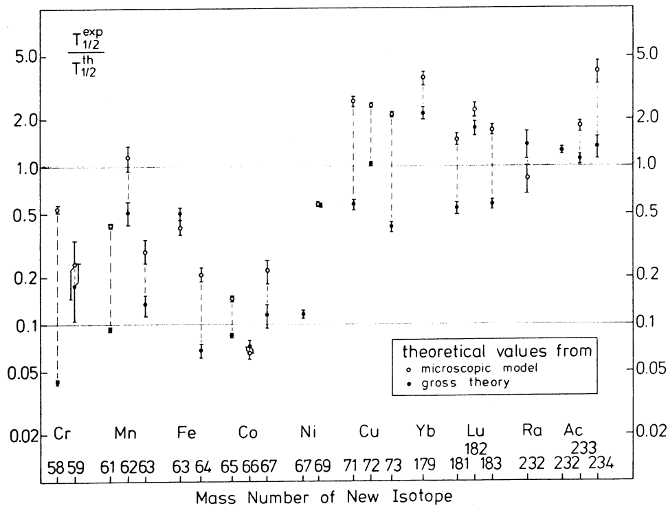
Fig. 1. Ratio of experimental and predicted \beta -decay half-lives, T_{1/2}^{\text{exp}}/T_{1/2}^{\text{th}} . The experimental values are from this work and refs. [1–5] and the theoretical ones from refs. [6,7]. The error bars represent only the experimental uncertainties.
