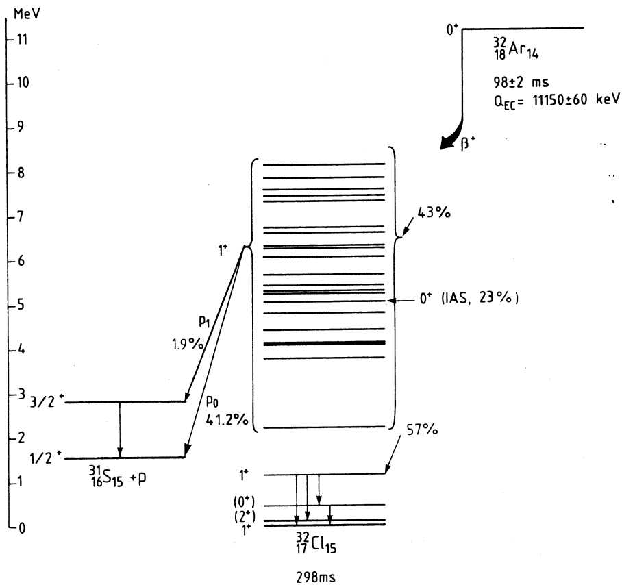
Fig. 8. Decay scheme of ^{32}\text{Ar} . The limit of detection in this work corresponds to 8.75 MeV excitation in ^{32}\text{Cl} .
