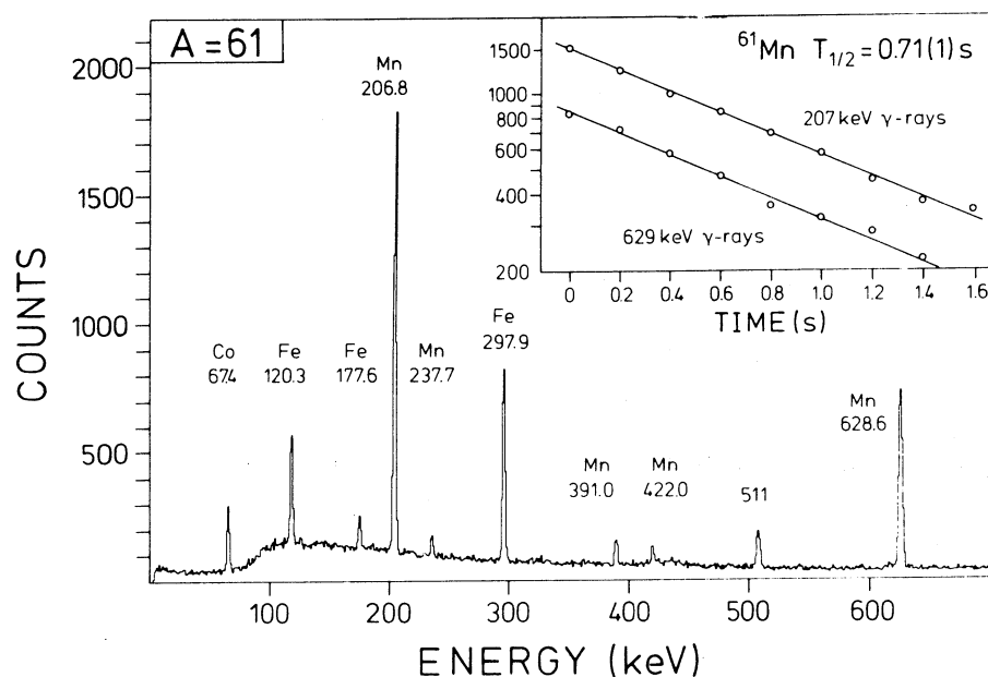
Fig. 1. Part of the \gamma -ray spectrum measured at A = 61 during 2 h with a 31% Ge(Li) detector in \beta -coincidence and a cycle of 4 s collection and counting time each. The beam intensity was 28 particle \cdot nA. The insert shows the decay curves of the most intense \gamma -rays assigned to ^{61}\text{Mn} .
