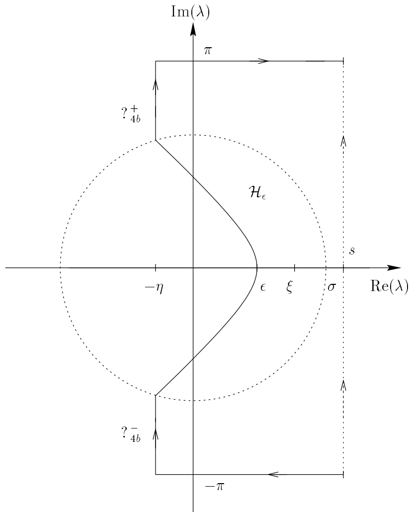
Fig. 2.11: Path of integration \Gamma_{4b}
