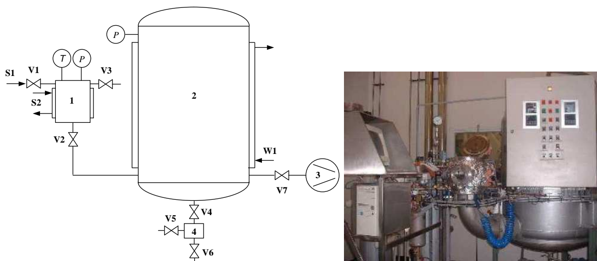
Figure 2.2. DIC set-up.
