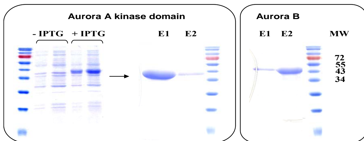
Figure 23. Purification of both the kinase domain of Aurora A and Aurora B kinase. SDS poly-acrylamide gel electrophoresis stained by Coomassie blue. On the left are shown bacterial lysates; Bacteria were either grown in the presence or the absence of IPTG. The samples eluted from the column are on the right (E1: the first elution. E2: the second elution). MW are in kDa.
