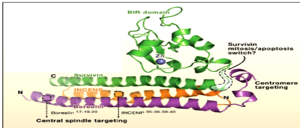
Figure 17. Survivin , INCENP and Borealin form a ternary complex. Survivin has a Zinc-binding globular domain (BIR domain) connected to the long C-terminal helix (C helix). Borealin and INCENP interact with the Survivin C helix to form a triple helical bundle. (Modified from Jeyaprakash et al. , 2007; Ruchaud et al. , 2007b).
