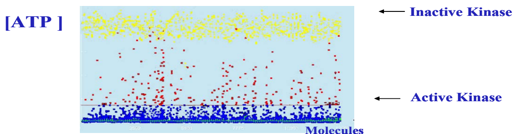
Figure 24: High throughput screening schema. The activity of Aurora kinase is determined based on the concentration of remaining ATP after the reaction between recombinant Aurora kinase and Histone H3. The highest concentration of ATP reflects the lowest Aurora kinase activity. Each point represents one tested molecule.
