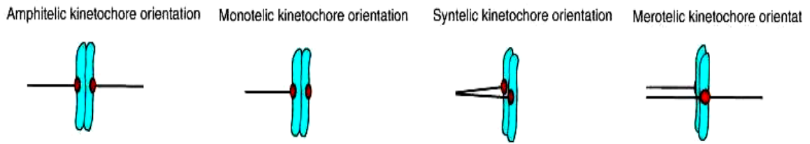
Figure II. 9: The model of kinetochore-microtubule attachments. Aurora B promotes the amphitelic kinetochore orientation. The mis-orientation, that consists in either monotelic or syntelic or merotelic kinetochore orientation, can lead to defects in chromosome segregation (Cimini and Degrossi, 2005).
