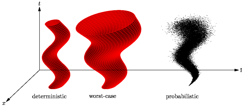
Figure 1.3: Uncertainty Representations.
