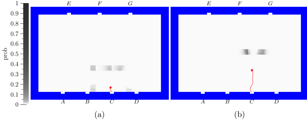
Figure 4.6: An object and its trajectory is observed (red): predictions for 10 timesteps ahead based on HMM graphs.
