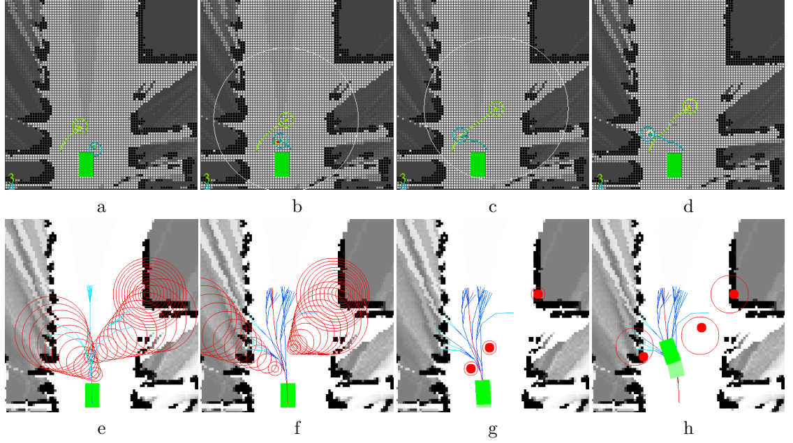
Figure 3.11: Partial planning in presence of two pedestrians: the Cycab is stopped and obstacles cross in front of it (a-d). At the beginning no movements are possible (e), but in next timesteps a safe trajectory is found (f). The trajectory is validated with observations from tracking (g-h).
