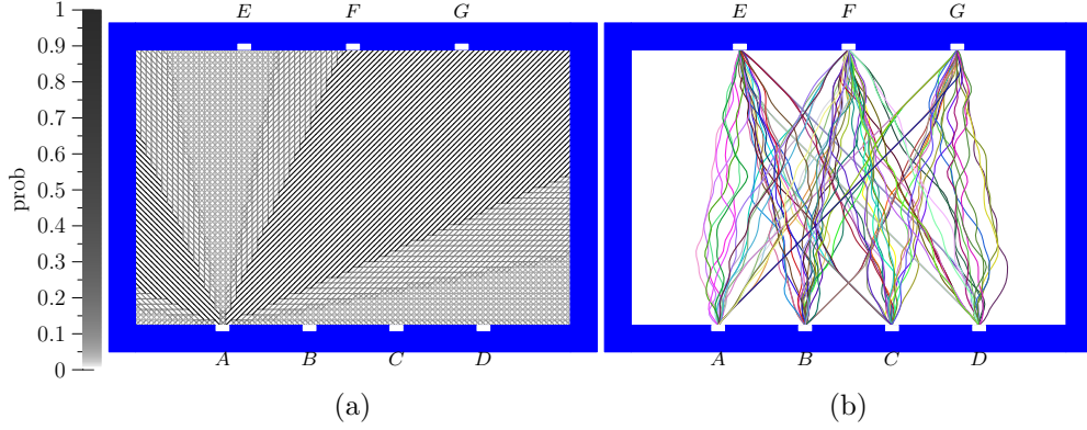
Figure 4.5: (a) Example of HMM graph toward goal A ; (b) Dataset of trajectories generated.
