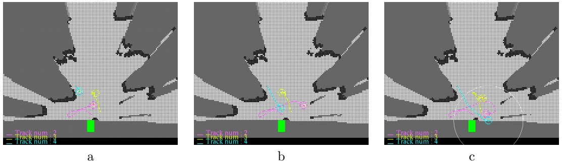
Figure 5.7: Mapping and target tracking example with three moving obstacles in front of the robot;(c) track number 4 disappears behind the robot.
