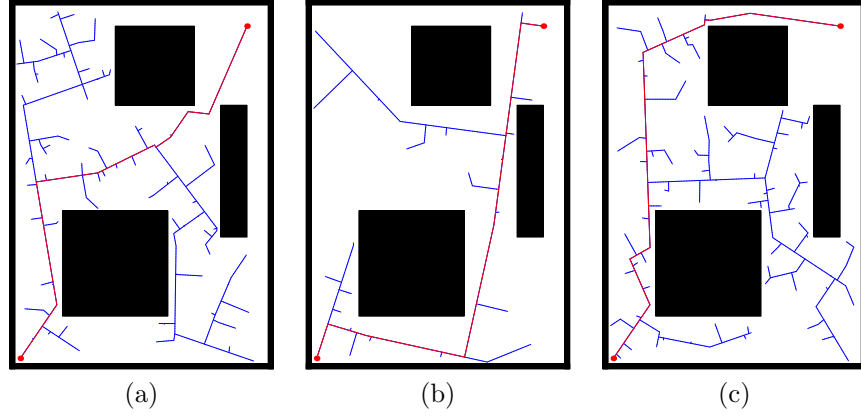
Figure 3.2: RRT basic algorithm applied to a point robot in a known static environment.
