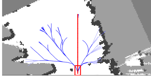
Figure 3.4: Probabilistic RRT algorithm applied to a non-holonomic robot in static environment. The search tree is shown in blue, lighter colour is for lower likelihood. The chosen path is shown in red. A discretized set of controls has been used to generate the tree.
